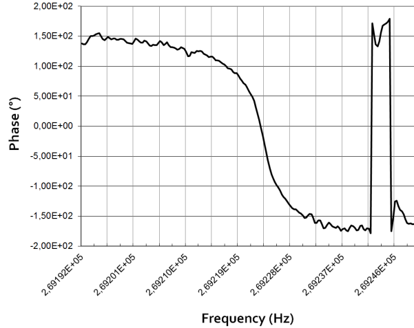
Fig. 2.17 – Phase frequency response of the MNT resonator, 2f measurement, 6V DC , 40mV AC and 200ms integration time. The frequency is the drive frequency, half the motion frequency.
