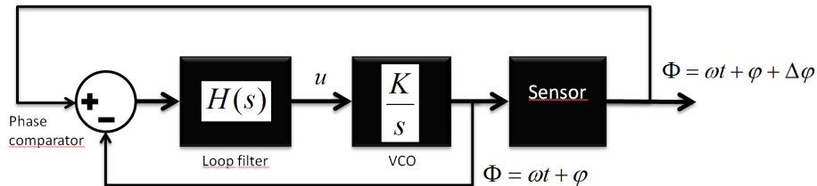
Fig. 2.19 – Principle schematic of a PLL applied to the frequency tracking of a resonant sensor. In this scheme, the feedback is performed only on the phase shift caused by the sensor, as sensor and VCO both operate at the same frequency.
