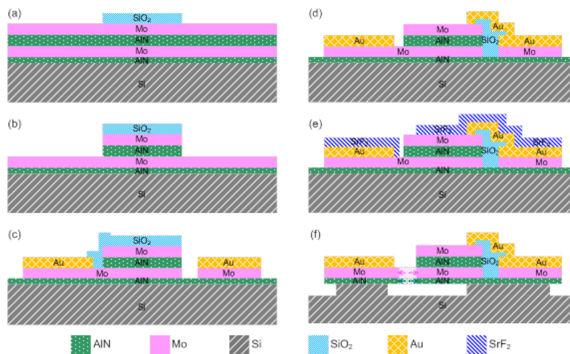
Fig. 3.20 – The multilayer stack comprises Mo/AlN/Mo/seed AlN (100nm/100nm/100nm/20nm) layers on Si. (a) Definition of SiO 2 mesa, followed by a Dry etch (b) to remove top Mo and AlN. (c) Au electrodes are patterned and deposited adjacent to the mesa region, along with an SiO 2 bridge protecting part of bottom Mo, while remaining bottom Mo removed. (d) SiO 2 is stripped and contact is made to the top Mo electrode (including deposition of a SiO 2 bridge layer. (e) NEMS devices are defined, using SrF 2 as a dry etch mask for both NEMS and all metallic contacts. (f) Anisotropic etching of all the structural layers down to Si by using Ar/Cl 2 ICP-RIE is followed by an isotropic Ar/NF 3 etch for device release, and subsequent removal of SrF 2 mask. The dashed arrows and lightly-hatched areas indicate that the bottom Mo and AlN layers are connected out of the present section plane (passing vertically through the longitudinal axis along a suspended cantilever).
