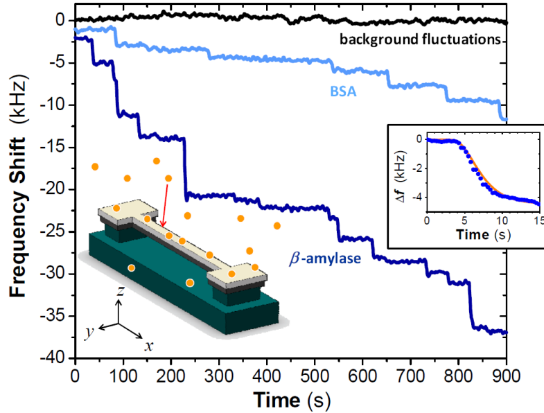
Fig. 5.4 – Real-time records of single-molecule adsorption events upon a NEMS mass sensor. This raw experimental data shows the distinctly-different, precipitous resonance frequency shifts of the NEMS during ESI-induced adsorption of bovine serum albumin (BSA, 66kDa) and \beta -amylase (200kDa). Each frequency jump downward is due to an individual protein adsorption event on the NEMS mass sensor. The height of the frequency jump is a convolved function of the mass of the protein adsorbed, and its position of adsorption upon the NEMS. Left Inset: Schematic illustrating single-molecule adsorption events on a NEMS resonator, and the coordinate system used to define its position-dependent mass responsivity ; from Naik et al. (2009).
