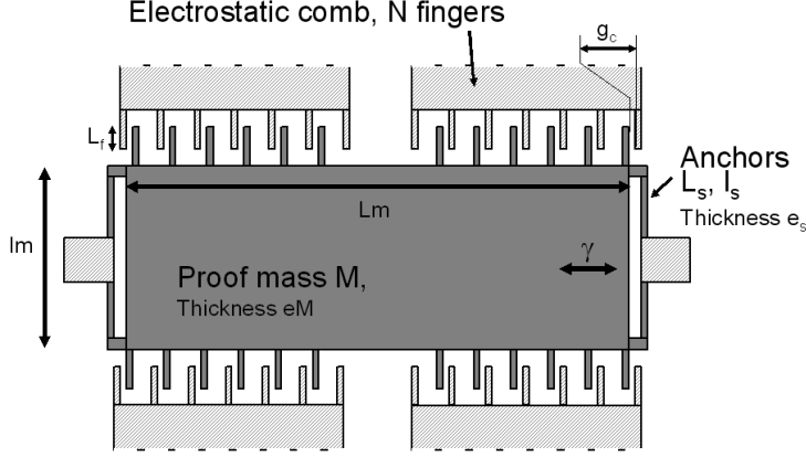
Fig. 2.22 – Studied structure
