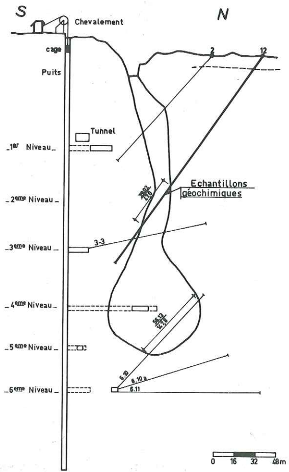
_ Section 200 E _
