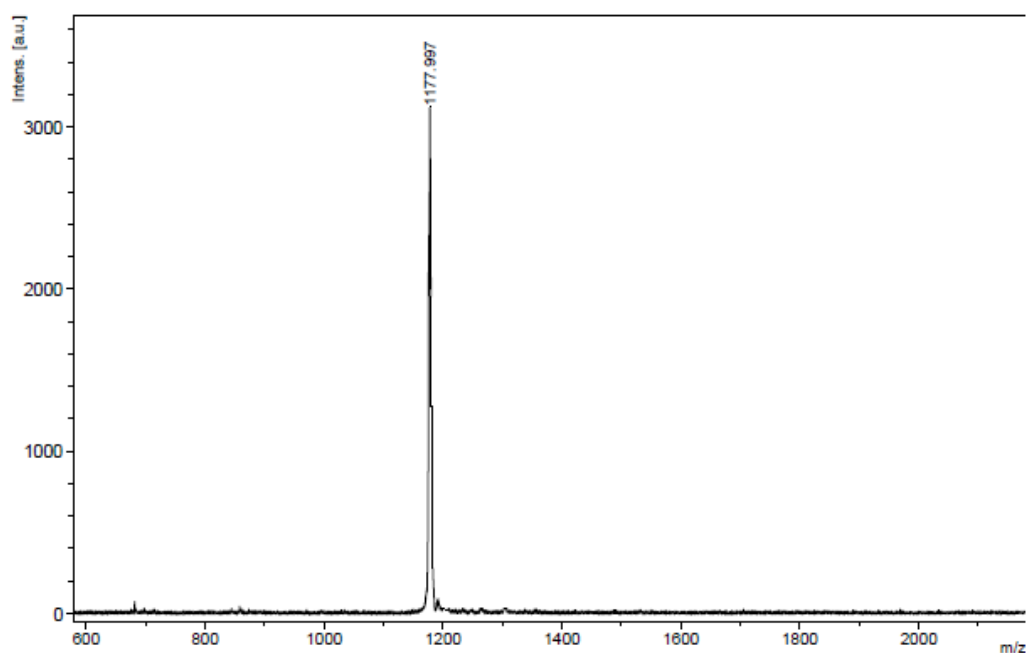
FigureANNEX4.16 Maldi-TOFspectrum of unsubstituted (A4) bis(phthalocyaninato) europium(III) complex ( \text{Eu}(\text{A}_4)_2 ) ( 16 ) [ \text{M}^+ : 1177]
