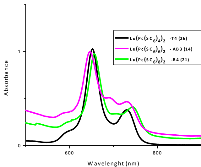
Figure 3.35. UV-NIR spectra of reduced \text{Lu(Pc)}_2\text{bis(phthalocyanine)} ( 1 \times 10^{-5} \text{ M} ) in \text{CHCl}_3
