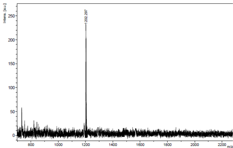
FigureANNEX4.18. Maldi-TOFspectrum of unsubstituted (A4) bis(phthalocyaninato) lutetium(III) complex ( \text{Lu}(\text{A}_4)_2 )( 18 ) [ \text{M}^+ : 1202]
