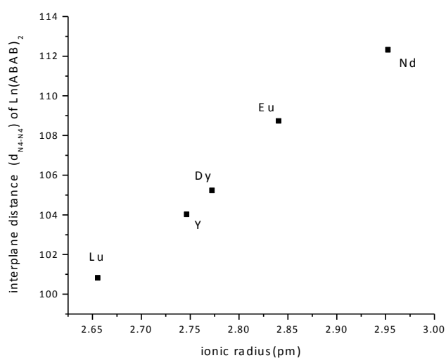
Fig. 3.17 The interplane distance ( d_{N4-N4} ) of Ln(ABAB) 2 vs lanthanide contraction
