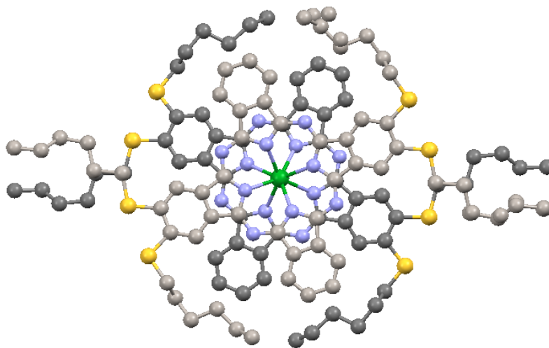
Figure 3.15 The molecular structure of \text{Lu}(\text{ABAB})_2 ( 9 )
