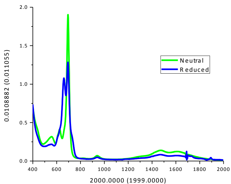
Figure ANNEX1.9. UV-NIR spectrum of AB3 bis(phthalocyaninato) yttrium(III) complex ( \text{Y}(\text{AB3})_2 )( 15 ) ( 1 \times 10^{-5} \text{ M} )
