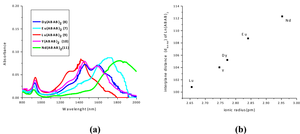
Figure 3.20(a) The UV-NIR spectrum of neutral Ln (Eu, Dy, Lu, Y, Nd)(ABAB) 2 in \text{CHCl}_3 ( 1 \times 10^{-5} M) (b) Plot of the interplane distances vs lanthanide ionic radius
