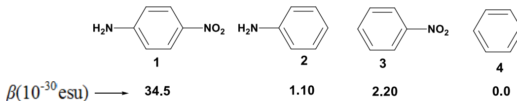
Figure 2.15. The second order optical nonlinearity in a donor or acceptor substituted benzene.
