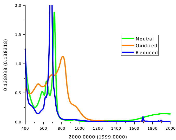
Figure ANNEX1.17. UV-NIR spectra of octahexylthia substituted (B4) bis(phthalocyaninato) neodymium(III) complex ( \text{Nd}(\text{B}_4)_2 )( 23 ) ( 1 \times 10^{-5} \text{ M} )
