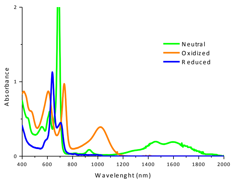
Figure ANNEX1.2. UV-NIR spectra of ABAB bis(phthalocyaninato) dysprosium(III) complex ( \text{Dy}(\text{ABAB})_2(\mathbf{8}) ) ( 1 \times 10^{-5} \text{ M} )
