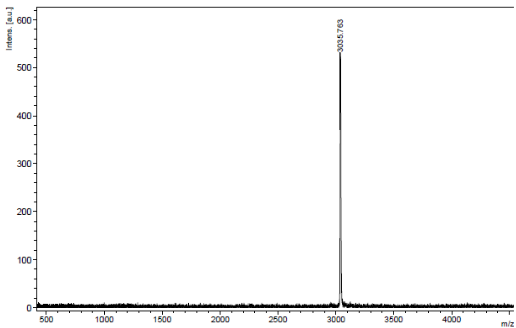
FigureANNEX4.19 Maldi-TOFspectrum of octahexylthia substituted (B4) bis(phthalocyaninato) europium(III) complex ( \text{Eu}(\text{B}_4)_2 ) ( 19 ) [ \text{M}^+ : 3035]
