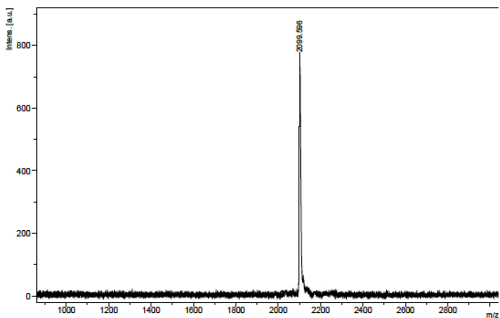
FigureANNEX4.11 Maldi-TOFspectrum of ABAB bis(phthalocyaninato) neodymium(III) complex ( \text{Nd}(\text{ABAB})_2(\mathbf{11}) ) [ \text{M}^+ : 2099]
