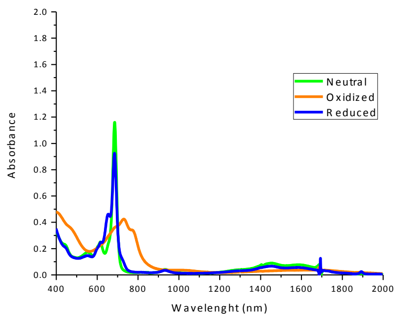
Figure ANNEX1.4. UV-NIR spectra of ABAB bis(phthalocyaninato) yttrium(III) complex ( \text{Y(ABAB)}_2 )( 10 ) ( 1 \times 10^{-5} \text{ M} )
