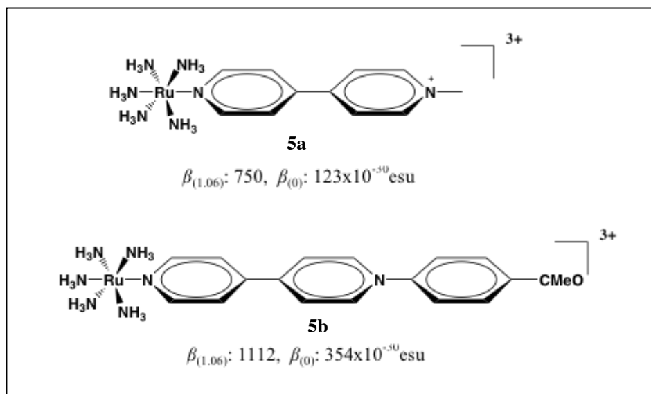
Fig. 2.19. Selected Ruthenium(II) amine complexes
