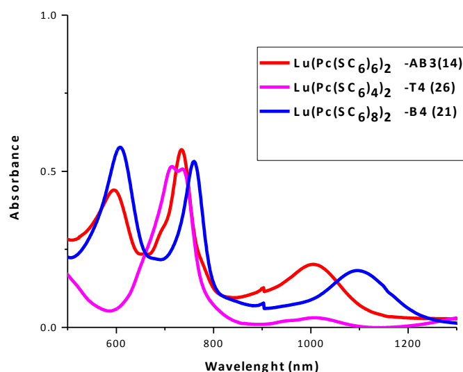
Figure 3.34. UV-NIR spectra of \text{Lu}(\text{Pc})_2 Bis(phthalocyanine) ( 1 \times 10^{-5} \text{ M} ) in \text{CHCl}_3 + \text{Br}_2 (oxidized)
