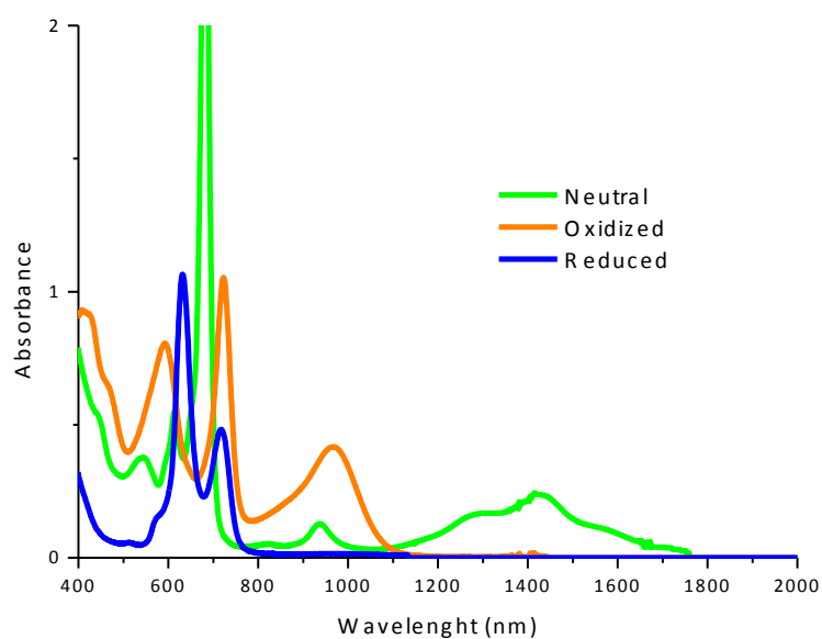
Figure ANNEX1.3. UV-NIR spectra of ABAB bis(phthalocyaninato) lutetium(III) complex ( \text{Lu}(\text{ABAB})_2(\mathbf{9}) ) ( 1 \times 10^{-5} \text{ M} )
