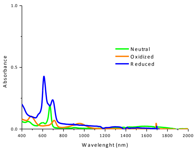
Figure ANNEX1.10. UV-NIR spectra of unsubstituted (A4) bis(phthalocyaninato) europium(III) complex ( \text{Eu}(\text{A}_4)_2 ) ( 16 ) ( 1 \times 10^{-5} \text{ M} )
