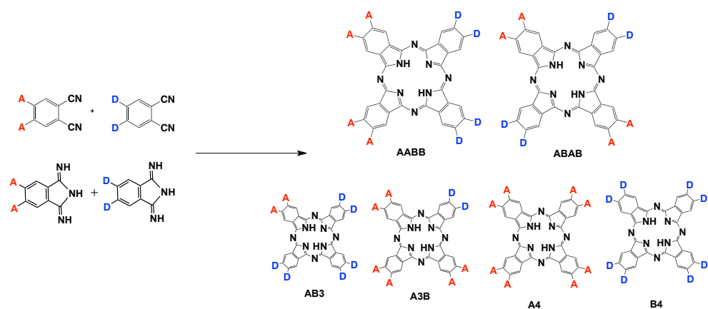
Figure3.2. The statistical condensation approach for the synthesise of ABAB type pc.
