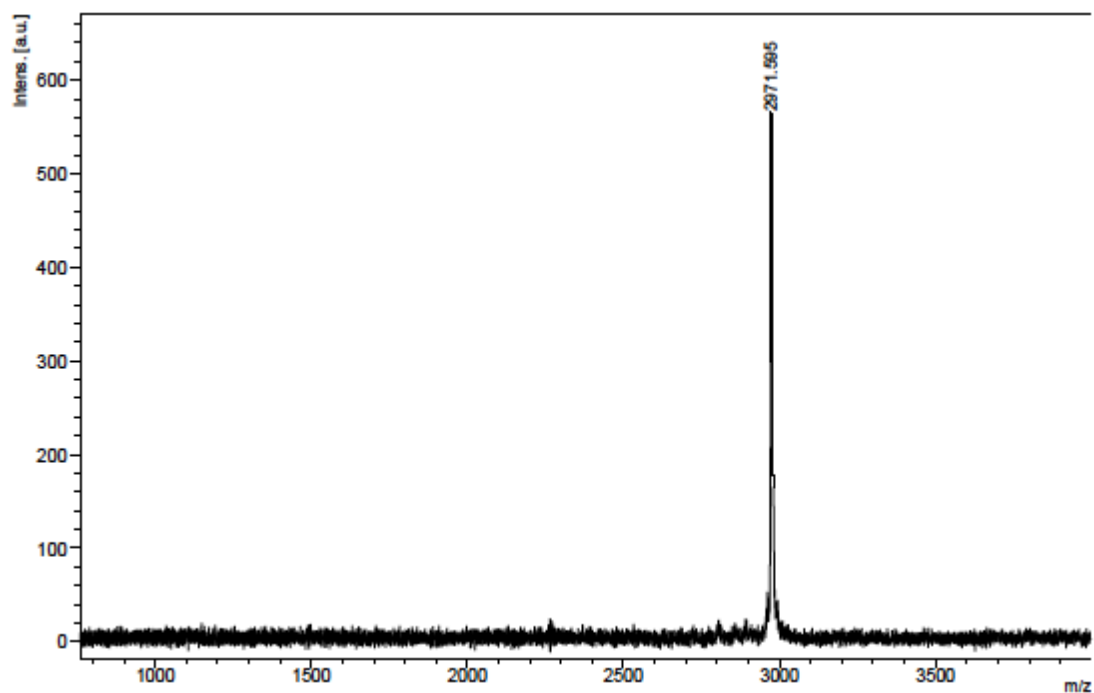
FigureANNEX4.20 Maldi-TOFspectrum of octahexylthia substituted (B4) bis(phthalocyaninato) yttrium(III) complex ( \text{Y}(\text{B}_4)_2 )( 22 ) [ \text{M}^+ : 2970]
