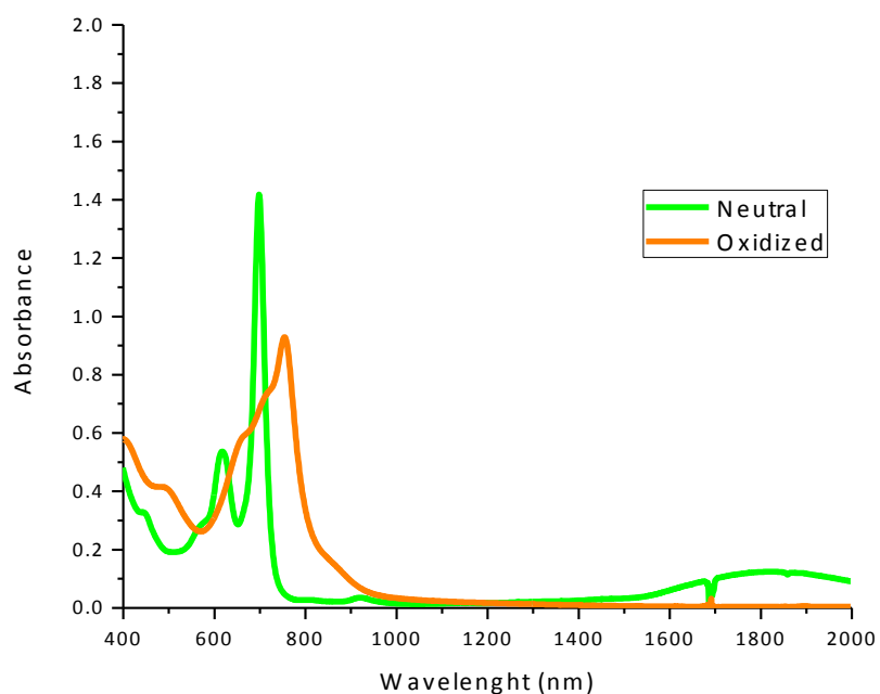
Figure ANNEX1.5. UV-NIR spectra of ABAB bis(phthalocyaninato) neodymium(III) complex ( \text{Nd(ABAB)}_2 )( 11 ) ( 1 \times 10^{-5} \text{ M} )
