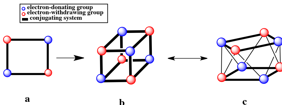
Figure 2.51. (a) Schematic representation of a molecule with square geometry (b) A cubic octupole template (c) A disordered cubic octupole template
