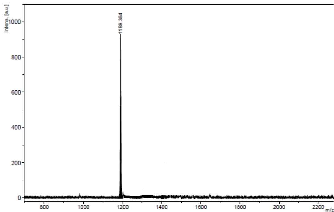
FigureANNEX4.17 Maldi-TOFspectrum of unsubstituted (A4) bis(phthalocyaninato) dysprosium(III) complex ( \text{Dy}(\text{A}_4)_2 ) ( 17 ) [ \text{M}^+ : 1189]
