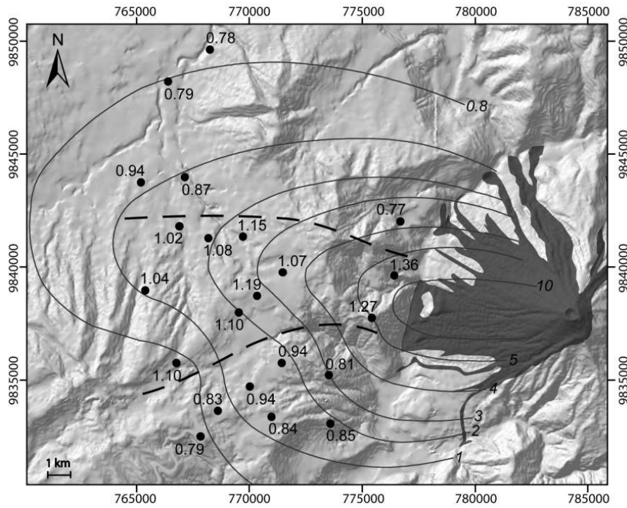
Figure 4.5 : Bulk density ( \text{g}/\text{cm}^3 ) measured at each sampling location with isopach contours in cm indicated (solid curves). Dashed line: boundary of the area where \rho_b > 1.0 \text{ g}/\text{cm}^3 .
