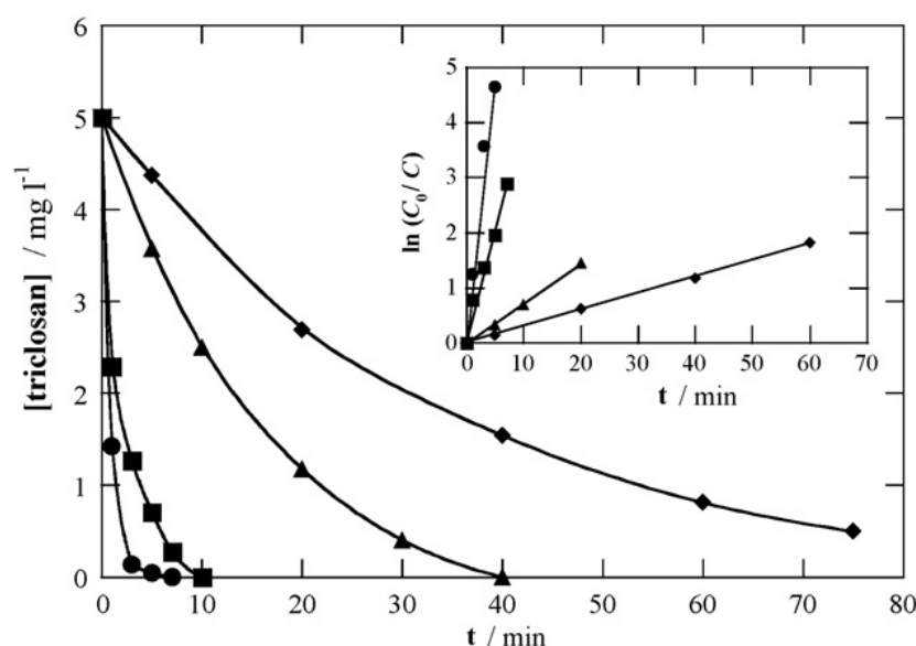
Figure 8. Triclosan degradation ( V_0 = 200 mL, C_0 = 5 mg triclosan/L, pH = 3 e I = 60 mA) in aqueous solution containing 0.05M of \text{Na}_2\text{SO}_4 and 0.20 mM of \text{Fe}^{3+} . Electrochemical cells: (●) Pt/FC, (■) BDD/FC, (▲) Pt/ \text{O}_2 and (◆) BDD/ \text{O}_2 (SIRÉS et al. , 2007b).
