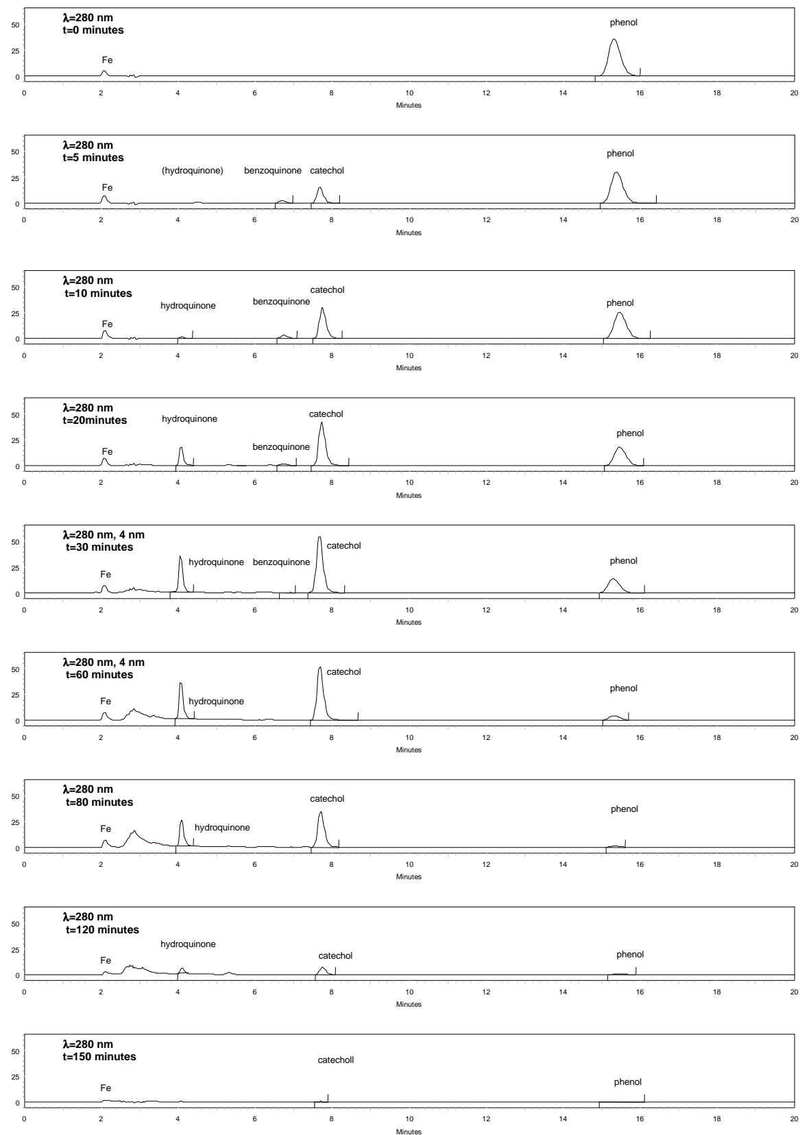
Annexe 1: Evolution of reverse-phase HPLC chromatograms (detection at 280 nm) during electro-Fenton treatment of 1.05 mM phenol aqueous solution. Experimental conditions: pH=3, I = 60 mA, V_0 = 125 mL, [Fe] = 0.1mM, Pt (1.5 cm x 2 cm) / CF (7 cm x 8 cm x 0,6 cm) electrodes. HPLC analysis conditions: Purospher RP-C18 column, eluent: water/methanol/acetic acid (79.2/19.8/1, v/v), flow rate: 0.8 mL/min.
