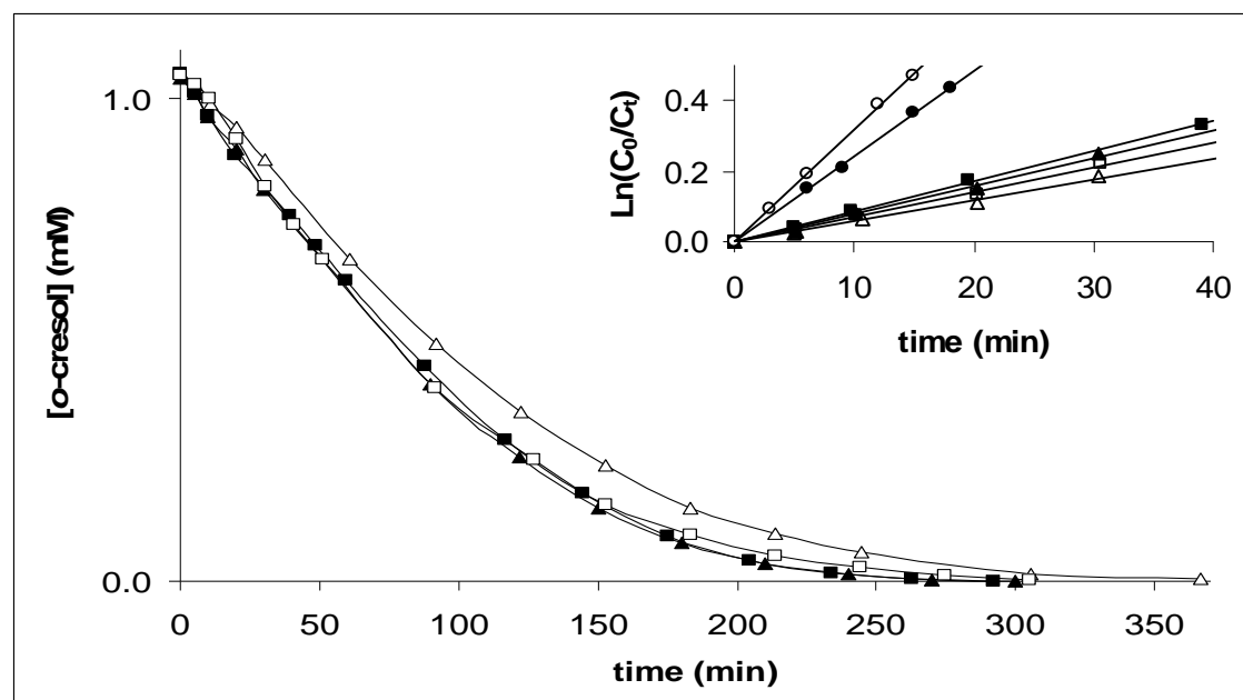
Figure 20. Effect of catalyst ( Fe^{2+} ) concentration on the degradation kinetics of o -cresol: (-□-) [Fe^{2+}] = 0.05 ( R^2=0.997 ), (-■-) [Fe^{2+}] = 0.10 ( R^2=0.999 ), (-▲-) [Fe^{2+}] = 0.25 ( R^2=0.997 ) and (-△-) [Fe^{2+}] = 1 mM ( R^2=0.996 ); m -cresol: (-○-) [Fe^{2+}] = 0.10 mM ( R^2=0.999 ) and p -cresol: (-●-) [Fe^{2+}] = 0.10 mM ( R^2=0.998 ) at pH 3 during current controlled electrolysis at 60 mA by electro-Fenton process. Experimental conditions: V_0=125 mL and Pt (1.5 cm x 2 cm) / CF (7 cm x 8 cm x 0,6 cm) electrodes.
