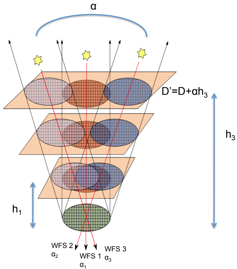
Figure 5.17: Principle of an AO wide field of view system of a diameter D , using 3 turbulent layers and n_{GS} = 3
