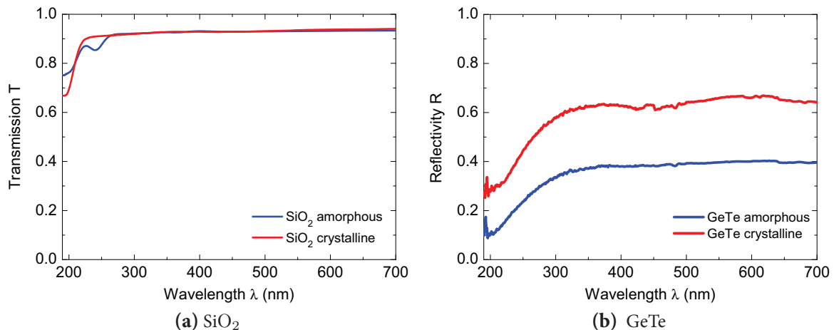
Figure 2.5: In contrast to non phase-change materials phase-change materials such as GeTe show a pronounced contrast in optical properties between an amorphous and a crystalline phase in the visible range. Image source: [Mer11]
