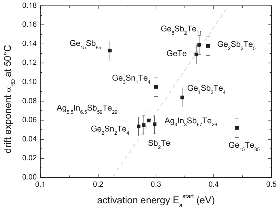
Figure 6.19: Comparison of drift exponents describing the increase in resistivity measured during heating amorphous phase-change materials and chalcogenides at 50^\circ\text{C} . In most of the studied materials the resistance drift is linked to the activation energy of electrical conduction E_a^{\text{start}} measured at the start of the drift, where a- \text{Ge}_{15}\text{Te}_{85} and a- \text{Ge}_{15}\text{Sb}_{85} form exceptions.
