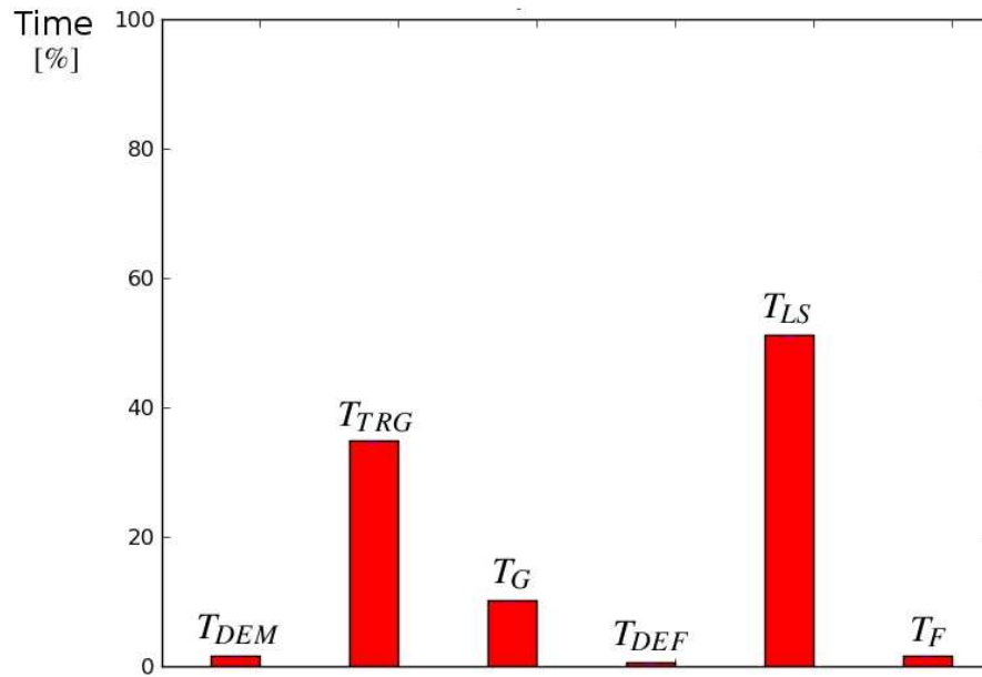
Figure 5.2: Cost proportion of each operation of eq.(5.1). The resolution of flow problem takes the 90% of the total time.
