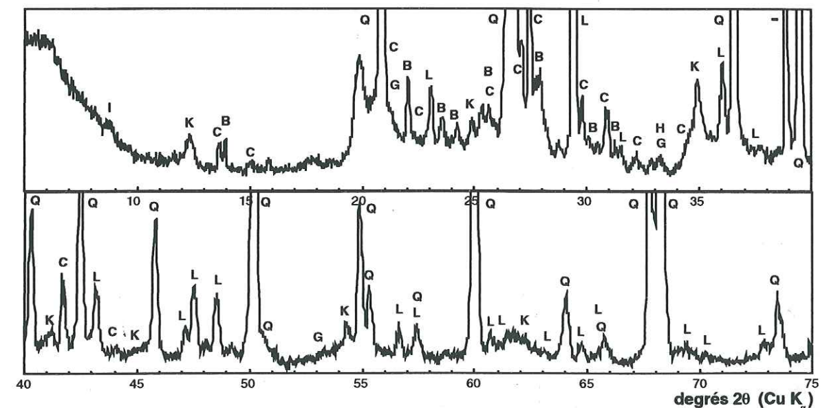
Figure 6-2 : Diffractogramme X de S 3 <1mm. I=illite, K=kaolinite, C=microcline, B=albite, Q=quartz, G=goéthite, H=hématite, L=calcite, - = organique.
