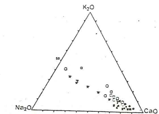
Figure 6. Na 2 O-K 2 O-CaO diagram of Possession Island lavas. Same symbols as Figure 4.
