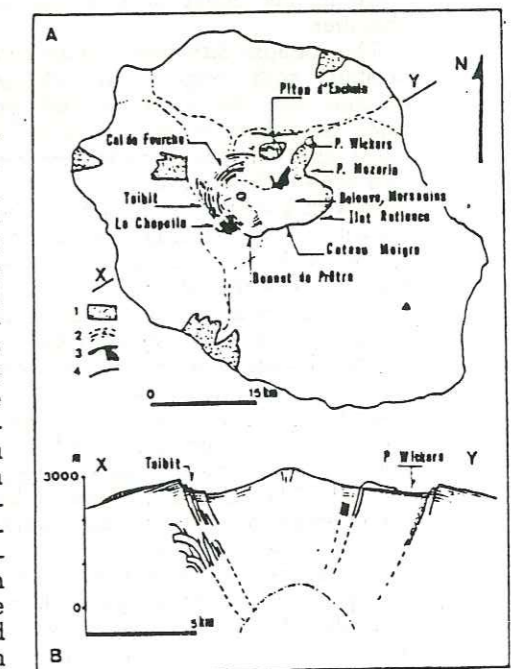
FIG. 7 — Caldera stage of the alkaline differentiated period.
