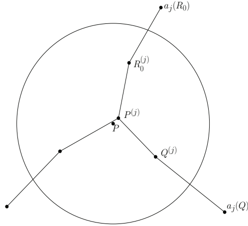
FIGURE 6.6.1 – Cas A
