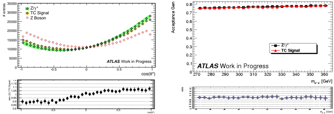
Figure F.1: On the left plot \cos(\theta^*) distribution at generator level for the Z bosons, the Z/\gamma^* , and TC signal process, the colored bands define the variation of the \cos(\theta^*) distribution for different m_{ee} values. On the right plot at generator level the total acceptance as a function of the m(e^+e^-) for the Drell-Yan process and for a TC signal at 300 GeV. Note that Z/\gamma^* process is generated in the same mass range as the TC signal as described in section 5.1.2.
