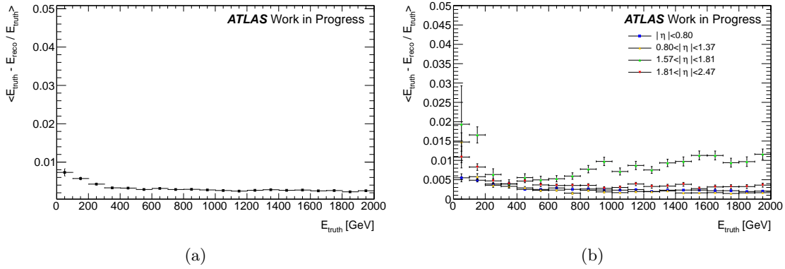
Figure E.1: Energy bias as a function of E_{truth} . (a) energy bias over full \eta range; (b) energy bias in \eta bins. The points in the plots correspond to the mean value of the \frac{\sigma_e}{E_{truth}} distribution obtained with a gaussian fit.
