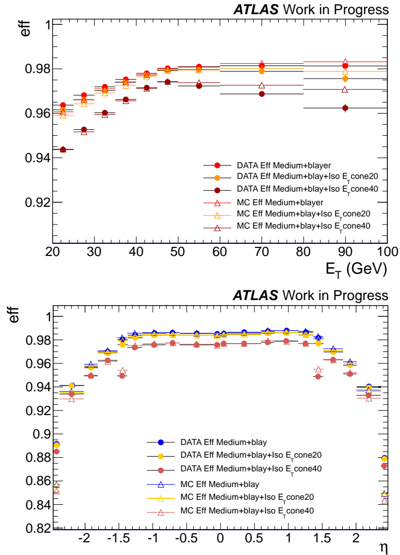
Figure 4.7: Data and MC electron identification efficiencies of the B-layer hit requirement, of the B-layer hit plus E_T cone20 isolation requirement, and of the B-layer hit plus E_T cone40 isolation requirement. Those efficiencies are measured as a function of (top) the electron E_T and (bottom) as a function of \eta for electron with E_T > 25 GeV. The errors evaluated in the plots take into account only the statistical uncertainties.
