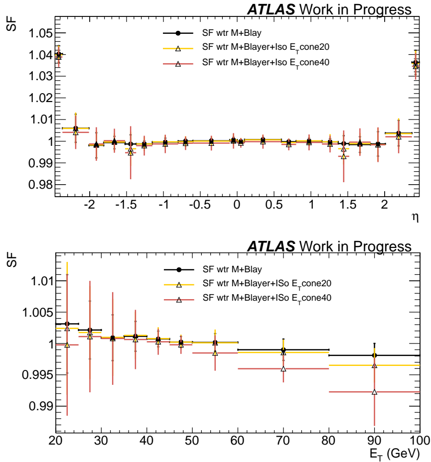
Figure 4.9: SF for the identification efficiencies for medium plus B-layer electrons and medium plus B-layer and E_{T\text{cone}20} and E_{T\text{cone}40} isolation requirement as a function of the electron \eta (top) and as a function of E_T (bottom) bins. The errors evaluated in the plots take into account the statistical and systematic uncertainties.
