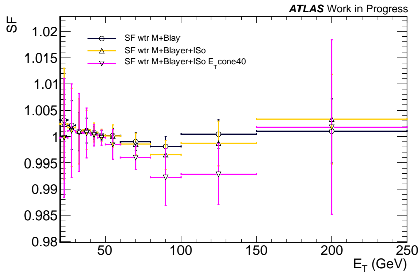
Figure D.4: SF for the identification efficiencies for medium plus B-layer electrons and medium plus B-layer and E_T cone20 and E_T cone40 isolation requirement as a function of the electron E_T bins. The errors evaluated in the plots take into account the statistical and systematic uncertainties.
