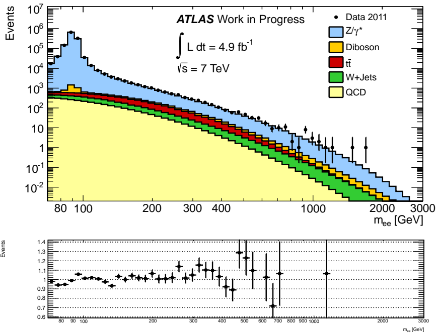
Figure 5.11: Dielectron invariant mass ( m_{ee} ) distribution after event selection for the 2011 data and the SM backgrounds overlaid.
