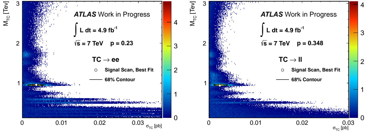
Figure 5.18: The absolute value of the profile LLR test as a function of \sigma_{TC} and M_{TC} for the likelihood fit (left) to ATLAS data in the dielectron channel; (right) to ATLAS data for the combination of the dielectron and dimuon channel.
