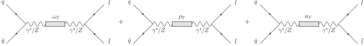
Figure 1.6: Feynman Diagram of the LSTC process giving fermion pairs l\bar{l} as a final state.
