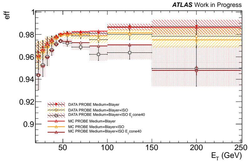
Figure D.3: Data and MC electron identification efficiencies of the B-layer hit requirement, of the B-layer hit plus E_T cone20 isolation requirement, and of the B-layer hit plus E_T cone40 isolation requirement. For the data points the errors evaluated in the plot take into account both the statistical and the systematic uncertainties.
