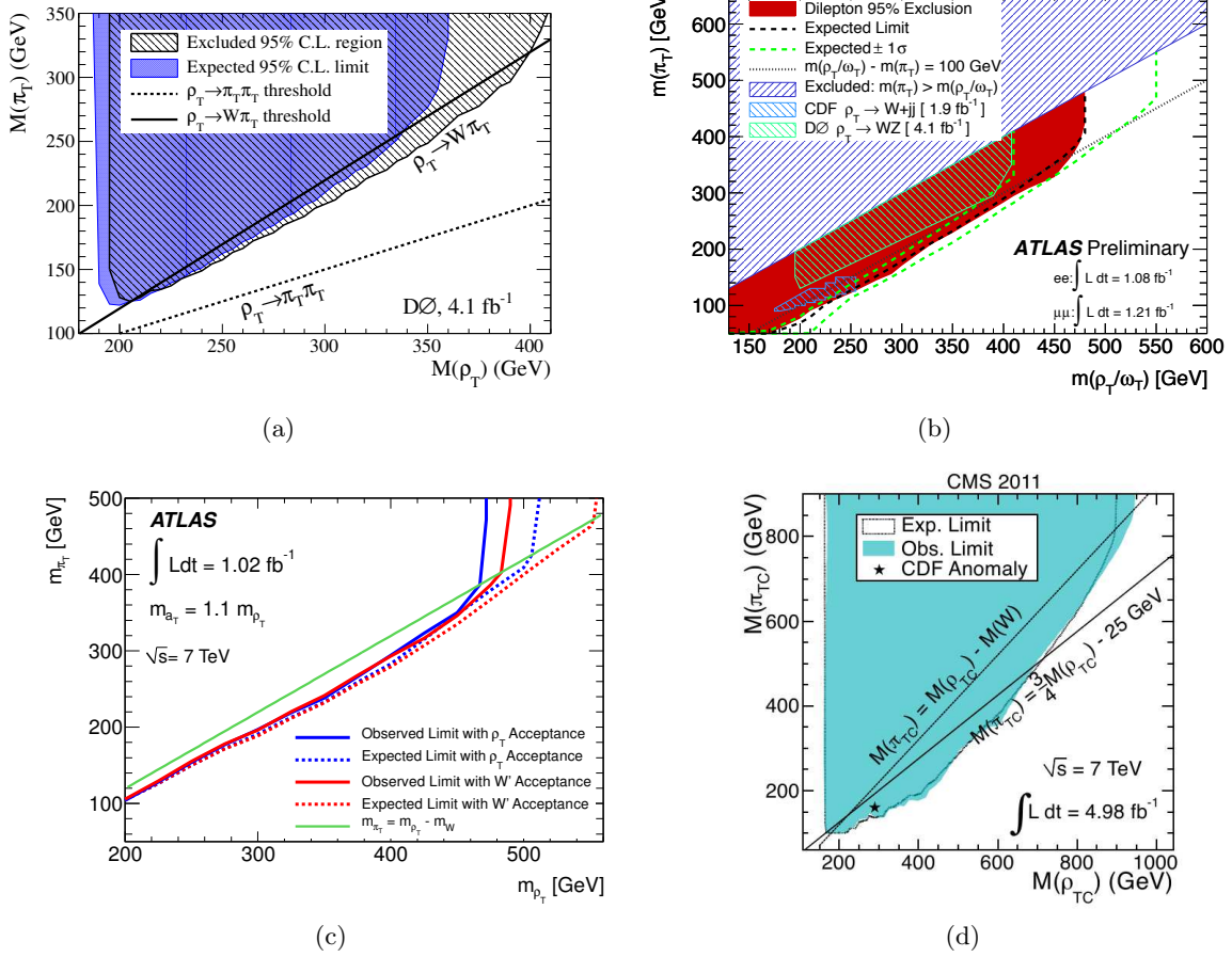
Figure 1.8: Current limits on LSTC. (a) 95% exclusion region in the plane of \rho_T vs. \pi_T masses in WZ \rightarrow ll\nu channel from the D\emptyset collaboration, using 4.1 \text{ fb}^{-1} of data [45]. (b) 95% exclusion region in the plane of \rho_T vs. \pi_T masses from the ATLAS collaboration, in \rho_T/\omega_T \rightarrow ll decay channel where the a_T contribution is not taken into account. Are also quoted the previous exclusion limits from CDF and D\emptyset collaborations [36]. (c) The 95% CL expected and observed excluded mass regions in the plane of \rho_T vs. \pi_T masses in WZ \rightarrow ll\nu channel from the ATLAS collaboration using \sim 1 \text{ fb}^{-1} of data [37]. (d) The 95% exclusion region in the plane of \rho_T vs. \pi_T masses in WZ \rightarrow ll\nu channel from the CMS collaboration, using 5 \text{ fb}^{-1} of data [38].
