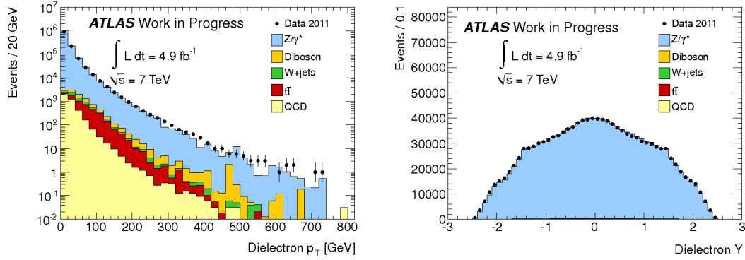
Figure 5.10: Dielectron p_T and rapidity after event selection.
