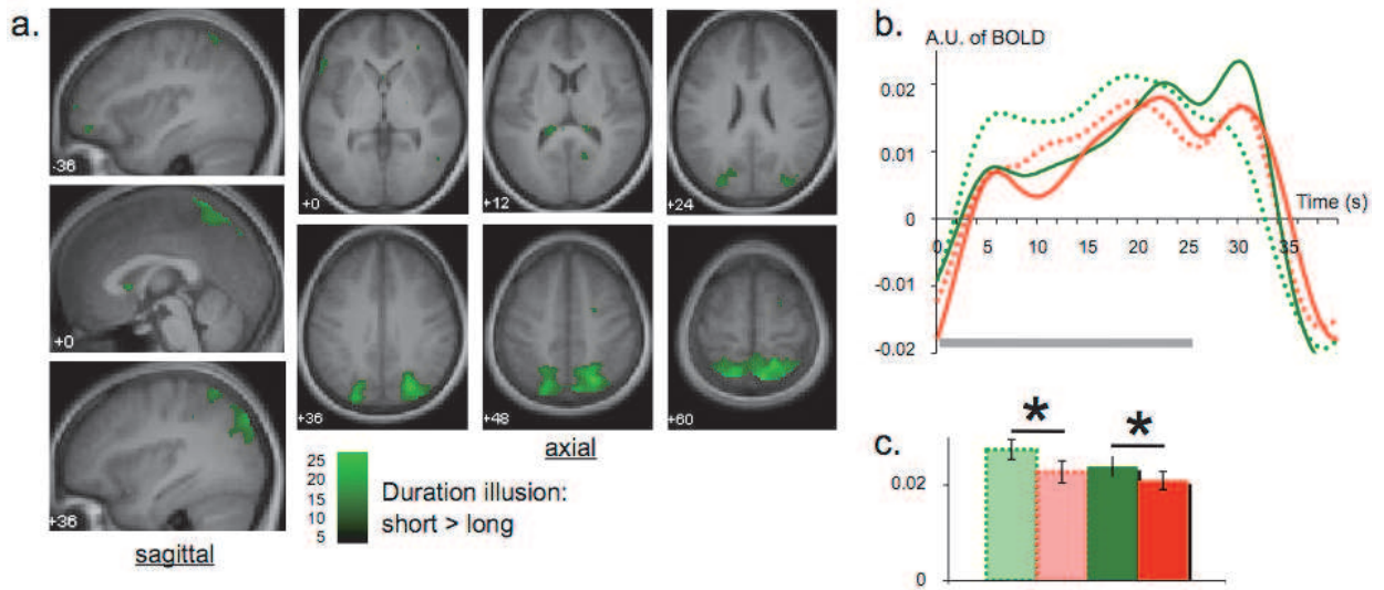
Figure 5: Independent component 23 showing an effect of duration illusion (short > long). (a) Activation map (thresholded at p < 0.001 FWE), (b) event-related averages of the time course adjusted for each condition, level of activation in arbitrary units over a 40 s period, the grey bar corresponds with the painful stimulation and (c) mean beta-weights ( \pm SEM) for each condition ( * p < 0.1 ). Slices representing axial and sagittal positions are in MNI space. Light/dashed: medium temperature; dark/solid: high temperature. Green: short duration; red: long duration.
