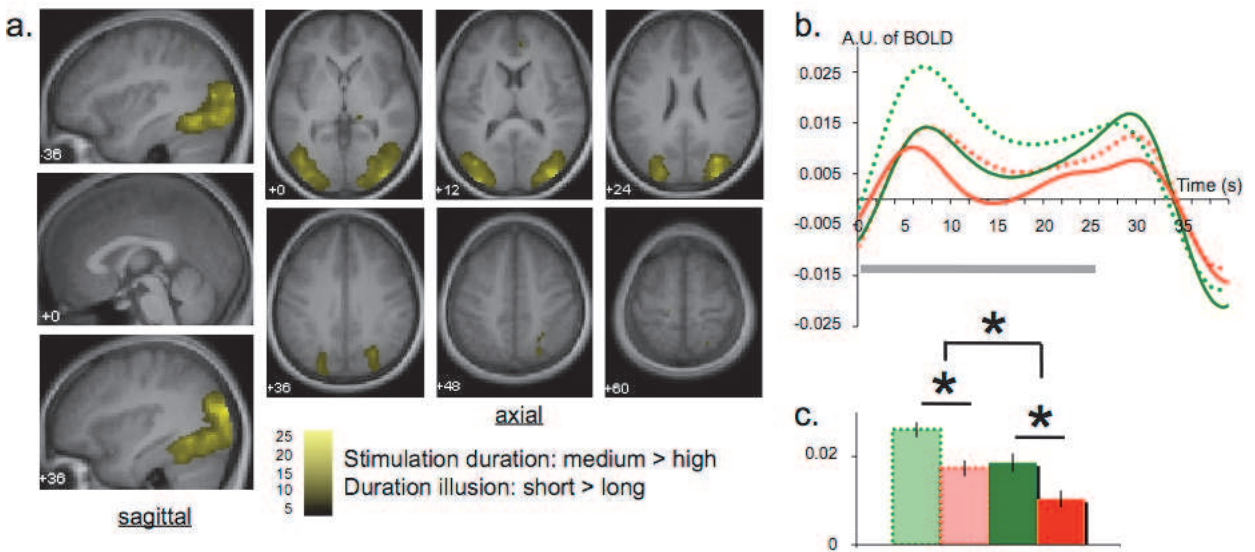
Figure 6: Independent component 29 showing an effect of duration illusion (short > long) and of stimulation intensity (medium > high). (a) Activation map (thresholded at p < 0.001 FWE), (b) event-related averages of the time course adjusted for each condition, level of activation in arbitrary units over a 40 s period, the grey bar corresponds with the painful stimulation and (c) mean beta-weights ( \pm SEM) for each condition ( * p < 0.1 ). Slices representing axial and sagittal positions are in MNI space. Light/dashed: medium temperature; dark/solid: high temperature. Green: short duration; red: long duration.
