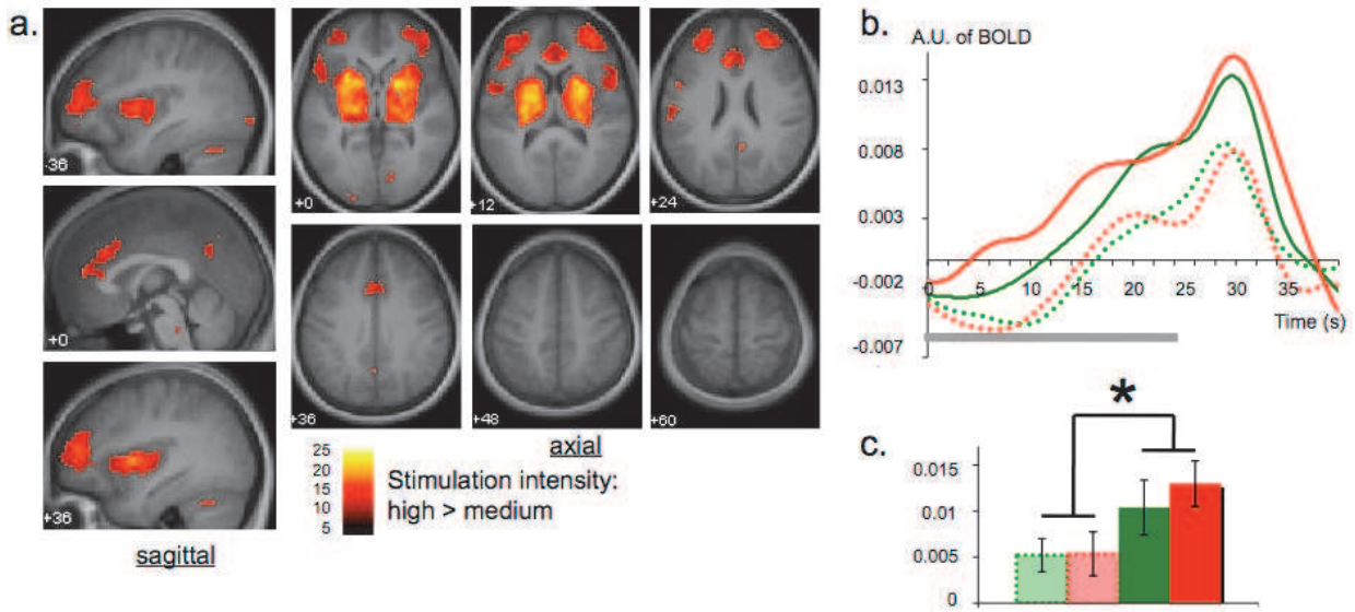
Figure 3: Independent component 30 showing an effect of stimulation intensity (high > medium). (a) Activation map (thresholded at p < 0.001 FWE), (b) event-related averages of the time course adjusted for each condition, level of activation in arbitrary units over a 40 s period, the grey bar corresponds with the painful stimulation and (c) mean beta-weights ( \pm SEM) for each condition (* p < 0.1 ). Slices representing axial and sagittal positions are in MNI space. Light/dashed: medium temperature; dark/solid: high temperature. Green: short duration; red: long duration.
