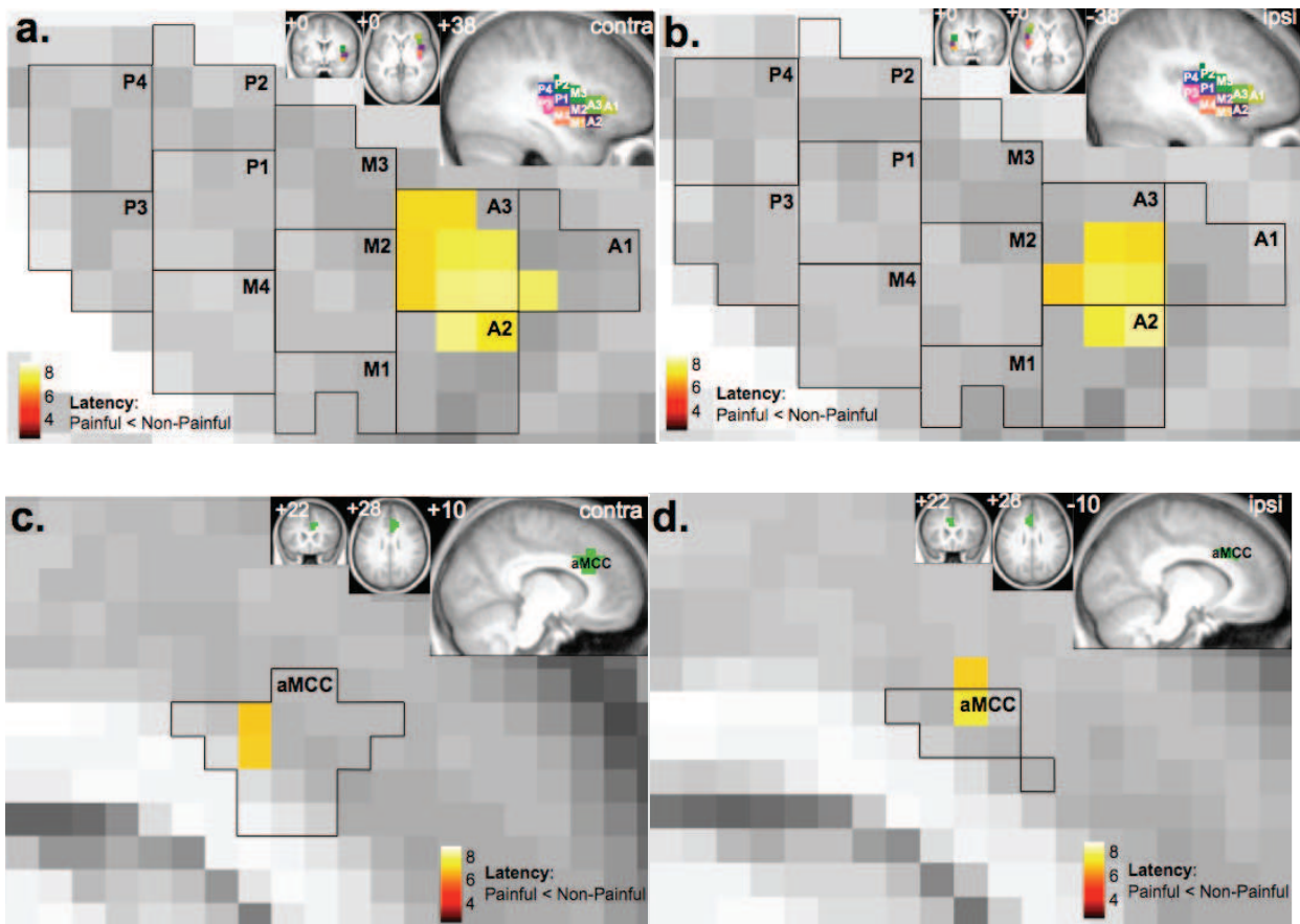
Figure 7: Map of latency differences.
