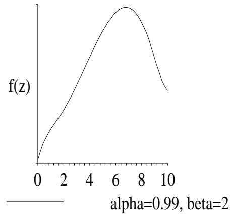
Figure 4.3: Proportional fair objective function f_\alpha given by (4.4) with \alpha \approx 1 , as function of BS location z . User density \lambda(x) = x , \beta = 2
