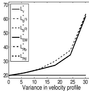
Figure 3.6: Optimal cell size versus variance of the velocity.
