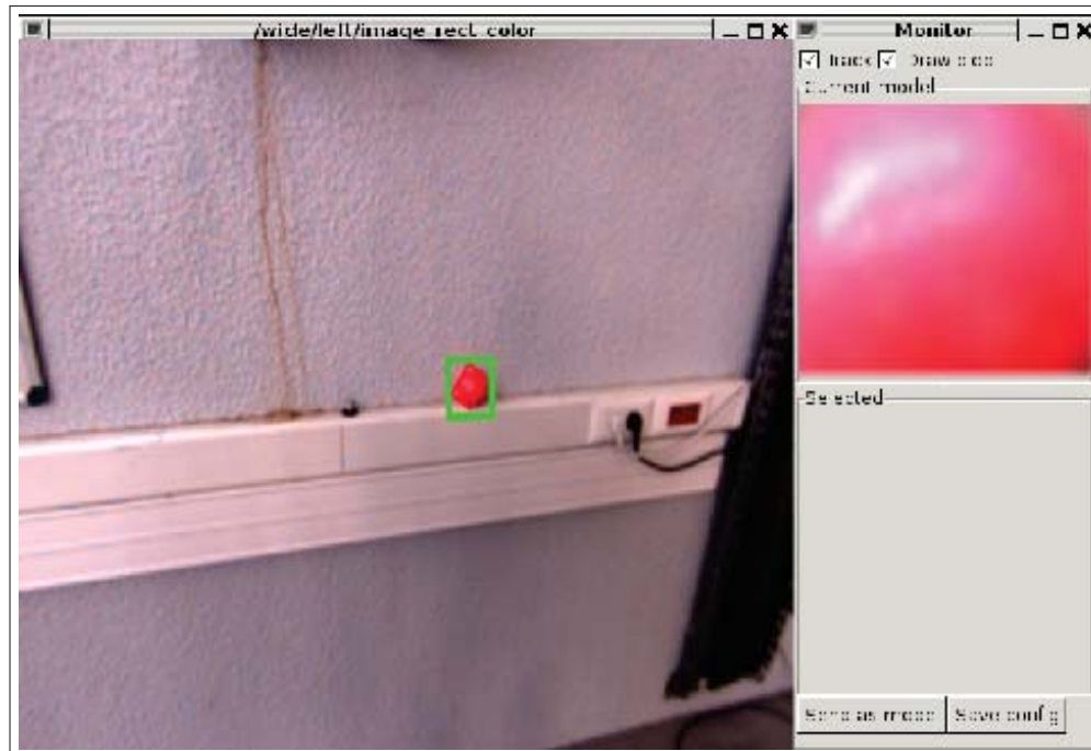
Figure 4.4: Hueblob interface
