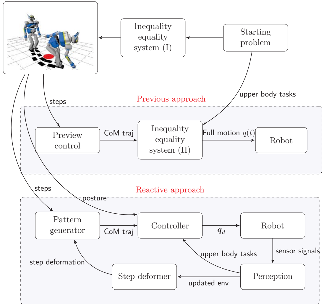
Figure 3.1: Reactive walking vs. offline computed walking
