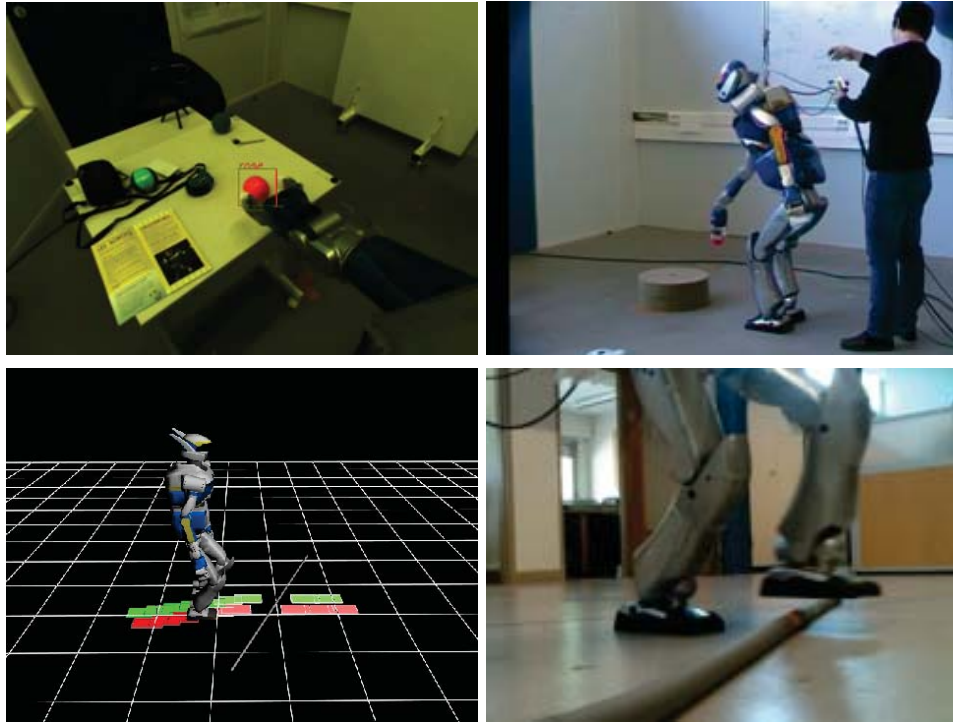
Figure 1.6: Experiments on HRP-2 using the real-time footstep optimization
