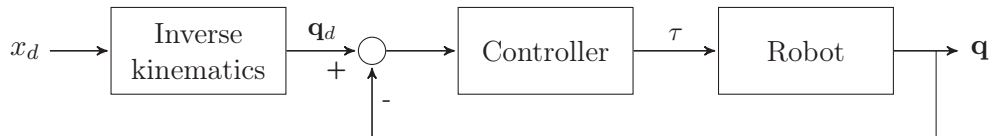
Figure 2.7: Joint space controller
