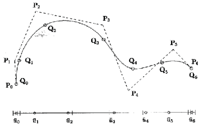
Figure 6.6: Cubic spline
