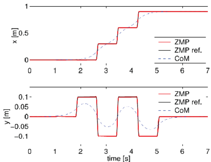
Figure 2.14: Tracking performance for preview windows 1.6s
