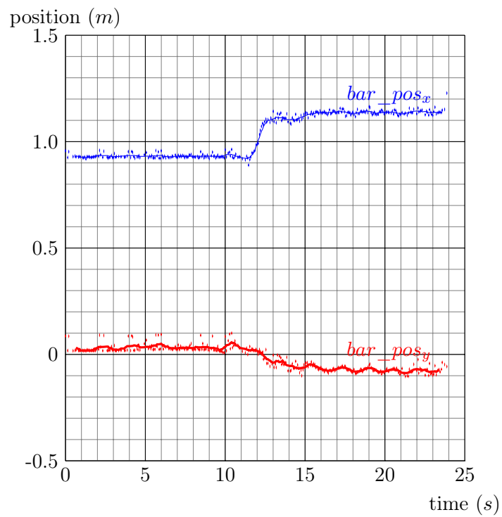
Figure 5.9: Perceived position of the bar ( x and y components) which is moved while the robot is walking (around second 12).
