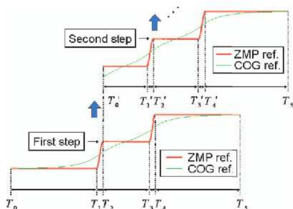
Figure 2.17: Step scheduling with analytical CoM strategy
