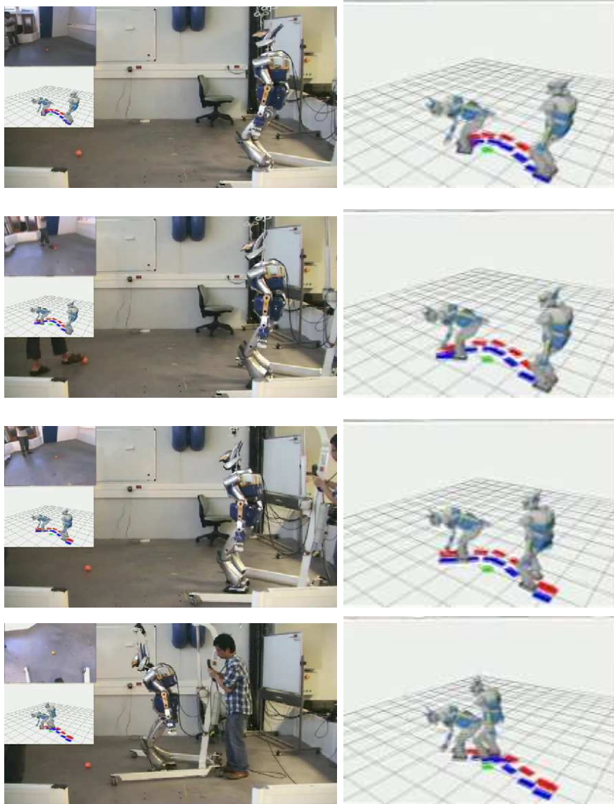
Figure 6.11: Foot step adaptation during a grasping movement. This experiment illustrates how the robot adapts its footsteps (right figures). The target is pushed while the robot walks.
