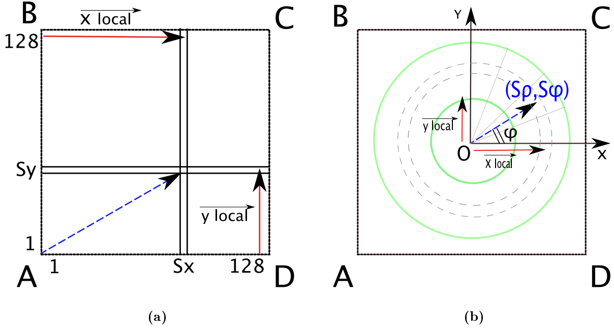
Figure 3.17: Reconstruction of the hit position with respect to the local system of MUST2 (a) and S1 (b) detectors.
