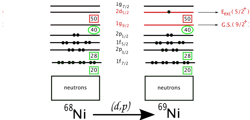
Figure 1.12: On the left hand side a shell-model of the ^{68}\text{Ni} . A (d,p) reaction on ^{68}\text{Ni} transfers a neutron to its empty orbitals and infers the single-particle structure of ^{69}\text{Ni} nucleus (right hand side).
