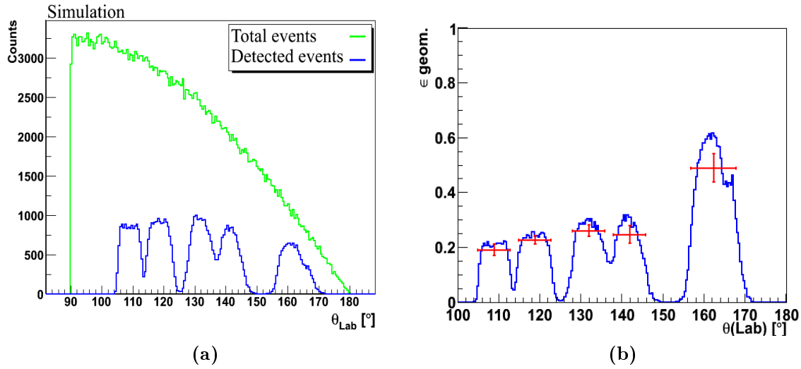
Figure 3.19: The histograms are obtained from simulated data. (a) The green line shows the total emitted particles, from an isotropic source in the laboratory-reference system placed at the target position. The histogram in blue represents only the detected particles by the detection system placed in the backward angles. (b) Histogram showing the ratio of detected events over total number of events for each bin. The ratio gives the geometrical efficiency of the detection system. The horizontal bars in the red crosses correspond to the angular ranges used in the analysis while the vertical bars represent the error on the calculated efficiency.
