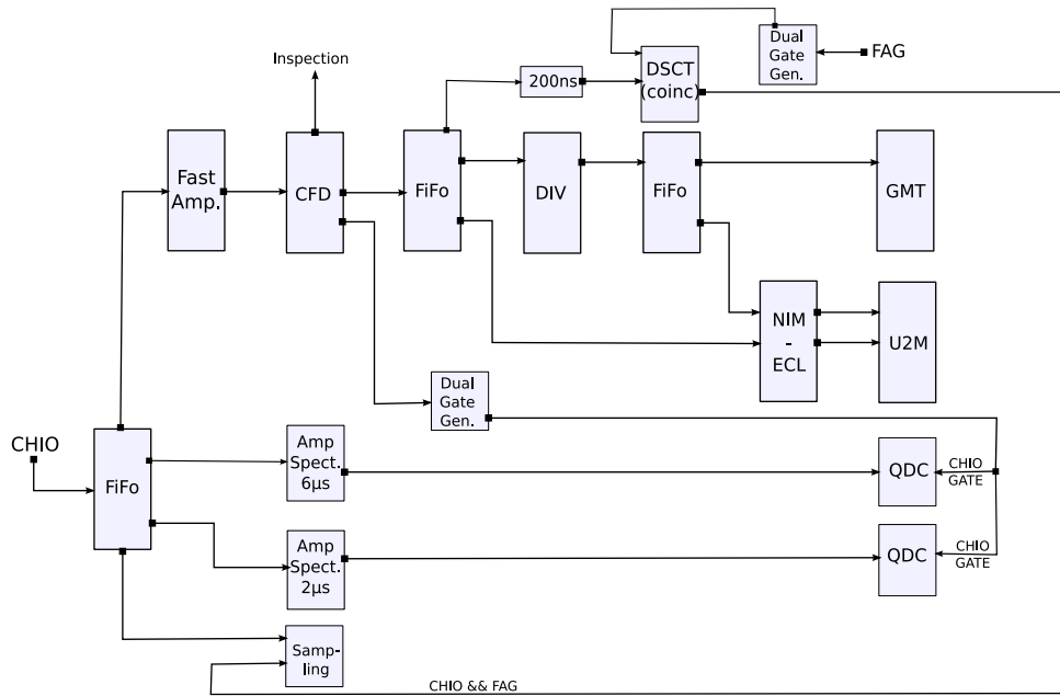
Figure B.4: Electronic diagram associated to the ionization chamber. The time signal is used as a gate to encode the energy signal from the chamber deposited by the particle (QDC). The same signal in coincidence with FAG generates a gate to enable sampling. The time signal is also sent to the scalers (U2M) and to GMT after division.
