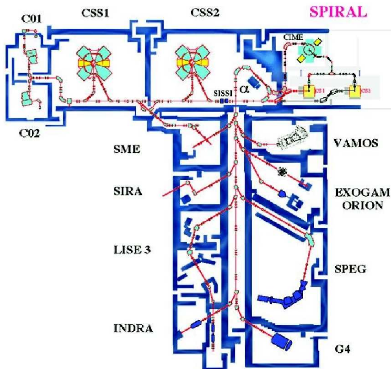
Figure 2.4: GANIL facility and its different installations.
