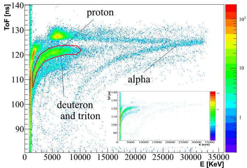
Figure 3.12: Particle identification by E - \text{ToF} technique in S1 detector. Proton, deuteron and alpha particles can be clearly identified by their maximum deposited energies in S1 . The insert shows the E - \text{ToF} spectrum when Ni isotopes are requested in the plastic detector..
