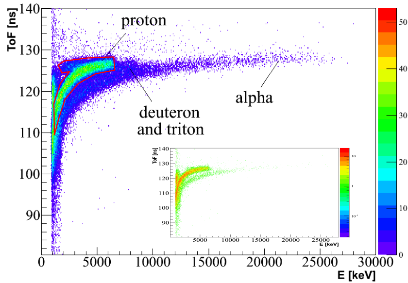
Figure 3.11: Particle identification by E - \text{ToF} technique in MUST2 first stage. The insert shows the E - \text{ToF} spectrum when Ni isotopes are requested in the plastic detector.
