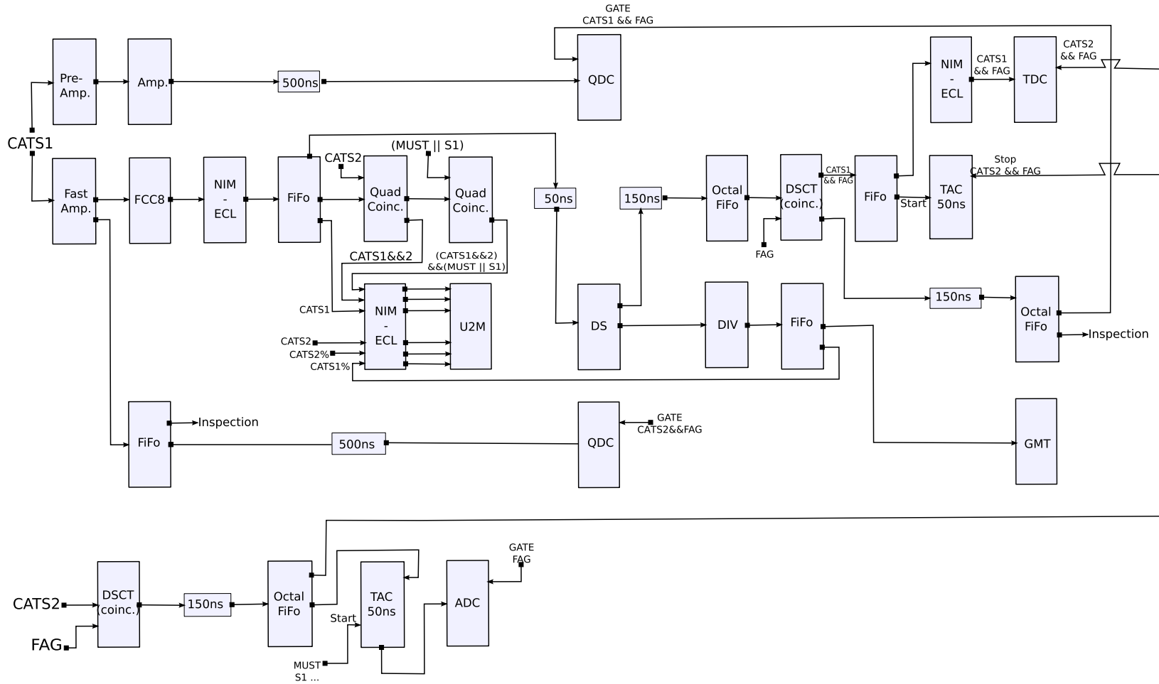
Figure B.1: Electronic diagram of the time and charge signals of CATS1 and CATS2. The coincidence of the time signal from CATS1 (CATS2) with the FAG is used as a start (stop) signal for TACs and TDCs and as gates for QDCs. The time signal of CATS2 is also used as a stop signal for all other detectors to measure time-of-flight. The use of TACs and TDCs is redundant but ensures a time measurement in case of failure. The charge signals from CATS1 (CATS2) are authorized to trigger the acquisition once every 1000 (3000) detected events.
