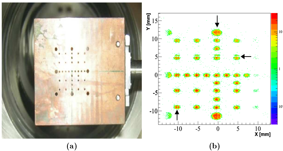
Figure 3.2: (a) Grid placed behind CATS1. (b) Reconstruction using X_3^{COG} with correction factors given in table 3.2 .
