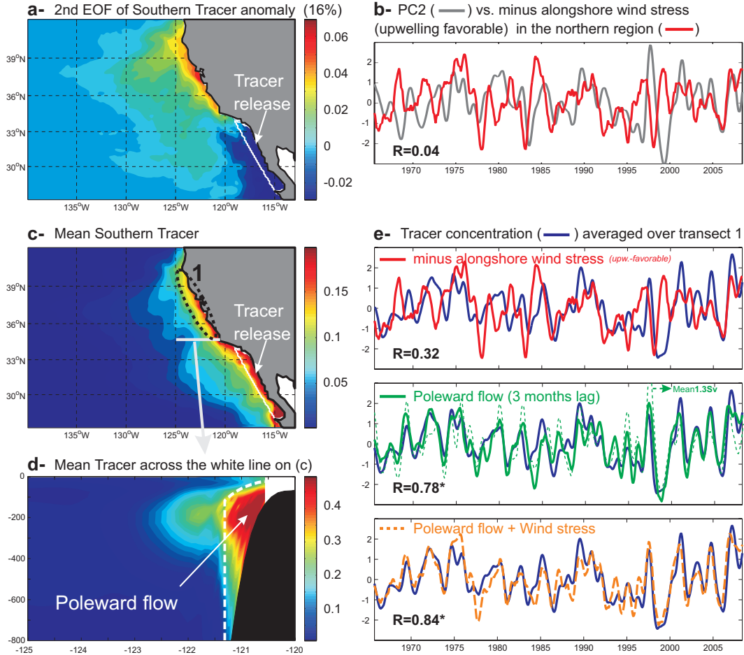
FIGURE 3.8 – Tracer is released in the SUBSURFACE and in the SOUTHERN region. Time series are anomalies and normalized. 2nd EOF (a) and Principal component (b; grey line) of that tracer. (c-d) mean tracer at the surface and across the white line in (c). (e) compares the tracer at the surface in the northern region (blue) with the alongshore wind stress (red) and with the strength of the poleward flow (green; defined as the tracer averaged over the surface delimited by the white dashed line in (b) - dashed green : defined as the meridional transport averaged over the region where \text{Tracer} > 0.3 ). Orange dashed line represents a linear model of poleward flow (green line) and alongshore wind stress (red line).
