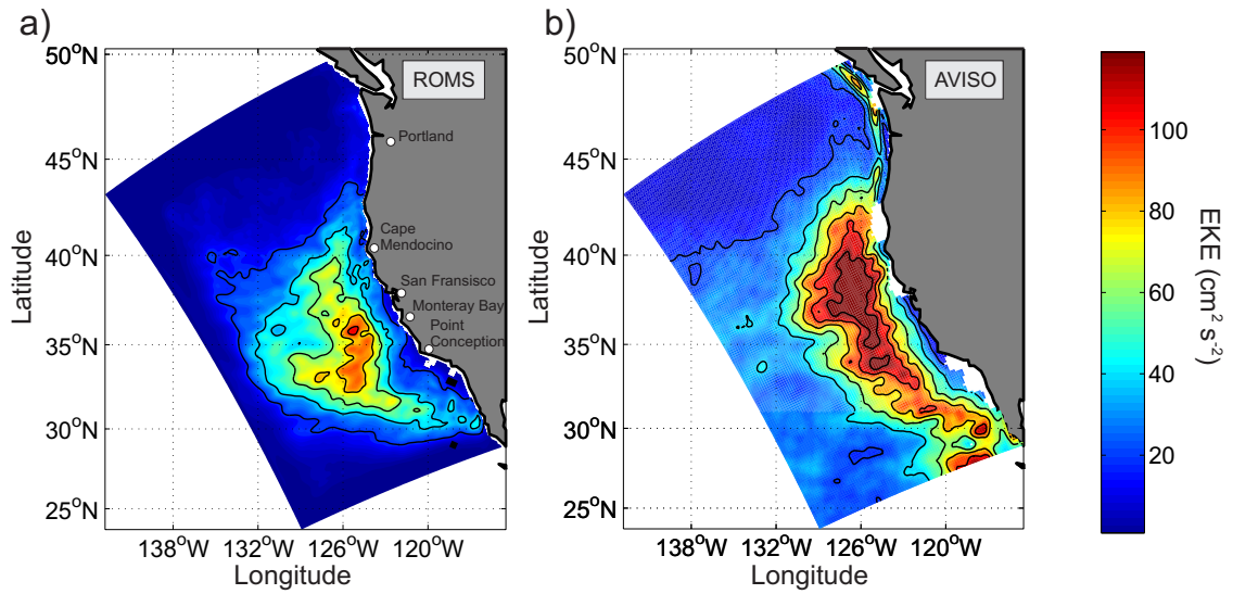
FIGURE 5.6 – Annual mean eddy kinetic energy ( EKE ) from (a) the model and (b) satellite-derived SSH observations (AVISO, 1992-2009). Units : cm^2/s^2 . The contour interval is 20 cm^2/s^2 .
