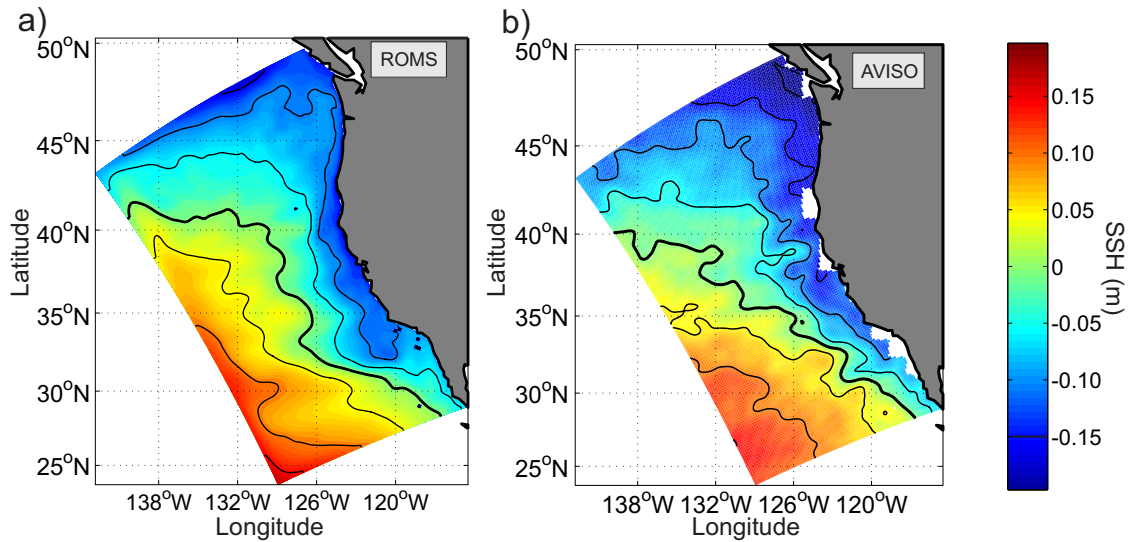
FIGURE 5.7 – Annual mean sea surface height ( SSH ) from (a) the model and (b) satellite-derived SSH observations (AVISO, 1992-2009). Units : m . The contour interval is 0.05 m and the 0 m contour is in bold.
