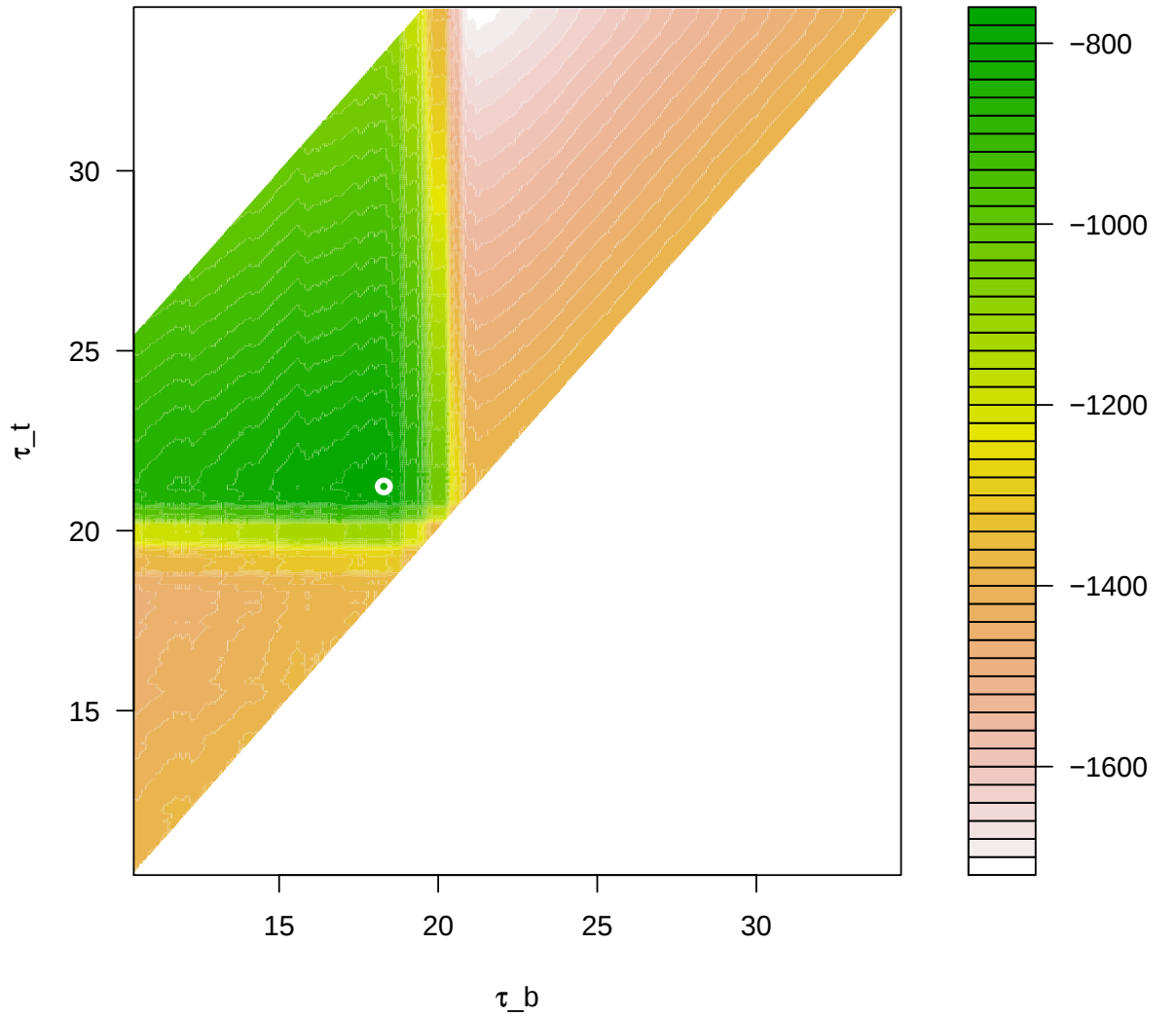
FIGURE 3.7 – The likelihood \mathcal{L} as a function of the cloud bottom \tau_b and top \tau_t altitude for the measured backscatter profile of Figure 3.6. The maximum of \mathcal{L} is indicated with an open circle.
