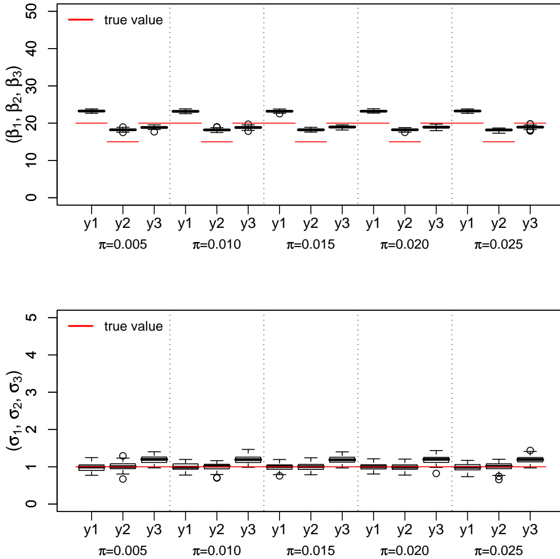
FIGURE 5.9 – Same as in Figure 5.8 but with a fixed (\sigma_1, \sigma_2, \sigma_3)^T = (1.0, 1.0, 1.0)^T and five different \pi = 0.005, 0.010, 0.015, 0.020, \text{ or } 0.025 .
