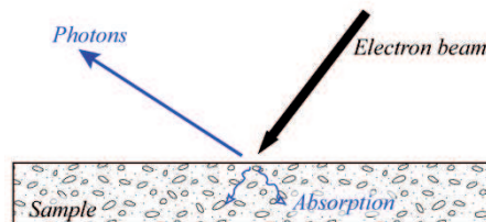
Figure A.1. Scheme of the cathodoluminescence phenomenon.
