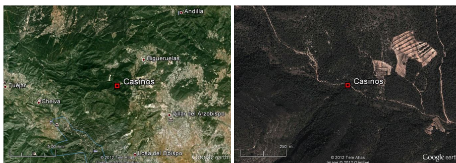
Figure 3.17 Idem figure 3.13 mais pour “Casinos”.
