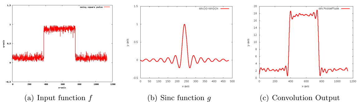
Figure 3.5: Convolution of a noisy input function (a) with a Sinc function (b). (c) the result function of the convolution. Note how the perturbed data is reduced while maintaining the sharp discontinuities in the data.
