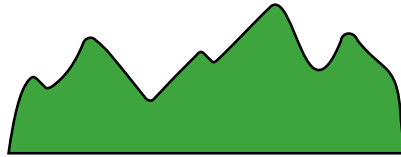
Figure 4.4: A continuous smooth histogram based on a Gaussian distribution.
