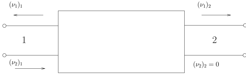
Figure 1.8: Reflectometry on a two-port network
