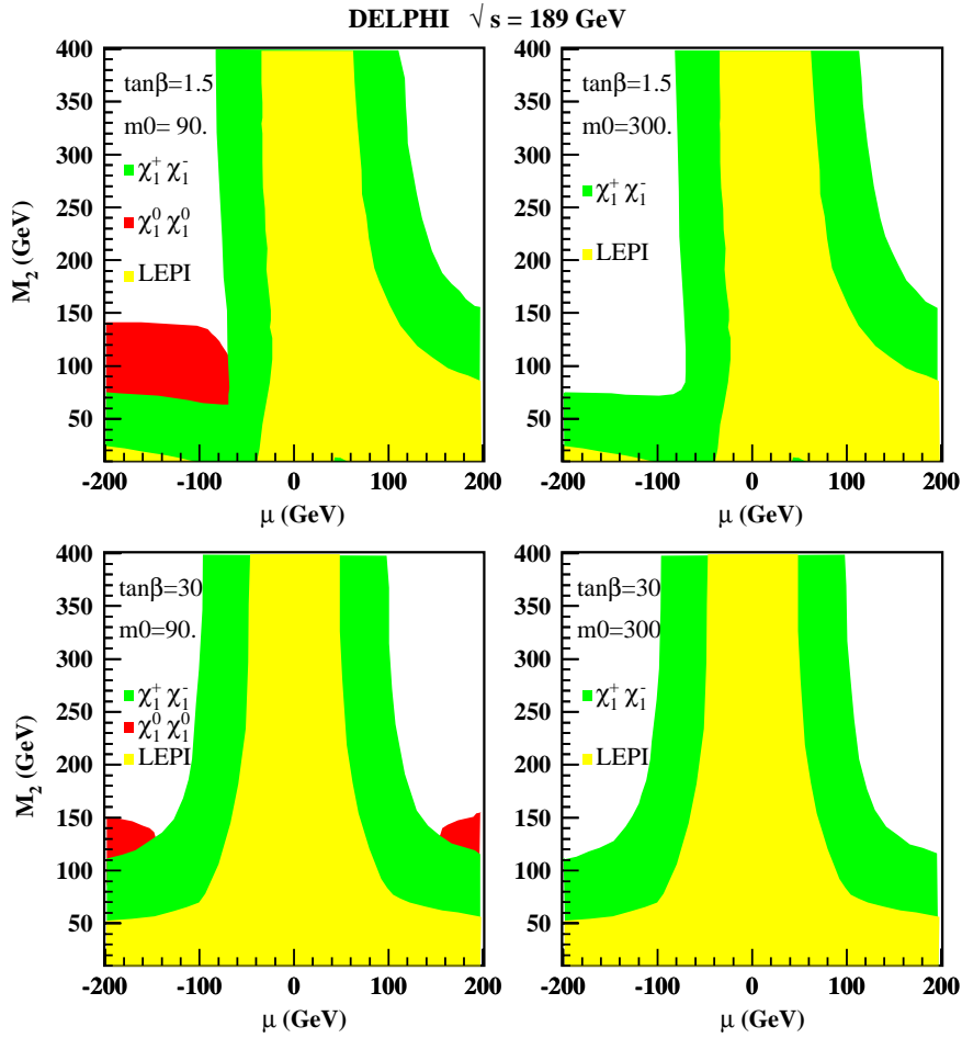
Fig. 7.9. Regions in the (\mu, M_2) plane excluded at 95% CL for \tan\beta = 1.5, 30 and m_0 = 90, 300 \text{ GeV} in the case of a dominant \bar{U}\bar{D}\bar{D} coupling [445].
