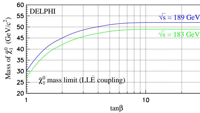
Fig. 7.10. The lightest non-excluded neutralino mass as a function of \tan\beta at 95% CL . This limit is independent of the choice of m_0 in the explored range and of the generation indices i, j, k of the \lambda_{ijk} coupling [445] and it assumes that the \tilde{\chi}_1^0 is in the detector.
