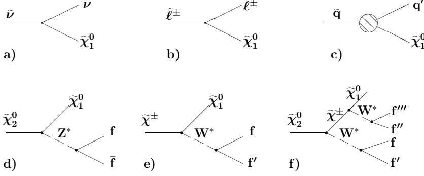
Fig. 2. Diagrams of sparticle R_p -conserving decays. To get the whole chain of the sparticle indirect decay, the LSP (lightest neutralino) has to undergo a direct R_p -violating decay. a,b slepton decays into a lepton and the lightest neutralino; c squark decay into a quark and the lightest neutralino, the hatched disk means decay beyond tree level for the stop case; d-f examples of gaugino decays
