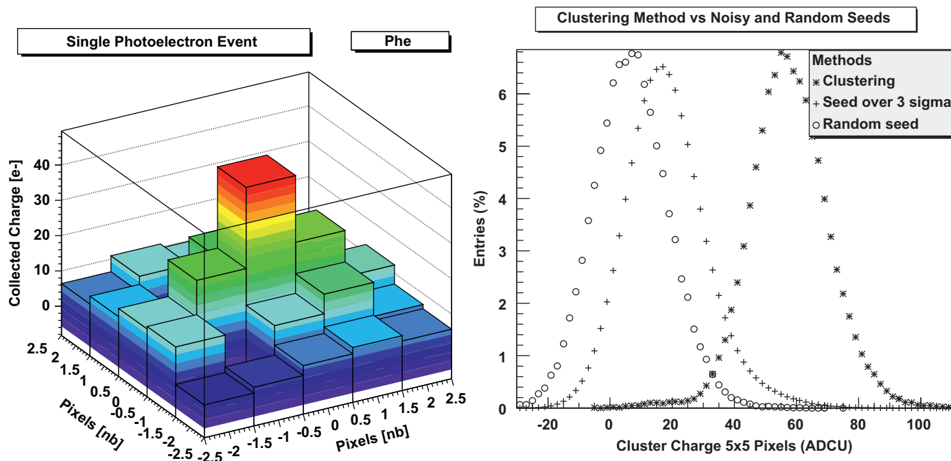
Fig. 7. Single photo-electron event recorded for HV=2.8 kV (left). The single photo-electron spectrum corresponds to the sum of 5 \times 5 pixels centred around the seed pixel (right). To illustrate the power of the selection, the same 5 \times 5 cluster is shown with random selection (circle) or on selected seed pixel with SNR greater than 3 (cross). The single photo-electron spectrum is clearly above the pixel noise.
