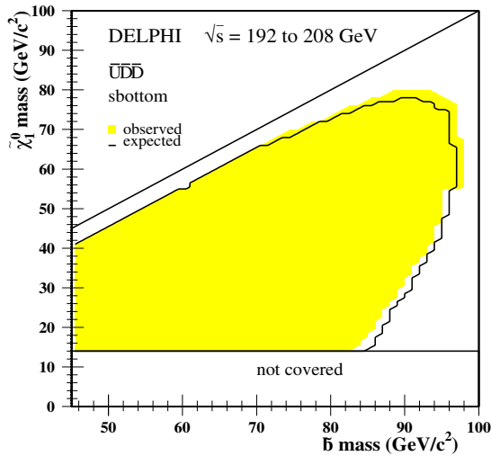
Fig. 19. \bar{U}\bar{D}\bar{D} : exclusion contours at 95% CL in the m_{\tilde{\chi}_1^0} versus m_{\tilde{b}} plane for the sbottom pair-production, with \text{BR}(\tilde{b} \rightarrow b\tilde{\chi}_1^0) = 100\% and neutralino decay into jets. The plot shows the obtained exclusion (filled area) for the lightest sbottom in the case of no mixing. The black contour is the expected exclusion at 95% CL
