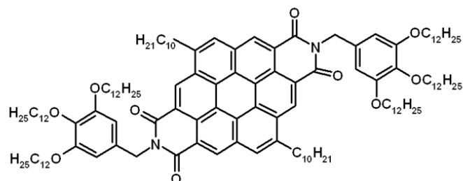
Coronene-BZ
