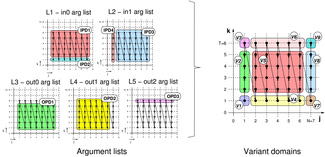
Figure 5.8.: Deriving the variant domains corresponding to a process
