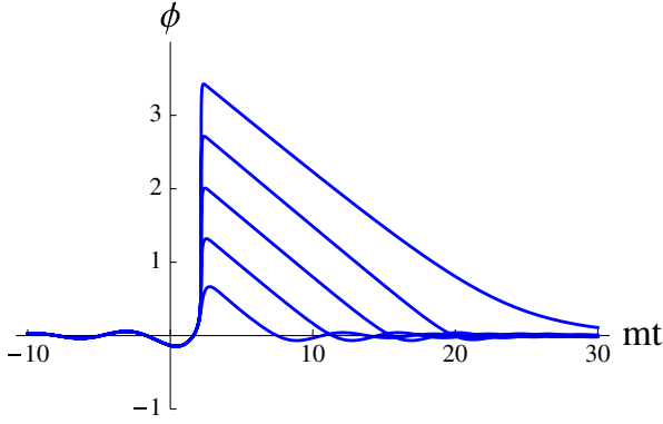
FIG. 5 (color online). The shark fin-type evolution of the scalar field for m = 10^{-3}m_{\text{Pl}} . Curves from bottom to top were computed for \rho_c = 10^{-6}, 10^{-4}, 10^{-2}, 1, \text{ and } 100[m_{\text{Pl}}^4] , respectively.
