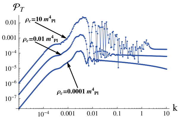
FIG. 11 (color online). Numerically computed power spectra for \rho_c = 10^{-4}, 10^{-2}, 10m_{\text{Pl}}^4 (from bottom to top in the UV range) with m = 10^{-3}m_{\text{Pl}} .
