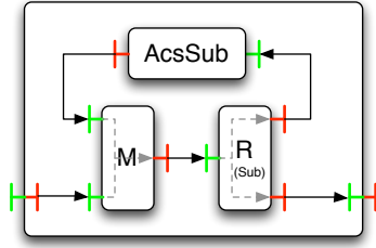
FIGURE A.1 – Le composant TheLoop
