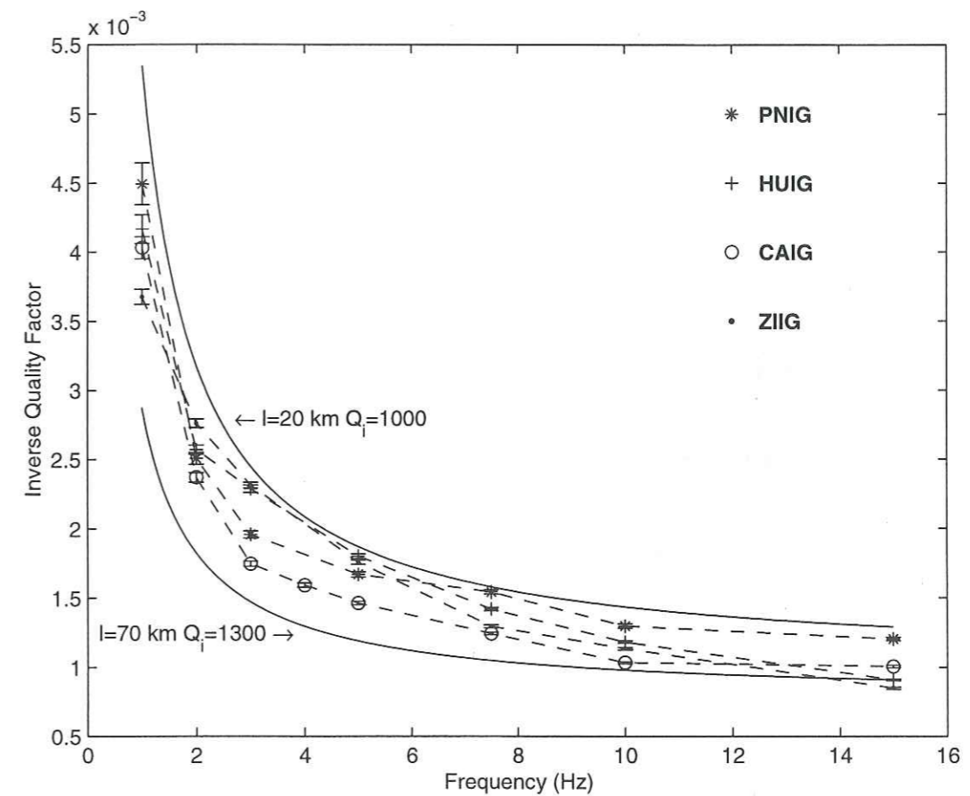
FIG. 5.4 - A comparison of the measured values of Q_c with the ones deduced from our model including a weak intrinsic absorption.
