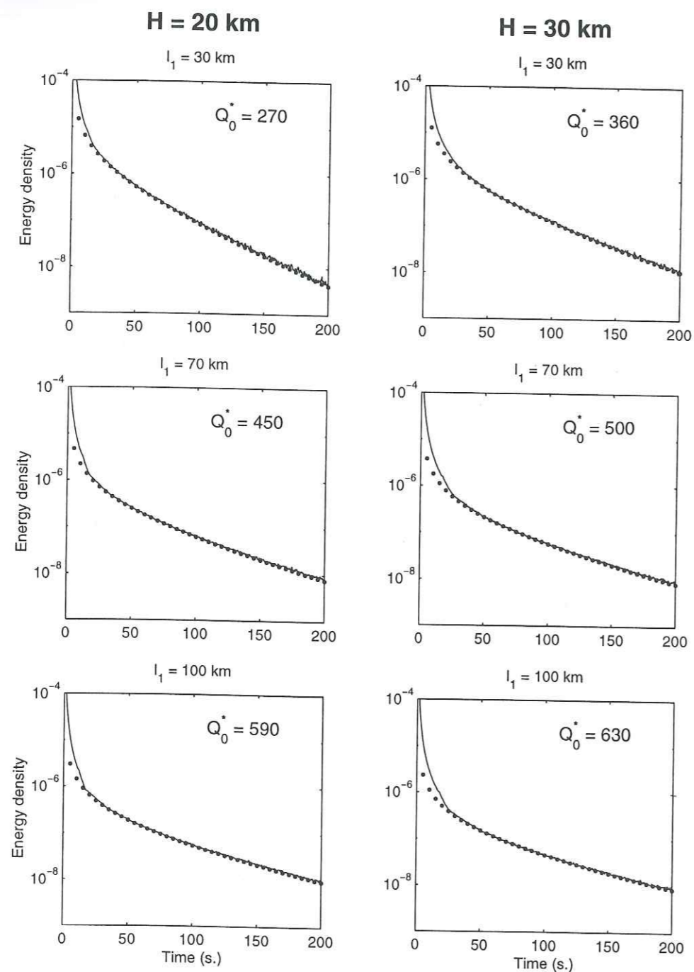
FIG. 3.2 - Coda decay obtained for our model with H = 20 km, H = 30 km, and the mean free path of the crust l ranging from 30 km to 100 km. Solid lines show the numerical solution of the Radiative Transfer Equation, while dotted lines show the best approximation obtained with the formula \frac{1}{t} \exp(-\frac{2\pi t}{Q_0^*}) . The Q_0^* value corresponding to the best approximation is given in the figures. The maximum standard deviation of the Q_0^* is \Delta Q_0^* \approx 30 .
