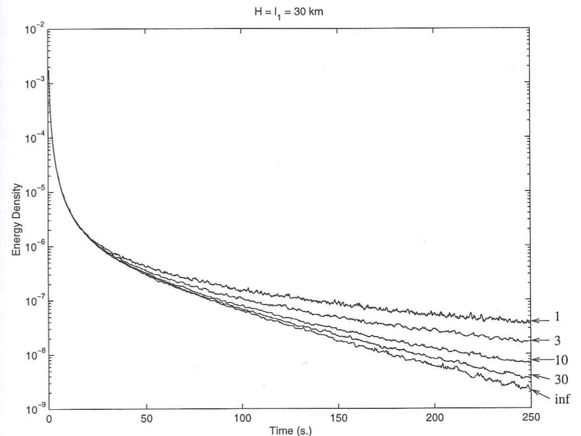
FIG. 3.4 – Effect of the mean free path contrast on the shape of the synthetic codas. The ratio of the crustal to the mantle mean free path is indicated in front of each curve. One can observe the steady transition from the algebraic decay t^{-3/2} , when there is no contrast, to the exponential decay 1/t \exp(-t/\tau_d) , when the mantle is transparent.
