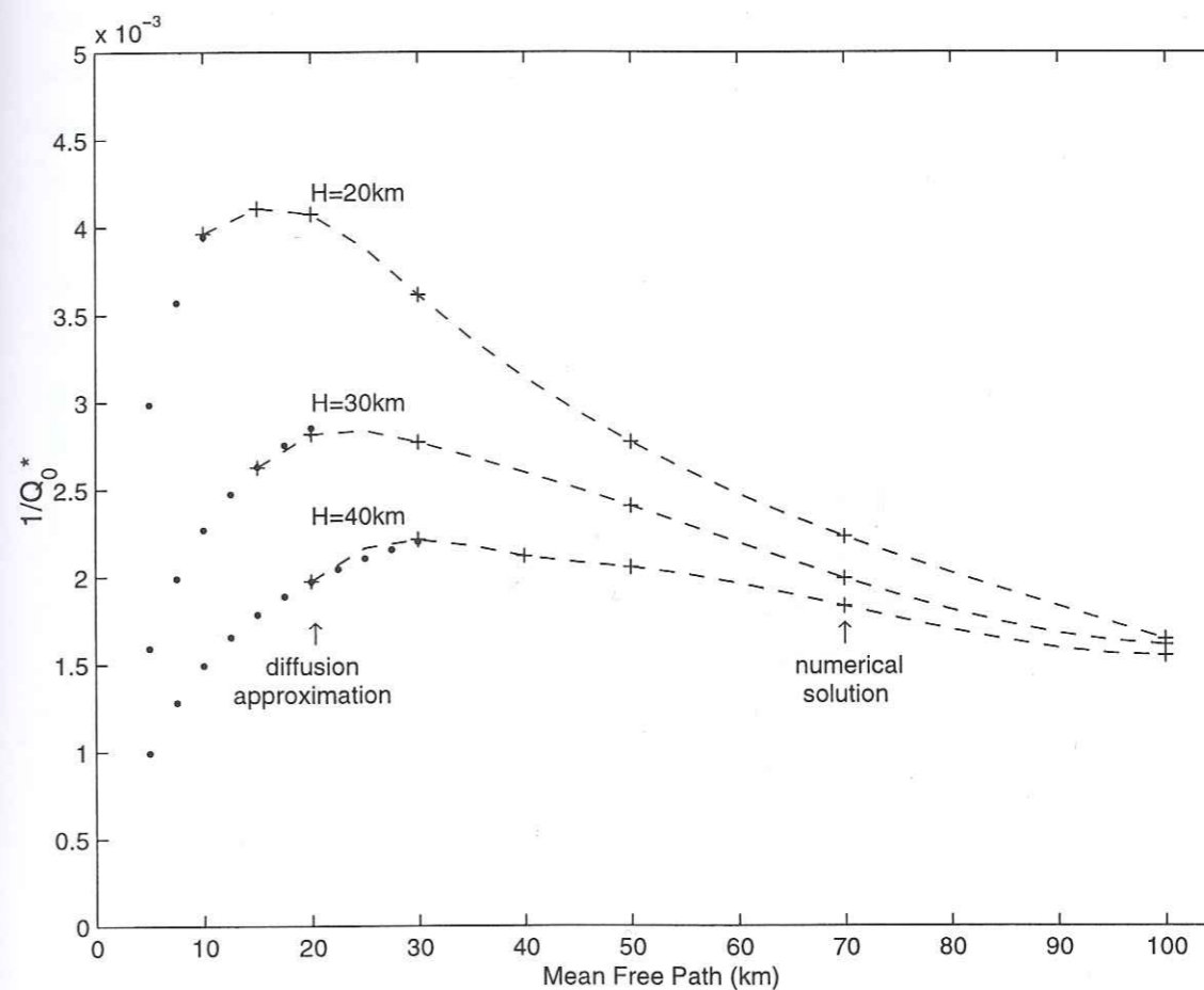
FIG. 3.3 - Dependence of the parameter 1/Q_0^* on the mean free path l for three crustal thicknesses H = 20, 30, 40 km. Dots correspond to the values calculated with the diffusion approximation, while crosses denote the values estimated numerically with the radiative transfer theory. Both coincide for l < H . The dashed line interpolates between the crosses.
