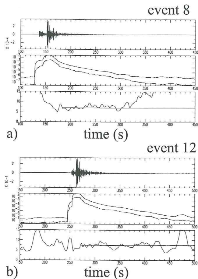
FIG. 5.7 – Examples of measurements . We selected events with different epicentral distances and backazimuths: a) event 8; b) event 12. For each event, we present the vertical component seismogram band-passed between 1 and 3 Hz (upper part), the P and S energies smoothed in a 16 s moving window (central part) and the S-to-P energy ratio (lower part).
