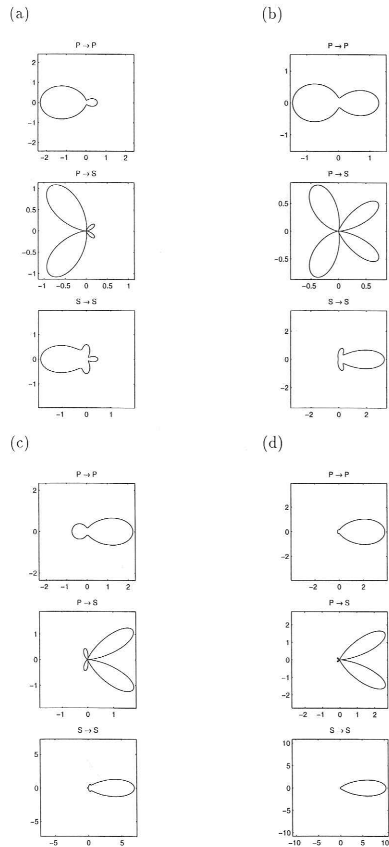
FIG. 4.6 – Polar plot of the differential scattering cross-sections for the mode conversions P-P, P-S and S-S. (a) Rayleigh Regime kpa \ll 1 (b) Rayleigh-Gans (R-G) Regime kpa = 1.2 (c) R-G kpa = 1.6 (d) R-G kpa = 2
