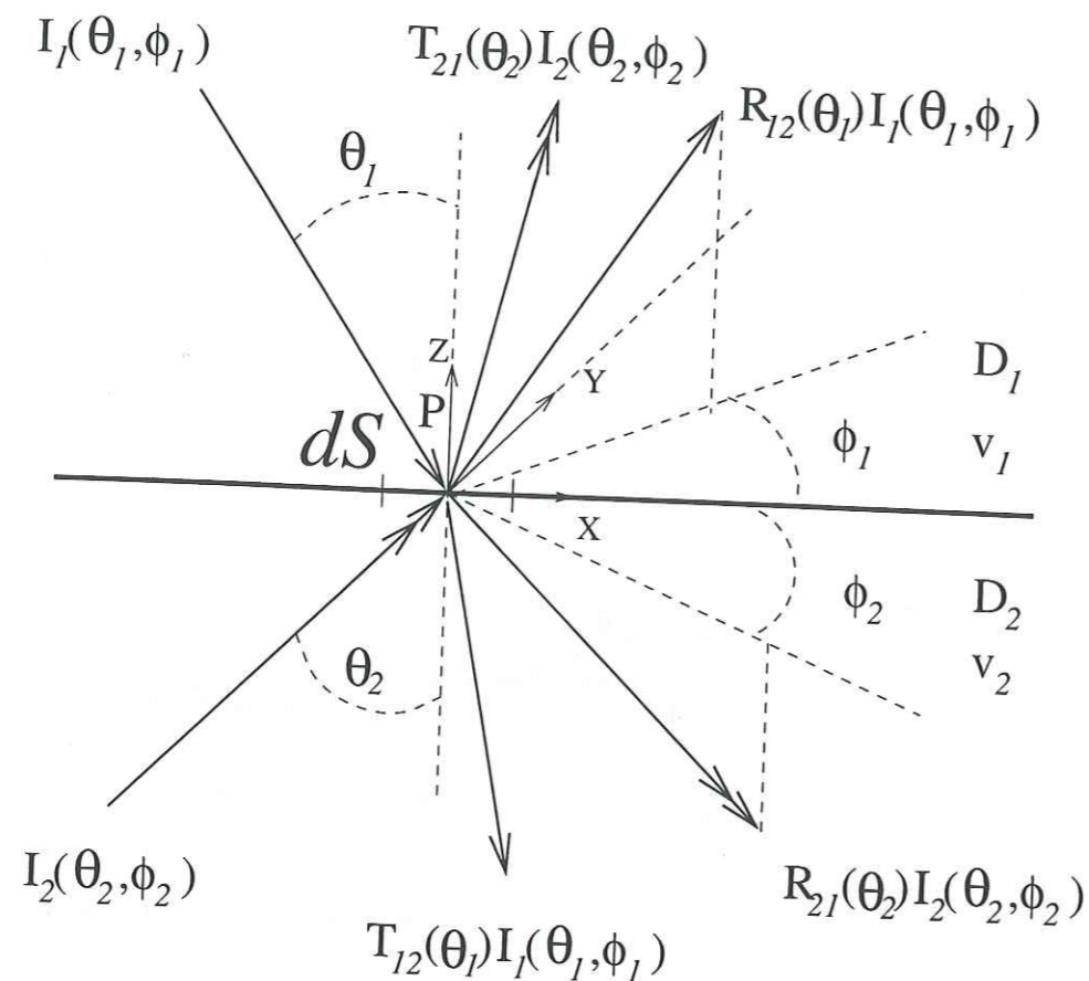
FIG. 2.5 - Energy balance at the interface between media 1 and 2. The beam 1 (resp. 2) has a single (resp. double) arrow. A beam of intensity I_i(\theta_i, \phi_i) is incident from medium i on a small surface element dS of the boundary of media i and j ( i, j = 1, 2 and i \neq j ). \theta_i and \phi_i are the angles of incidence of the beam i in spherical coordinates, the orthonormal reference frame being (\vec{x}, \vec{y}, \vec{z}) . The part of the beam i reflected in medium i is R_{ij}I_i . The part of the beam i transmitted in medium j is T_{ij}I_i .
