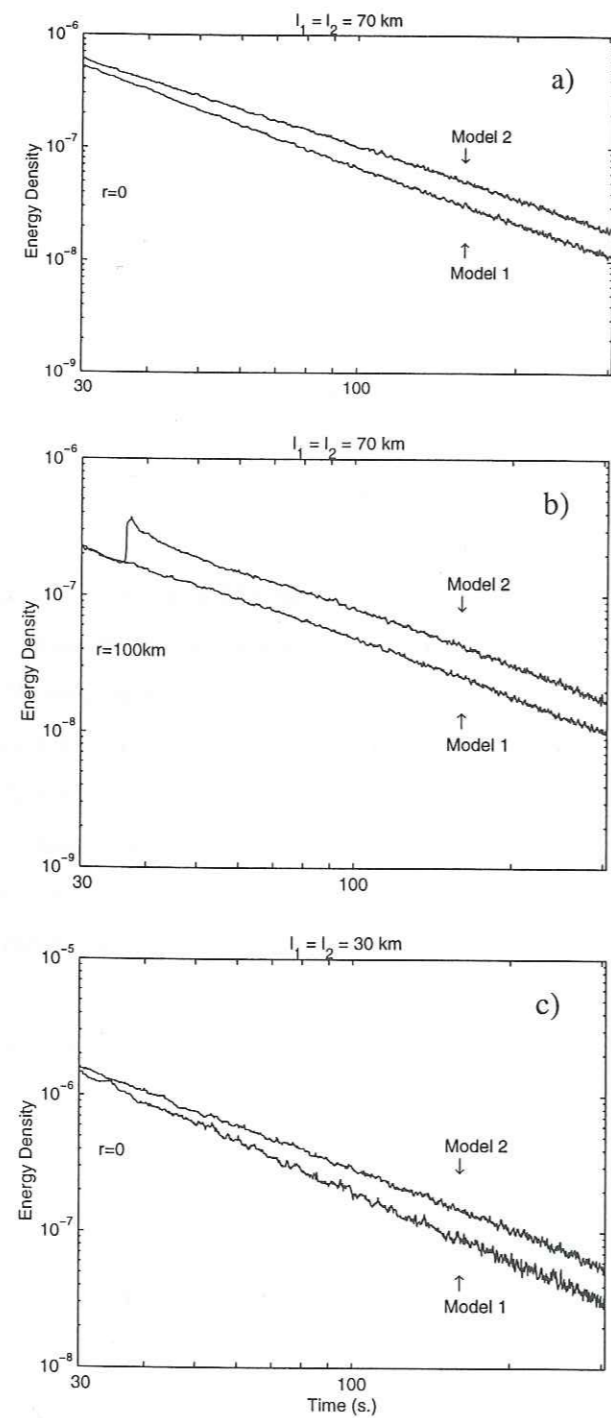
FIG. 2.8 – Comparison of the coda for models 1 and 2. The epicentral distance r is given in the figure. In both models, the mean free path is uniform and its value is indicated on top of each figure. For model 2 the upper layer thickness is H = 40 km and the velocity contrast is \frac{v_1}{v_2} = \frac{3.5}{4.7} . The time origin is the energy release at source.
