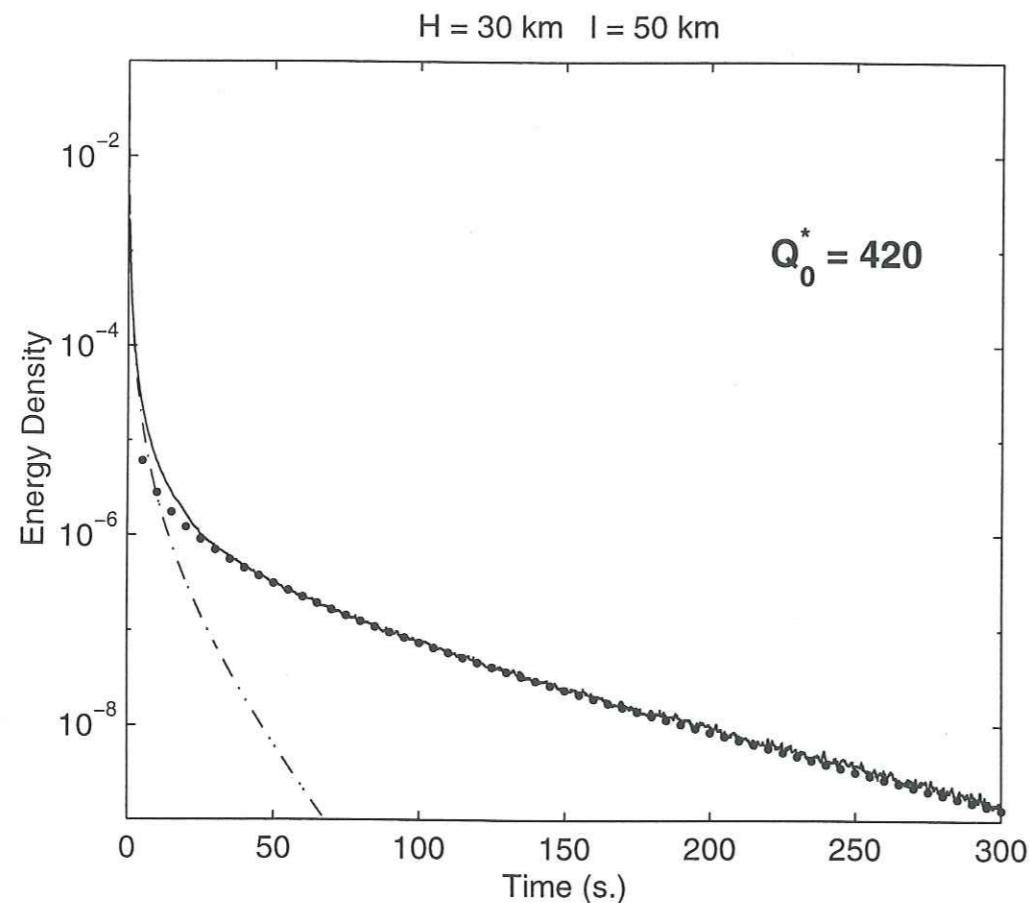
FIG. 5.2 – Coda decay obtained in our model with H = 30 km and the mean free path of the crust l equal to 50 km. Solid lines show the numerical solution of the Radiative Transfer Equation obtained by Monte Carlo modeling. The thin dotted lines shows the result of the single scattering approximation. The black circles indicate an approximation of the radiative transfer solution obtained with the formula \frac{1}{t} \exp(-\frac{2\pi t}{Q_0^*}) . The Q_0^* value corresponding to the best approximation is 420. The maximum standard deviation of the Q_0^* is \Delta Q_0^* \approx 30 .
