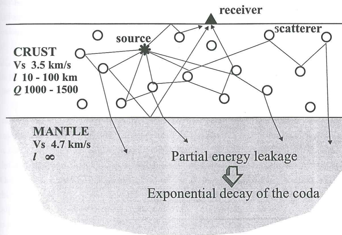
FIG. 3.1 - Geometry and physical parameters of the model.
