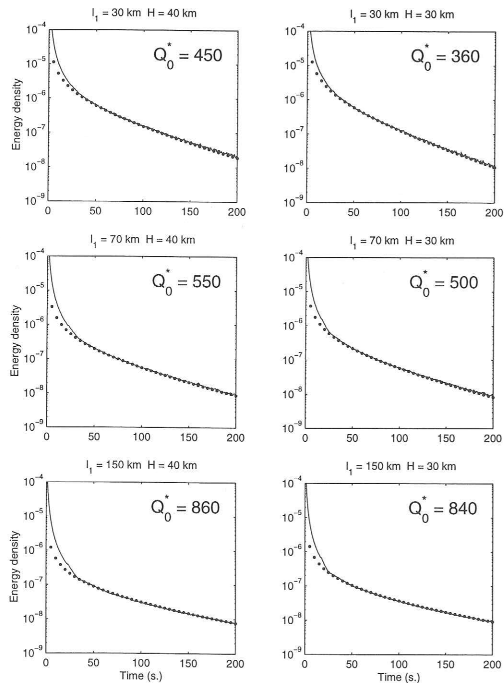
FIG. 2.10 - Coda decay obtained for model 4 with H = 30 km, H = 40 km, and the mean free path of the upper layer l_1 ranging from 30 km to 150 km. Solid lines show the numerical solution of the Radiative Transfer Equation, while broken lines show the best approximation obtained with the formula \frac{1}{t} \exp(-\frac{2\pi t}{Q_0^*}) . The Q_0^* value corresponding to the best approximation is given in the figures. The standard deviation of the Q_0^* is \Delta Q_0^* \approx 15 .
