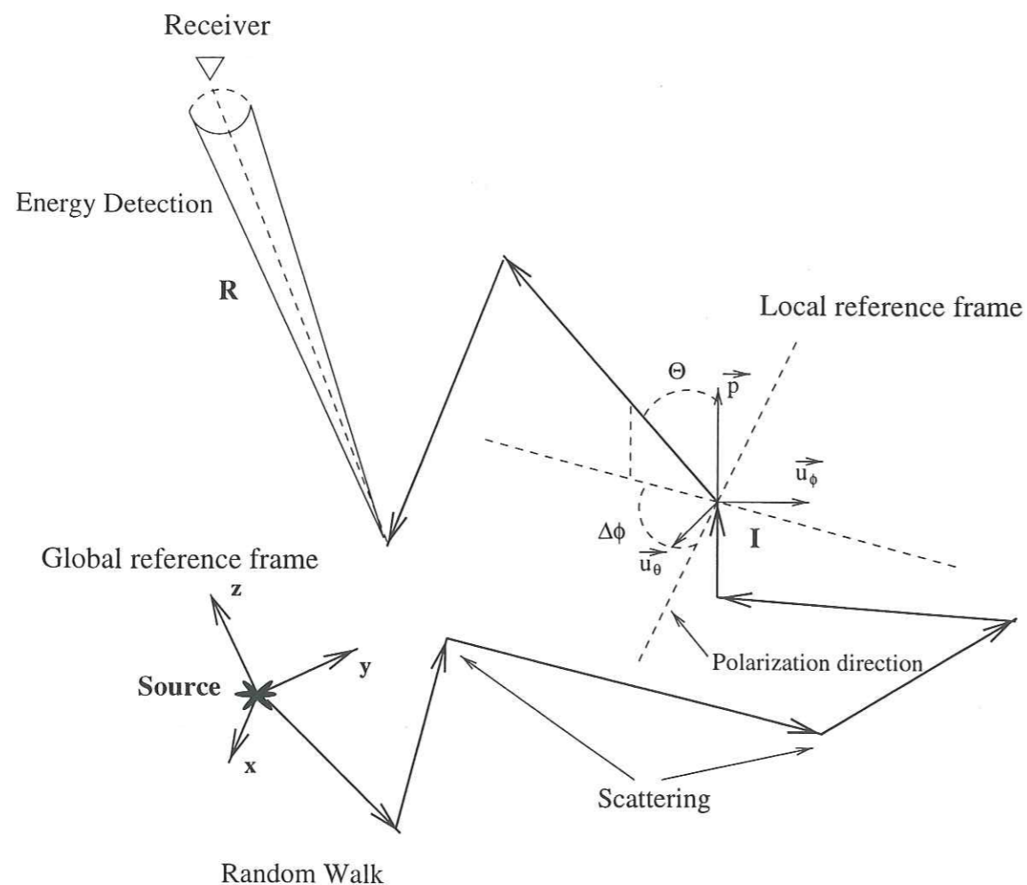
FIG. 4.3 – Schematic picture of the Monte Carlo simulation. The particle starts at a point source and makes a random walk in the medium. At each scattering, the choice of the new mode, propagation direction, path length is made; the energy contribution of the particle is also calculated at the receiver
