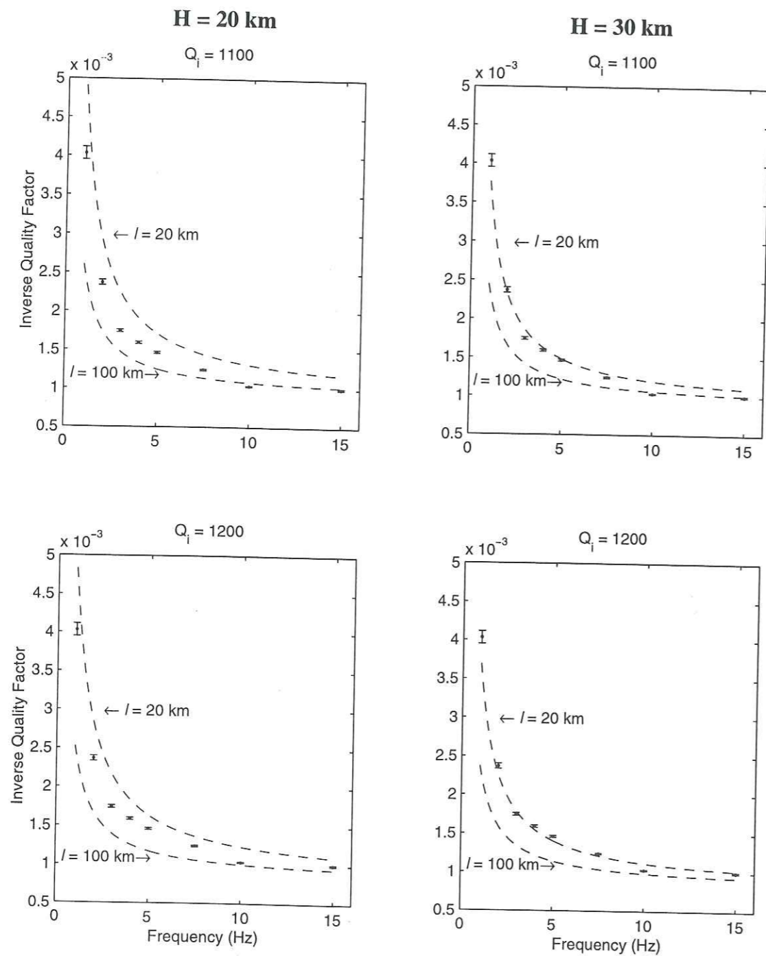
FIG. 3.7 - Same as figure 3.6 except that a constant intrinsic absorption Q_i has been incorporated in the model. The dashed curves limit the domain of 1/Q_m^* predicted by the model for 20 < l < 100 km.
