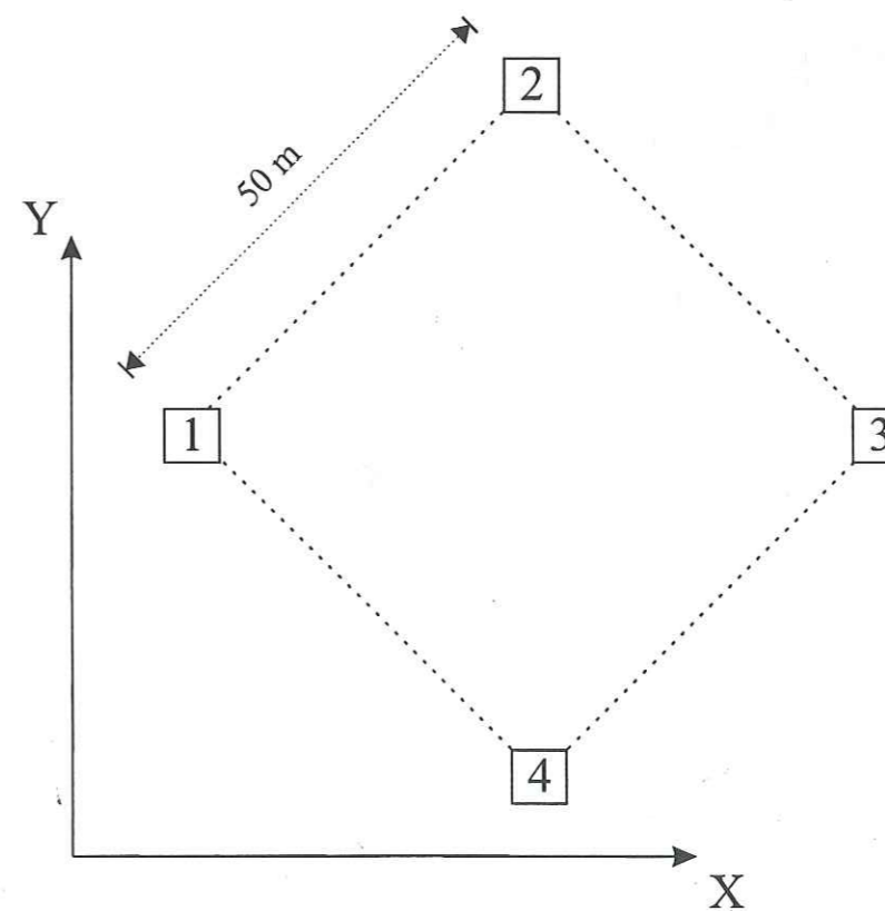
FIG. 5.6 - Configuration of the Chilpancingo array.
