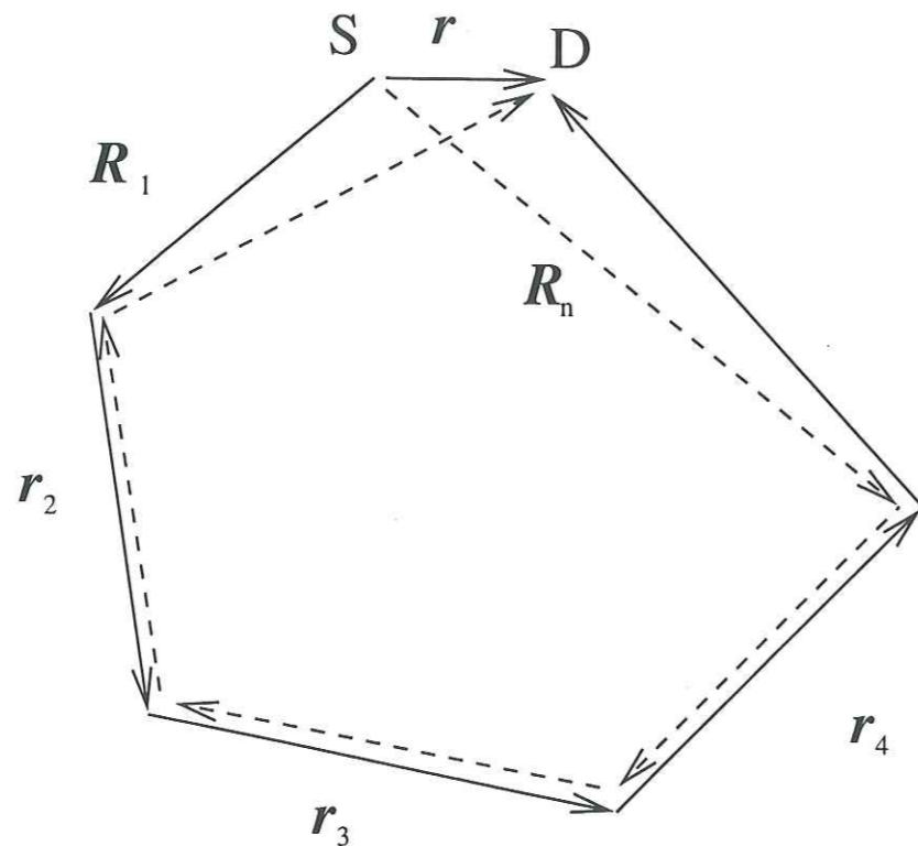
FIG. 6.2 - Geometry for the calculation of the CBS.
