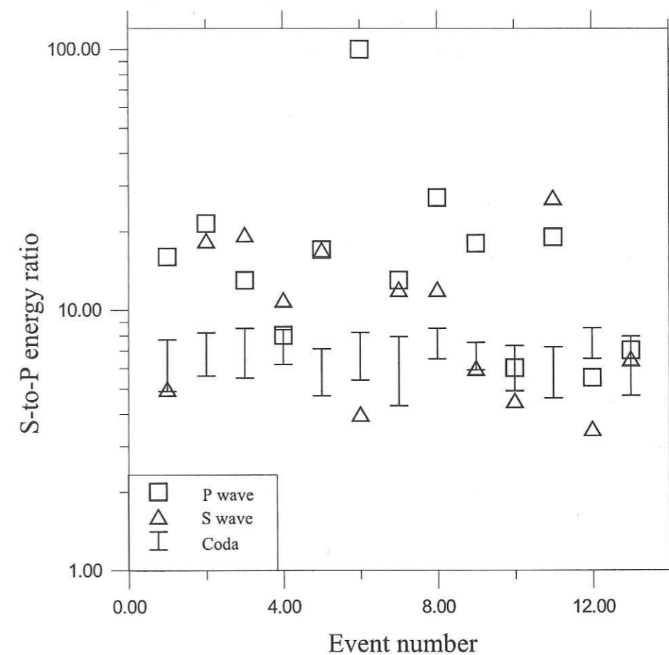
FIG. 5.9 – S-to-P energy ratios for the 13 events. The squares and the triangles indicate the ratios measured for P and S waves, respectively. Vertical bars show average values plus minus standard deviation of the S-to-P energy ratio measured in the coda window.
