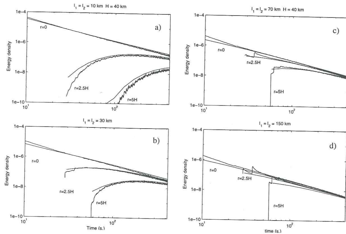
FIG. 2.6 – Comparison of the solutions of the Diffusion and Radiative Transfer Equations for model 2, with a layer thickness H = 40 km. The Radiative Transfer Equation solution curves exhibit characteristic ripples. The mean free path values l_1 (in the upper layer) and l_2 (in the underlying half-space) are indicated on top of each figure. The source is isotropic, point-like, instantaneous and has unit strength. Source and receivers are located just below the free surface. The time origin corresponds to the energy release at source. For each curve the source station distance r is indicated in terms of the upper layer thickness H .
