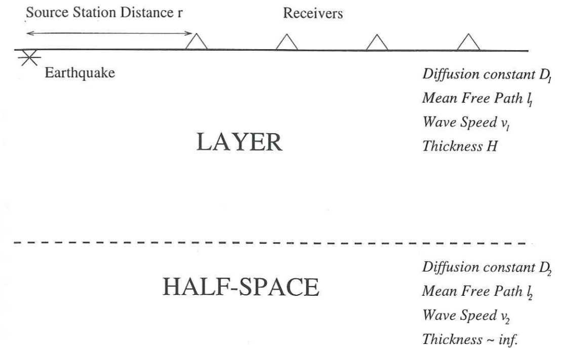
FIG. 2.1 - Geometry and physical parameters of the models. The earthquakes and receivers are supposed to be located just below the free surface. Numerical values of the physical constants can be found in Table I.
