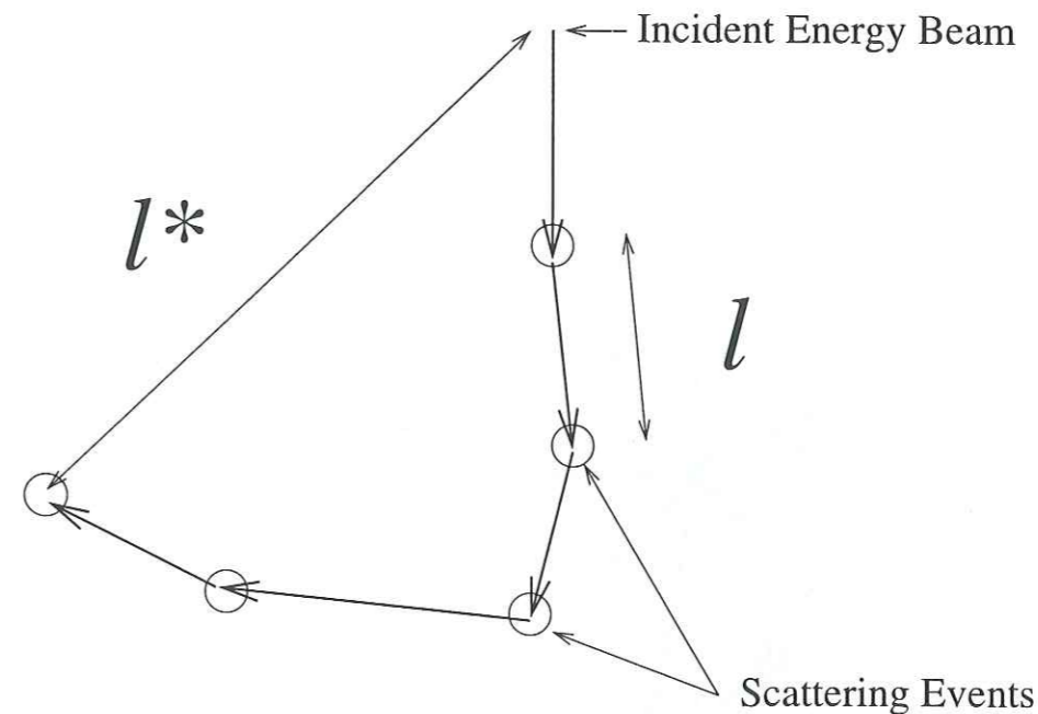
FIG. 2.4 - l is the scattering mean free path of waves. It represents the average distance between two scattering events. l^* is the transport mean free path. It is the length scale necessary for a wave packet to loose memory of its initial direction. In the case of isotropic scattering, both are equal.
