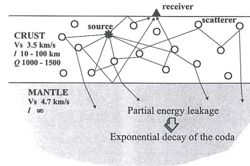
FIG. 5.1 - Sketch of our simplified model with the physical parameters used in the computations.
