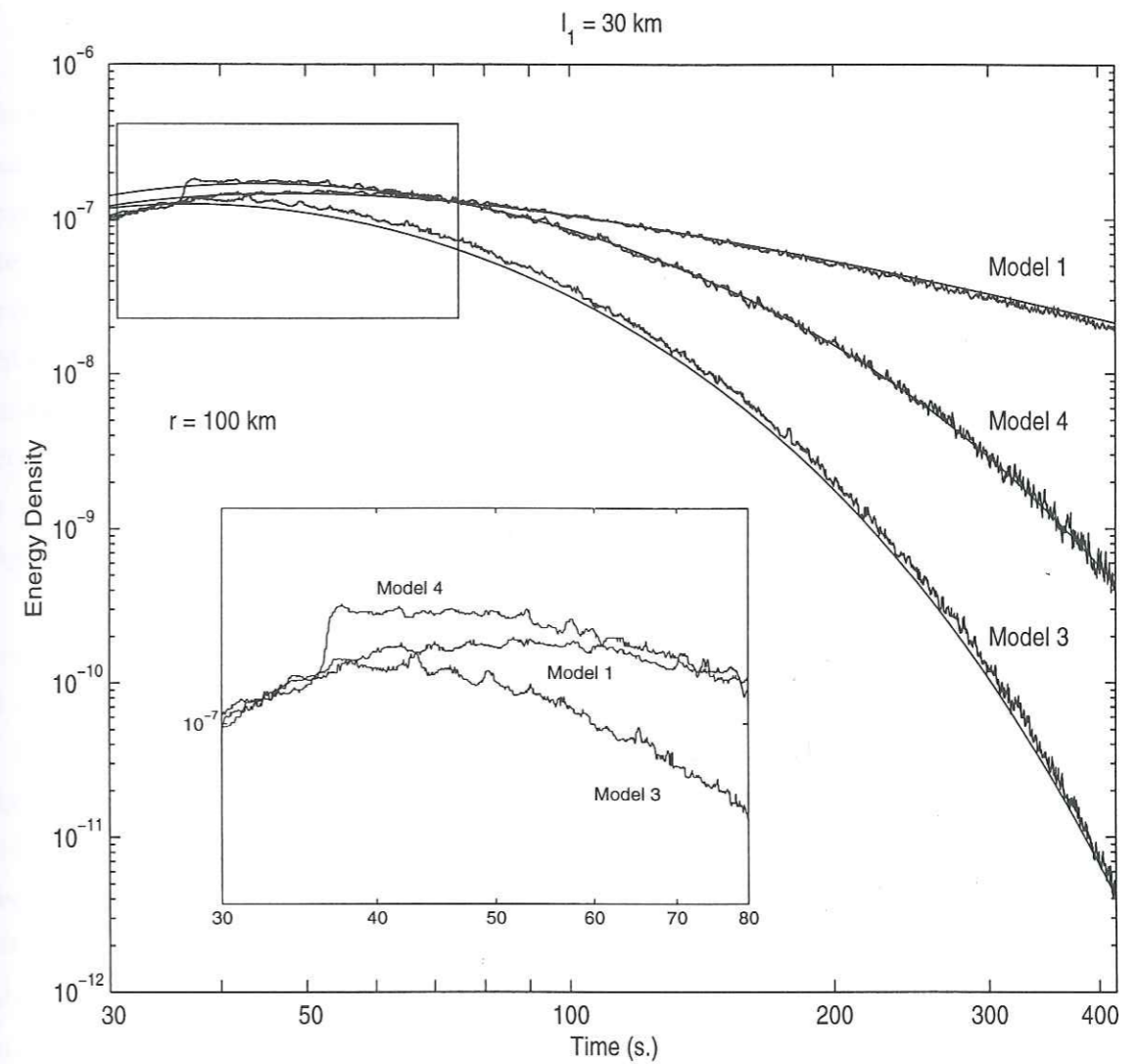
FIG. 2.9 – Comparison of models 1, 3 and 4. The Radiative Transfer and Diffusion Equation solutions are plotted. The Radiative Transfer Equation solution curves exhibit characteristic ripples. For models 3 and 4, the scattering is confined to an upper layer of thickness H = 40 km. In models 1 and 3, the S wave velocity is v_1 = 3.5 km/s, whereas in model 4 a velocity contrast \frac{v_1}{v_2} = \frac{3.5}{4.7} has been added. The source station distance is r = 100 km and the mean free path value is l_1 = 30 km for all models. The time origin is the energy release at source. The beginning of the signals has been magnified in order to distinguish the evolution of the coda for the three models.
