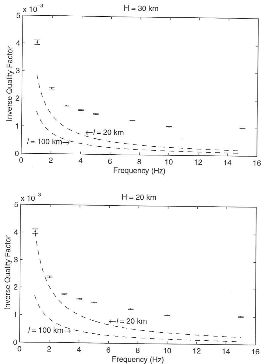
FIG. 3.6 - Dots with error bars show the values of 1/Q_c between 1 and 15 Hz at CAIG. In the same graph, the dashed curves delimit the domain of variation of 1/Q_c^* predicted by the model for the crustal thicknesses H = 20, 30 km, assuming that 20 < l < 100 km in the 1-15 Hz frequency band. Arrows show the value of l for each limiting hyperbola.
