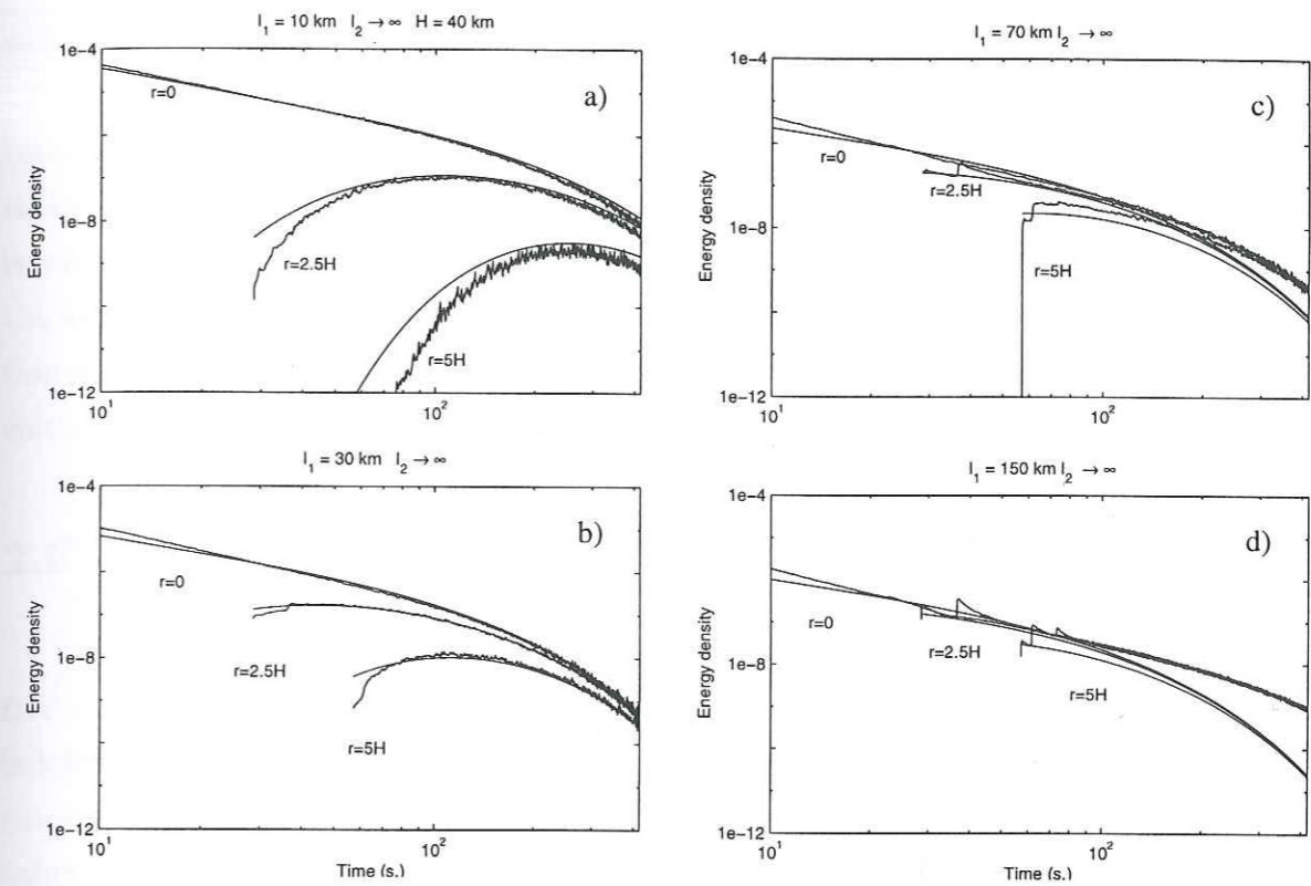
FIG. 2.7 – Same as figure 6 for model 4.
