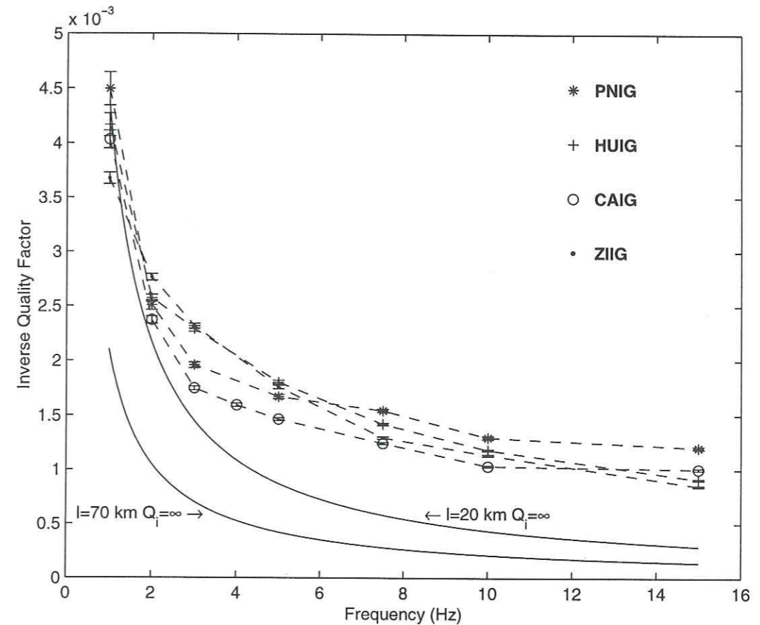
FIG. 5.3 – The symbols correspond to Q_c as a function of frequency measured at the different stations. The continuous lines correspond to the solution of the radiative transfer equation in a purely elastic medium for the extreme values of mean free path 20 km and 70 km.
