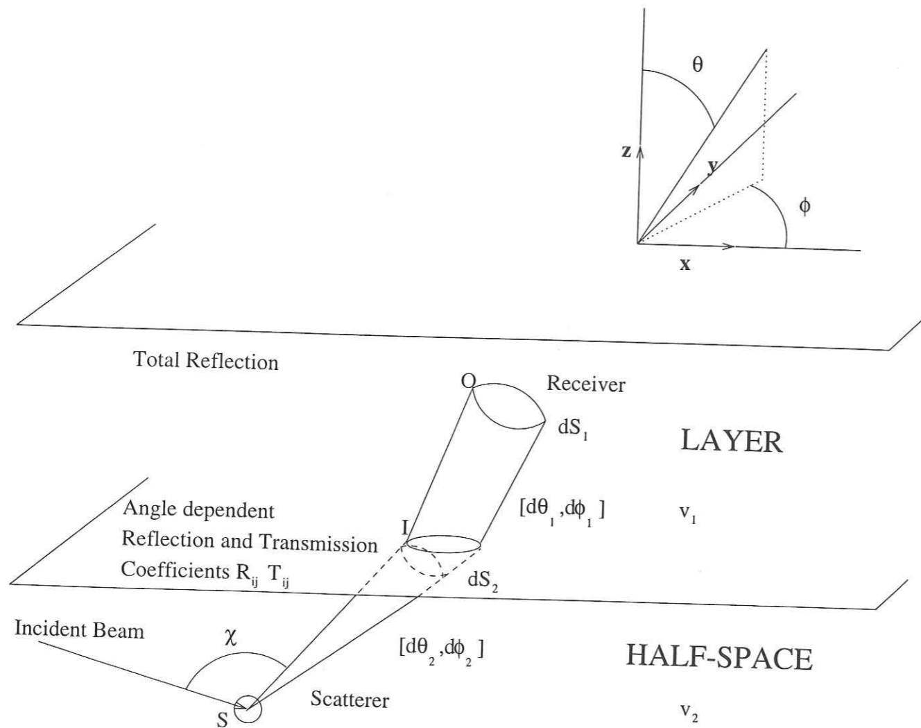
FIG. 2.3 – Transmission of a scattered energy beam at an interface separating two media with different wave speeds. S is the location of the scattering event. I is a point on the intersection surface between scattered beam and interface. O is the location of the detector. \chi denotes the angle between incident and scattered direction. The beam is composed of scattered energy in the solid angle of measure (d\theta_2, d\phi_2) from the point S , where \theta and \phi represent angular spherical coordinates. At the point I , cross section of the beam is dS_2 . Once the beam crosses the interface, the new solid angle is (d\theta_1, d\phi_1) . At the point O , cross section of the beam is dS_1 .
