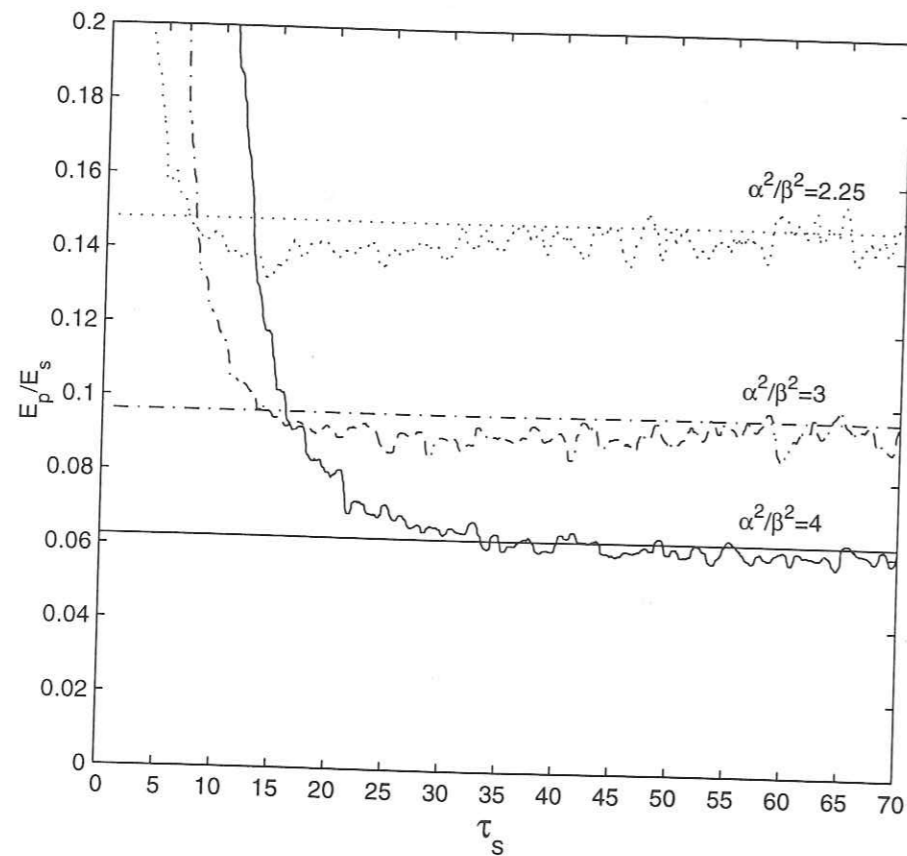
FIG. 4.5 – P to S energy ratio as a function of time for different values of the ratio of wave speeds \alpha/\beta . The Monte Carlo solutions exhibit characteristic ripples. The theoretical asymptotic value of the equilibration ratio is also plotted. Time unit is the mean free time of the shear waves.
