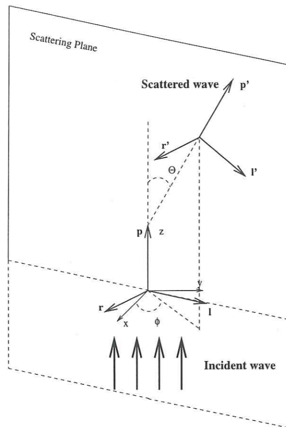
FIG. 4.1 - Sketch of the convention used to derive the scattering matrix.
