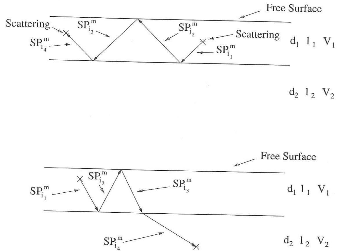
FIG. 2.2 - Determination of the free path between two successive scattering events in the layered medium. The direction of propagation of the particle changes according to Snell's law when it encounters a boundary and is kept constant otherwise. a) The particle remains in the layer, b) it is transmitted in the lower half-space.
