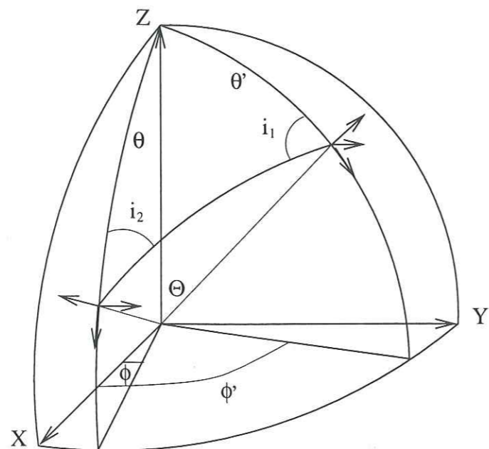
FIG. 4.2 – Sketch of the convention used to derive the Mueller matrix. i_1 denotes the dihedral angle between the incident and scattering planes, while i_2 denotes the dihedral angle between the scattering and outgoing planes. \Theta is the scattering angle.
