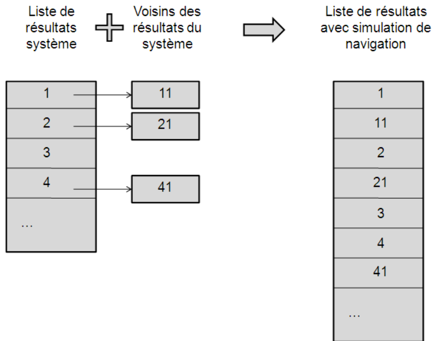
FIG. 8.7 – Simulation de navigation.
