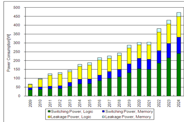
Figure SYSDD11 SOC Consumer Stationary Power Consumption Trends—UPDATED
