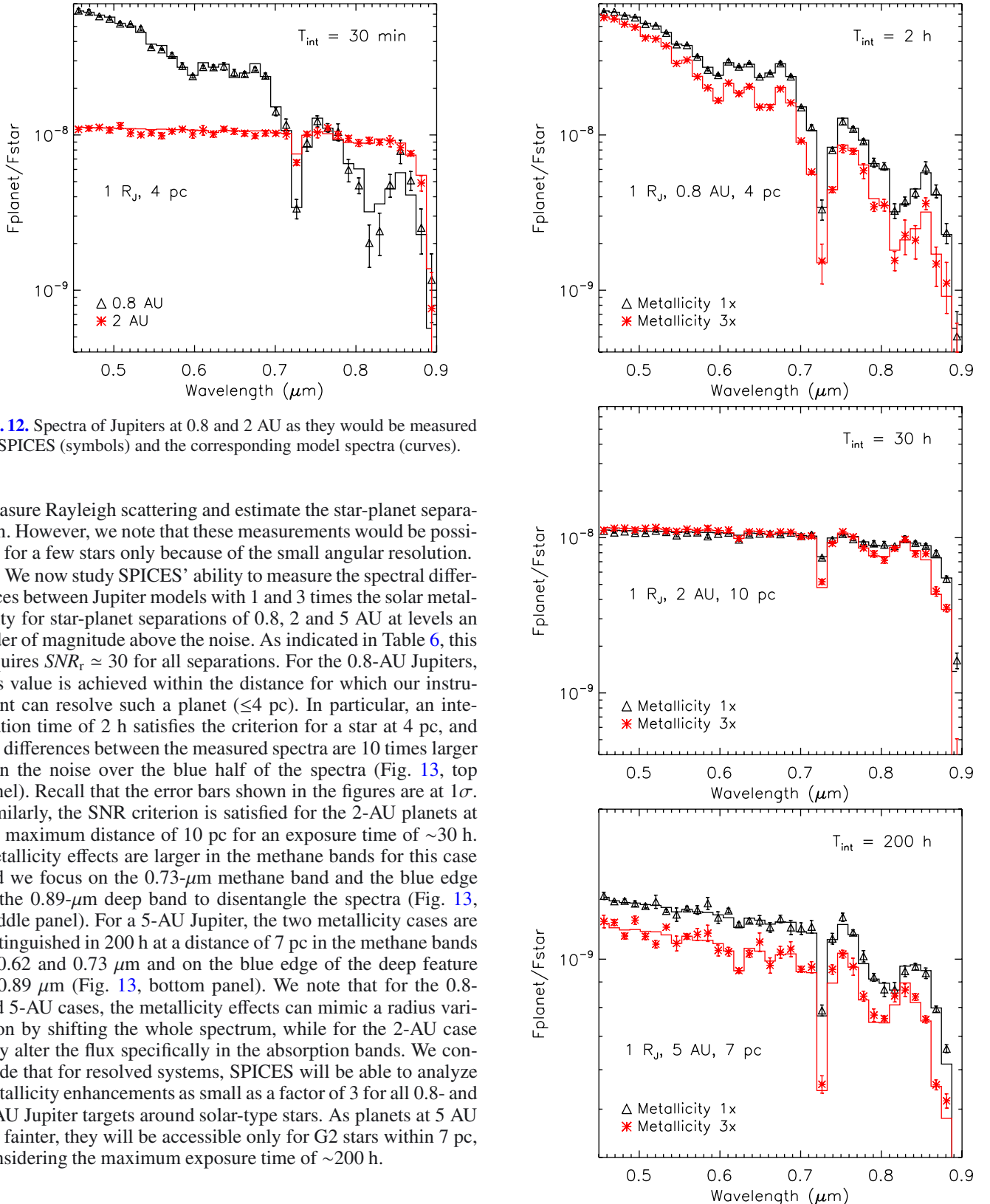
Fig. 13. Measured (symbols) and theoretical (lines) spectra of the 0.8-AU (top), 2-AU (middle) and 5-AU (bottom) Jupiter models for 1 and 3 times the solar metallicity. The planet/star contrast scale is identical to Fig. 12 for comparison except for the bottom panel.
