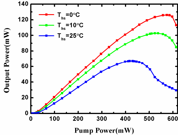
Figure 2.28 CW L-P curves of VECSEL with electroplated copper substrate versus focused pump power for heatsink temperature of 0°C (red), 10°C (green) and 25 °C (blue) in the plane concave cavity with a 99% reflectivity concave mirror (and ROC=15 mm).
