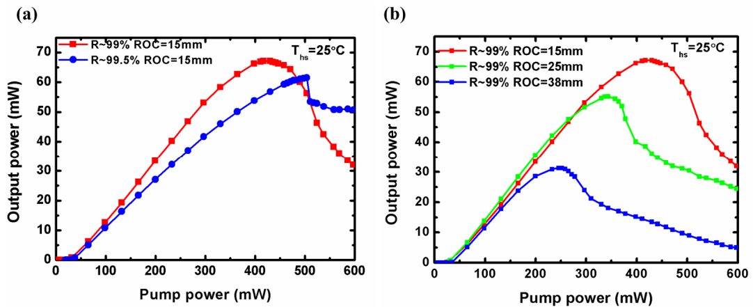
Figure 2.29 CW L-P curve of VECSELs with electroplated copper substrates versus pump power for heatsink temperature of 25°C in the plane concave cavity with (a) different reflectivity: 99% (red square) and 99.5 % (blue circles) of a concave mirror with ROC=15 mm; (b) 99% reflectivity concave mirror of ROC=15mm (red), 25mm (green) and 38mm (blue).
