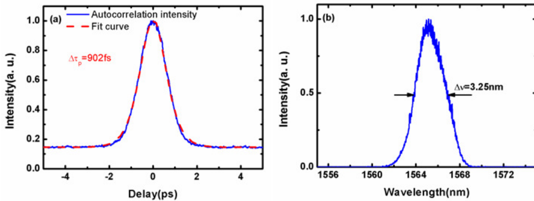
Figure 4.9 (a): Autocorrelation trace of the mode-locked pulse obtained for ACR54-B SESAM. Blue curve: experimental data. Red dash: fit assuming a \text{sech}^2 pulse. (b): Corresponding average optical spectrum.
