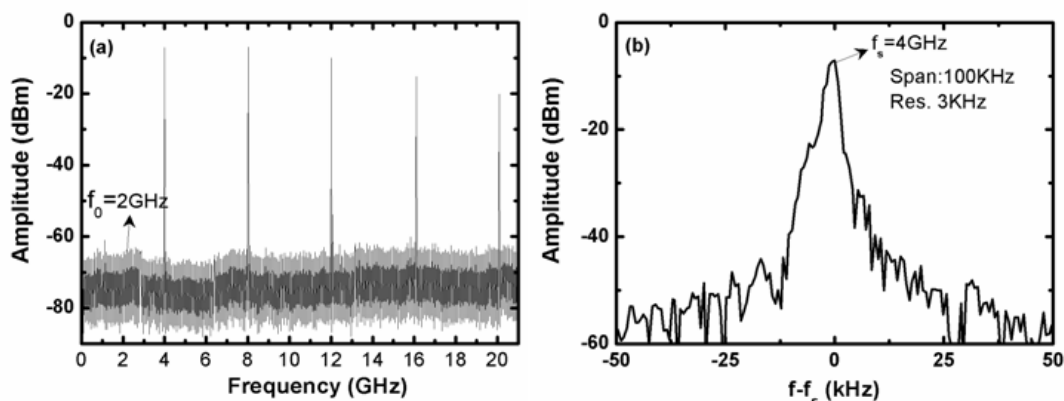
Figure 4.11 Second harmonic mode-locking results. (a) RF spectrum of the mode-locked pulse obtained for ACR54-A SESAM on a 21 GHz span . (b) Fundamental component of RF spectrum, taken at a 100 kHz span and 3 kHz resolution bandwidth
