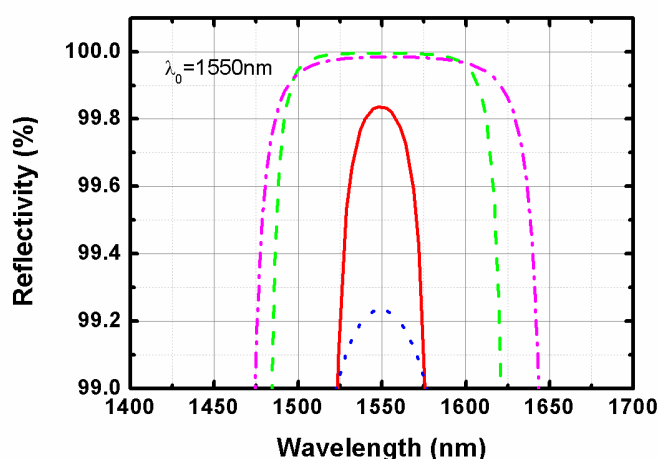
Figure 2.6 Calculated reflectivity of various DBR mirrors at 1550 nm. 48-pair InP/InGaAsP DBR mirror on InP substrate (red solid), 35-pair AlAs/GaAs DBR mirror on GaAs substrate (magenta dash dot), 17-pair AlAs/GaAs DBR mirror on GaAs substrate (blue dot) and hybrid mirror consisting of 17-pair AlAs/GaAs DBR plus a gold mirror (green dash).
