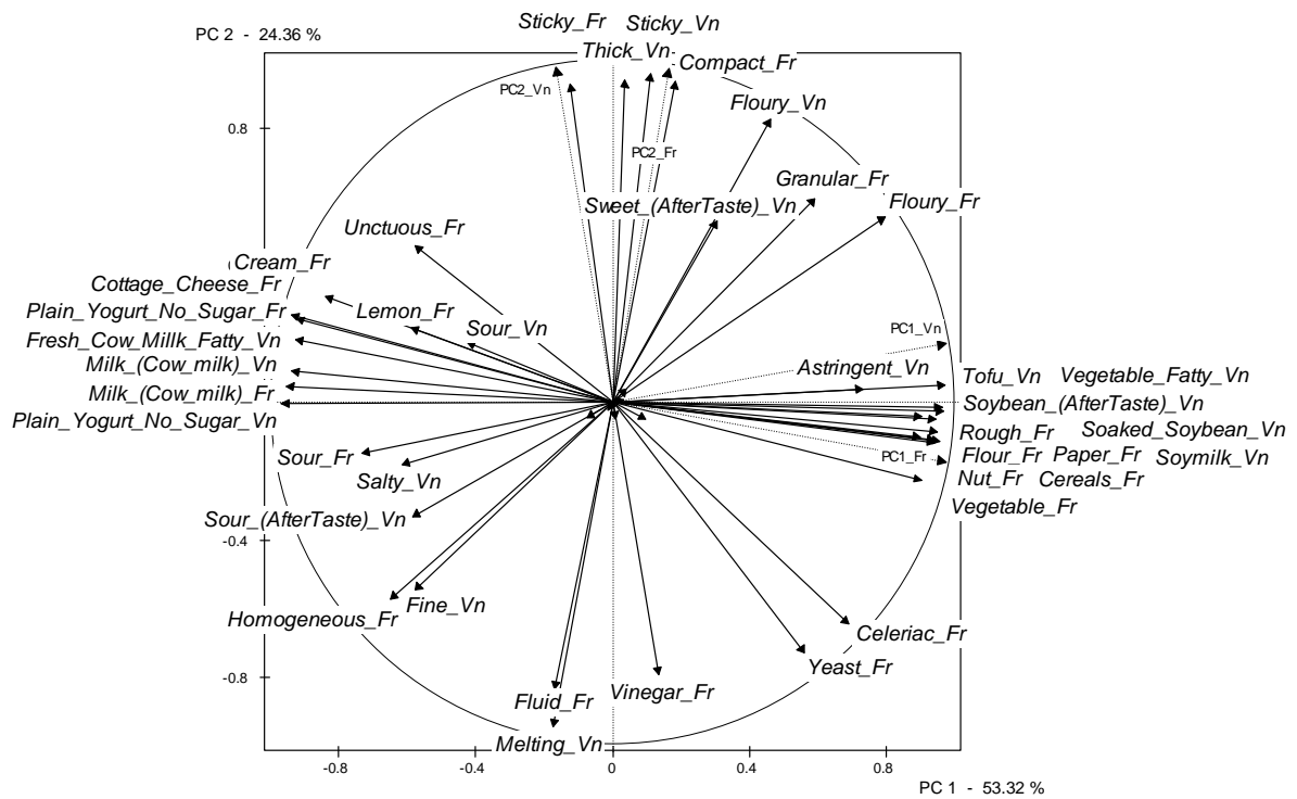
Figure 4. MFA plot – circle of correlation of French (Fr) and Vietnamese (Vn) panel.
