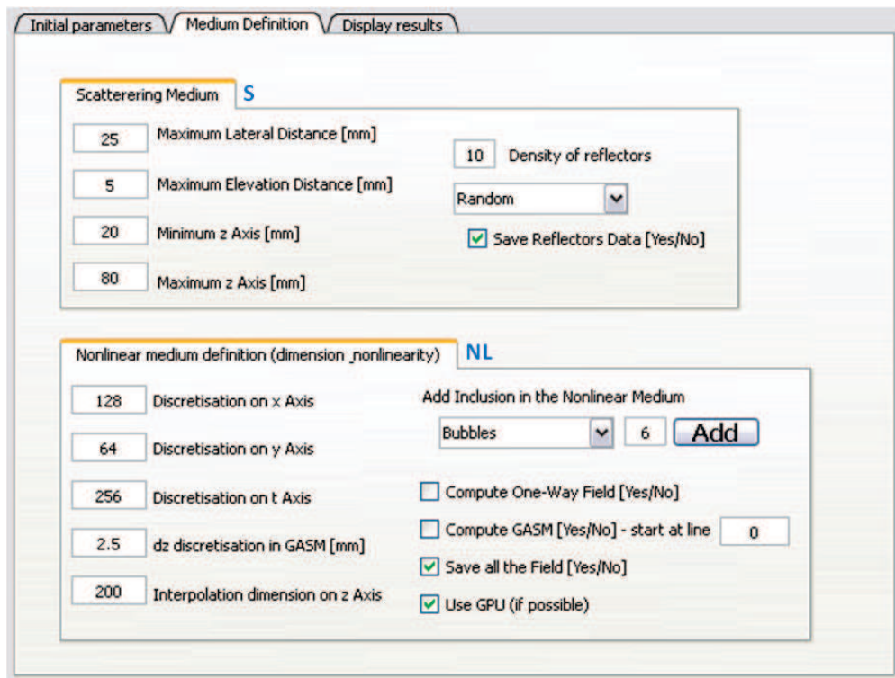
Figure C.3: Illustration of the scatterers definition and the GASM configuration.
