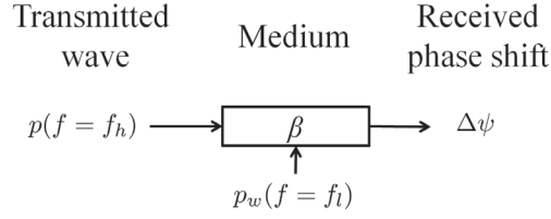
Figure 5.10: Pump wave method: the probe pulse is modified in function of the pump wave and the nonlinear coefficient of the medium.
