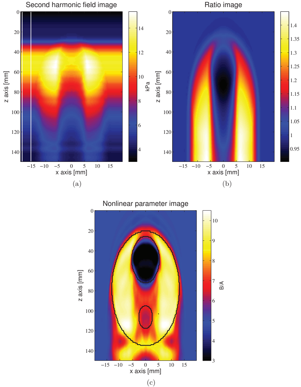
Figure 6.4: Resulting images obtained with the ECM method on the simulated media 2 (Fig. 6.2.b). (a) is the second-harmonic field image produced by GASIM with the region between the two vertical lines considered as the reference medium p_{20} , (b) is the ratio image between p_{2i} and p_{20} and (c) is the final B/A images obtained with the ECM. In (a) the region between the two vertical lines is considered as the reference medium. The solid line in (c) outlines the different regions.
