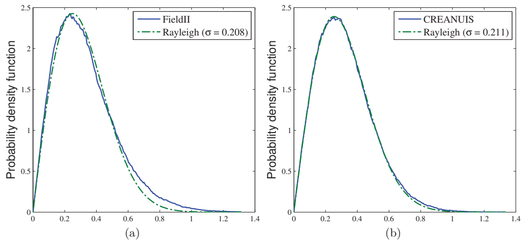
Figure 4.4: Comparison of theoretical Rayleigh probability density function obtained with (a) FieldII and (b) CREANUIS. These two distributions are very similar. The RMSE obtained with CREANUIS is 2.1%, and is smaller than the one obtained with FieldII, 7.7%.
