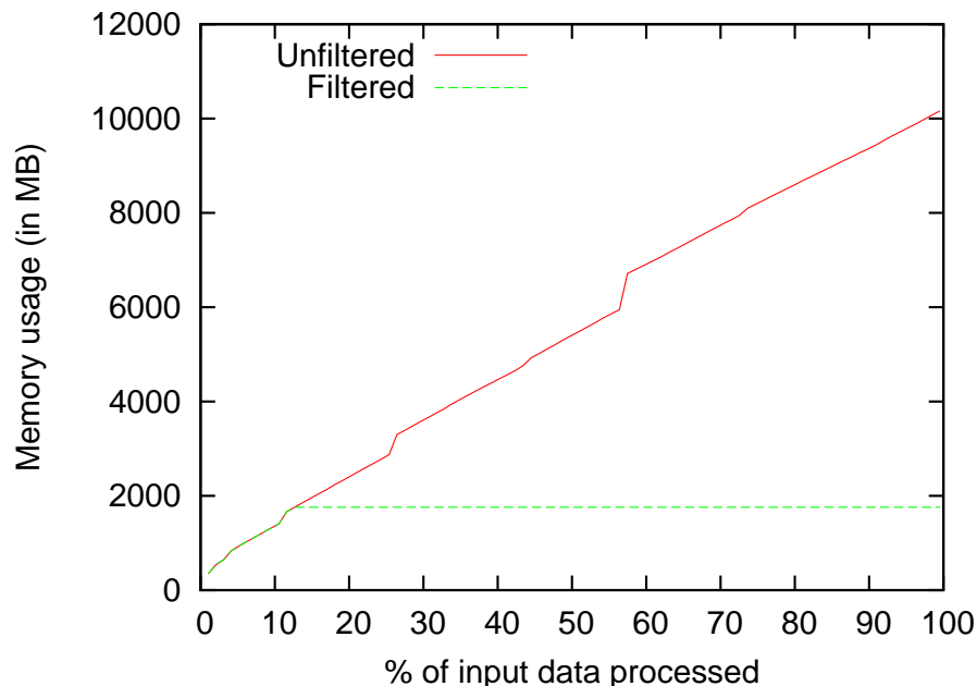
Figure 4-8: Memory usage during the on-line k -mers filtering procedure, compared with un-filtered indexing. Dataset 1 is processed with solidity threshold m_{solid} = 10 , error-detection resolution r = 10 , minimum amount of erroneous k -mers S_{min} = 10^7 and using 1 thread. The first filtering pass is triggered at 11.6% of the dataset. Sporadic jumps in memory consumption correspond to resize operations of the hash table. Figure taken from [9]
