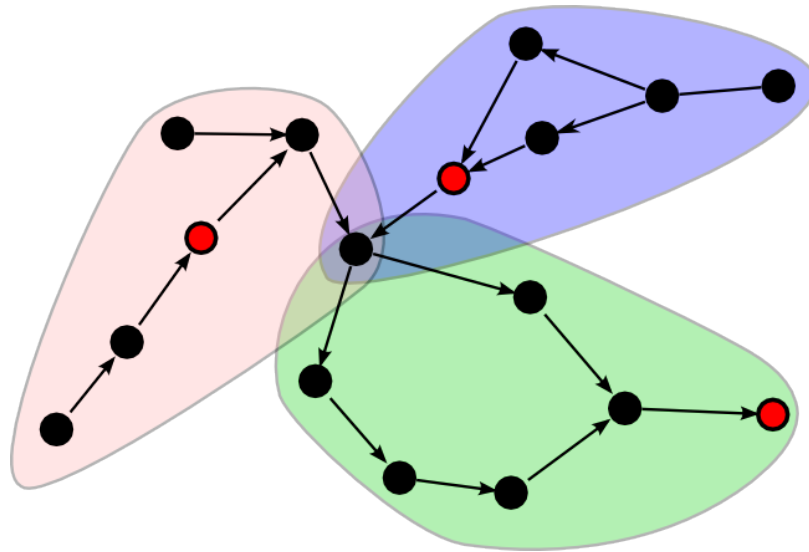
Figure 5-2: Assembly by localized sub-graph construction. Red nodes are starting regions. Each starting region initiates the construction of a sub-graph (clusters of different colors).
