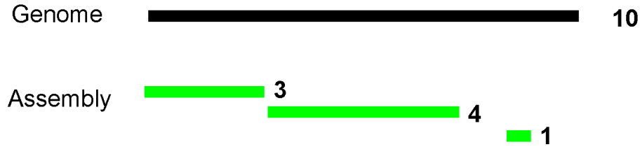
Figure 5-4: Toy example for computing the N50 and NG50 metrics. A genome (black line) is represent along with an assembly (green lines, representing contigs or scaffolds). The number next to the each line specifies a fictional sequence size. The N50 of this assembly is 4, and NG50 is 3.
