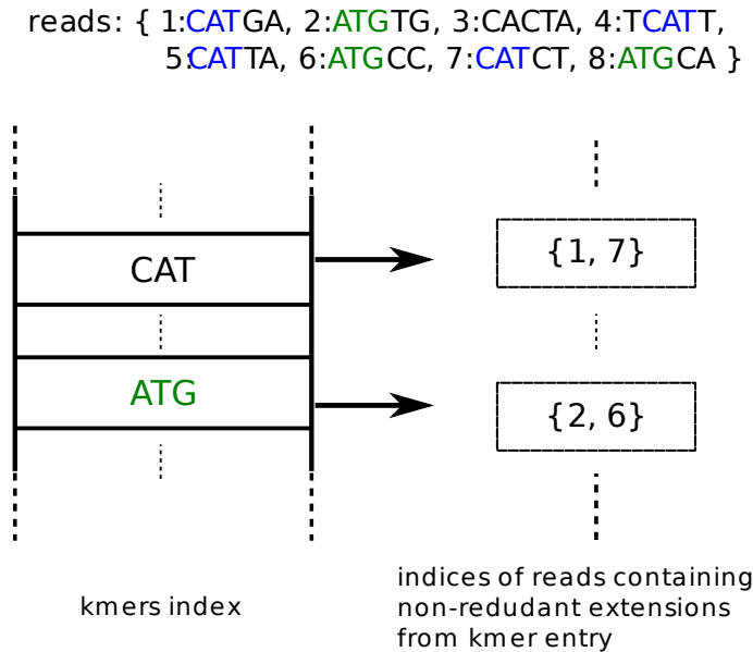
Figure 4-7: The representative reads spectrum for a set of 8 reads with parameters k = 3, t = 1 . Entries are solid k -mers from reads. Each k -mer is associated with a list of reads which extend the k -mer to the right. The extensions are filtered for t -redundancy. For instance, read 4 is not indexed in the CAT entry because the extension T is 1-redundant with respect to extension GA from read 1. In the CAT entry, read 5 could have been inserted instead of read 1 (arbitrary tie removal). Reverse complements of reads are also indexed, but are omitted in this figure.
