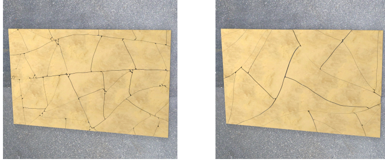
Figure 3.21 – Illustration of the two relaxation methods used. Left: the fracture has a preferred orientation. The stress relaxation of equation (3.16) is used. Right: the pattern does not have a preferred orientation. The stress relaxation of equation (3.17) is used.
