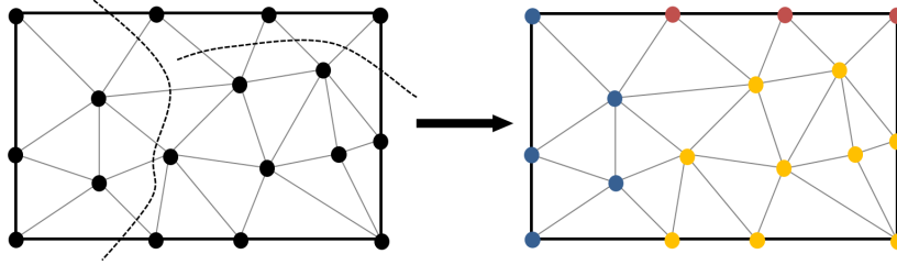
Figure 3.4 – Node fragment identifiers. Each node is associated to the fragment it belongs to. The connected set of nodes that have the same identifier form a fragment. Left: A body is damaged by two cracks represented by the dotted lines. Right: Resulting fragment identifiers on nodes (fragment identifiers are symbolized with colors)
