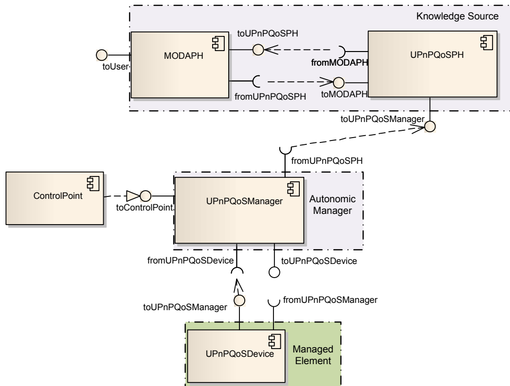
Figure 4.8: Autonomic QoS Management with MODA applied to UPnP QoS
