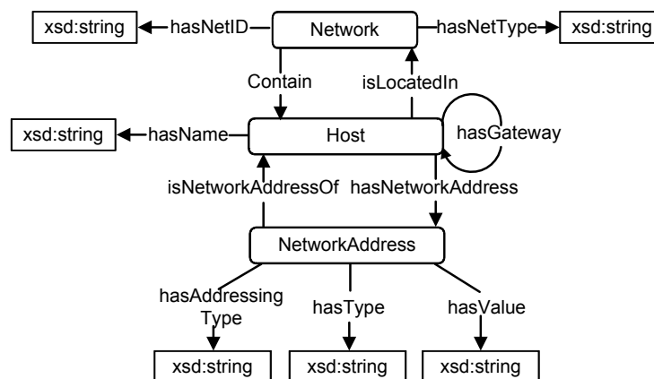
Figure 3.11: Host-Network Ontology.
