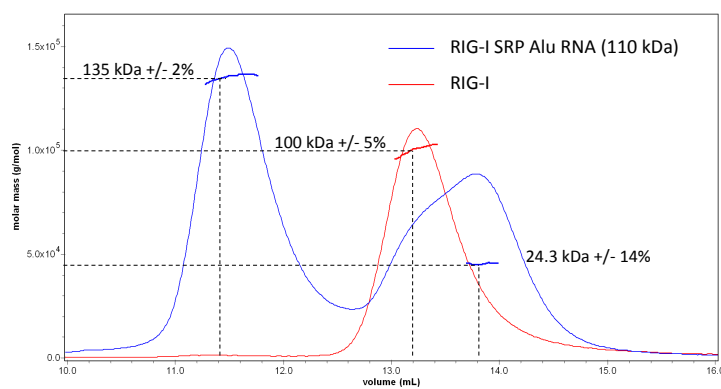
Figure 2.13: SEC-MALLS results of full length RIG-I and Pyrococcus horikoshii SRP Alu RNA.
