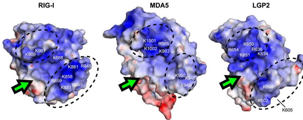
Figure 1.5: The positive charged RNA binding patch on the CTD of RIG-I, MDA5 and LGP2. Positive charges are colored in blue and negative charges in red on the surface representation of the domains [138].
