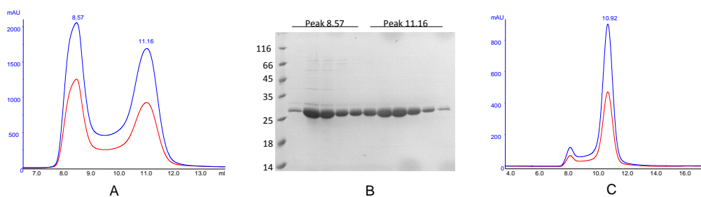
Figure 2.3: Purification of human RIG-I CARDs (residues 1-208) (A) Size exclusion chromatography profile on S75/10/300 column. The peak at 8.5 ml elution volume represents aggregated protein. The peak at 11.16 ml represents the monomeric CARDs. (B) The corresponding peak fractions on an SDS gel. (C) Re-inject of the concentrated fractions of the non-aggregate peak on the S75/10/300 column. CARDs stay mostly monomeric after concentration.
