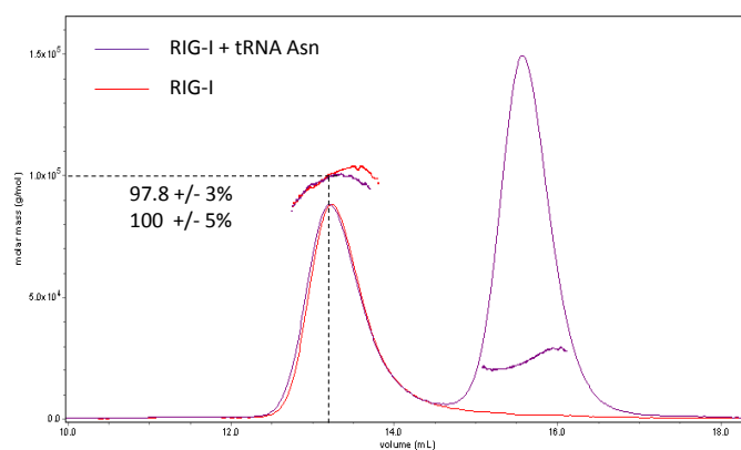
Figure 2.14: SEC-MALLS results of full length RIG-I and Candida albicans tRNA Asn RNA.
