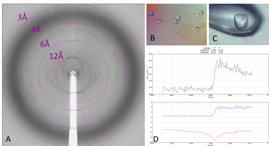
Figure 2.34: Preliminary results of crystallization of RIG-I from Anas platyrhynchos (A) Diffraction pattern. (B) Crystal drop. (C) Mounted crystal. (D) Absorption spectrum for Zn.
