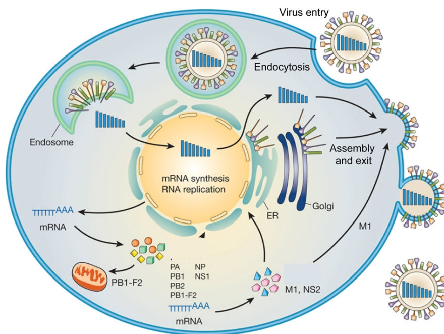
Figure 1.12: The replication cycle of the influenza virus [3]
