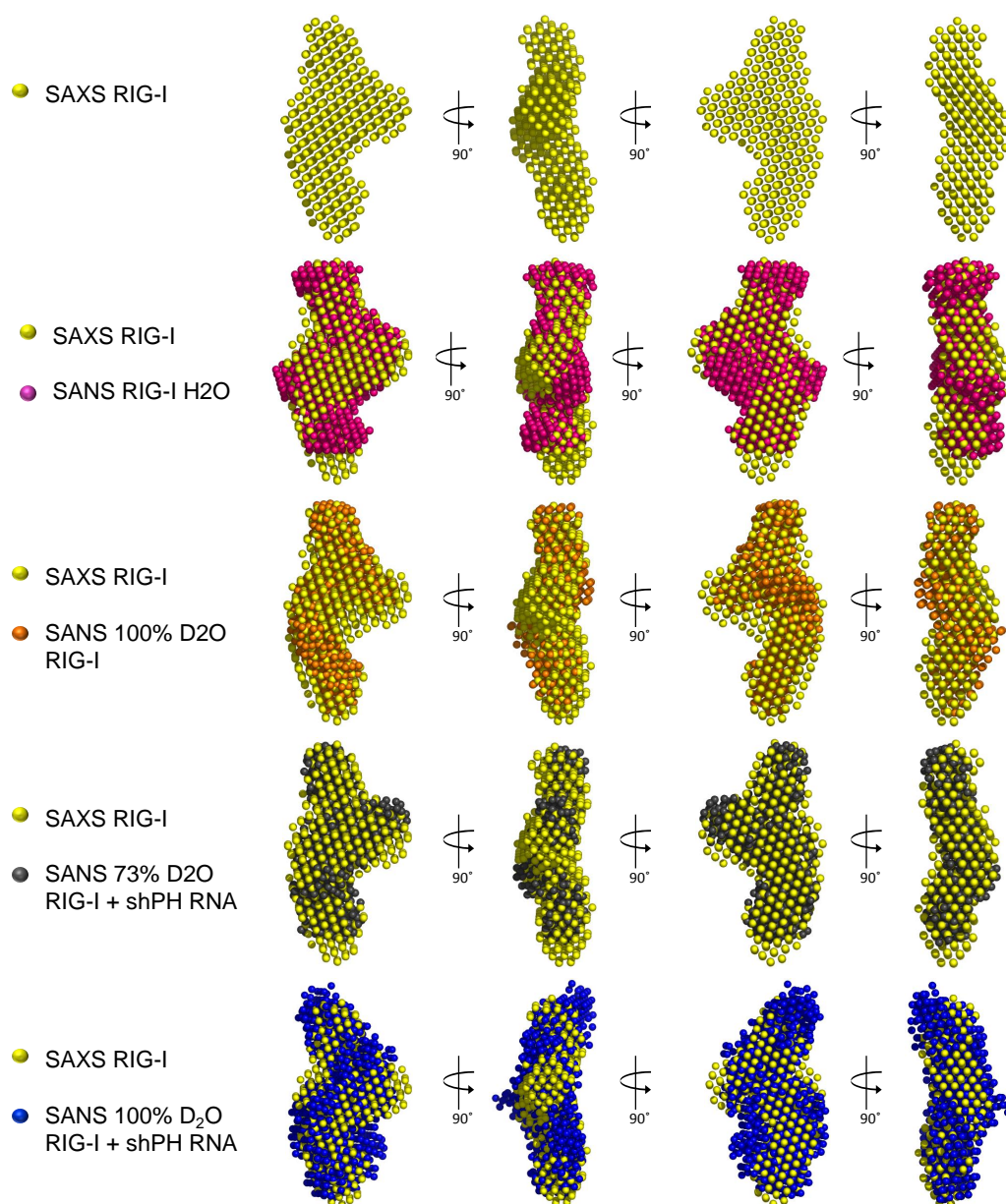
Figure 2.25: SANS models of RIG-I.
