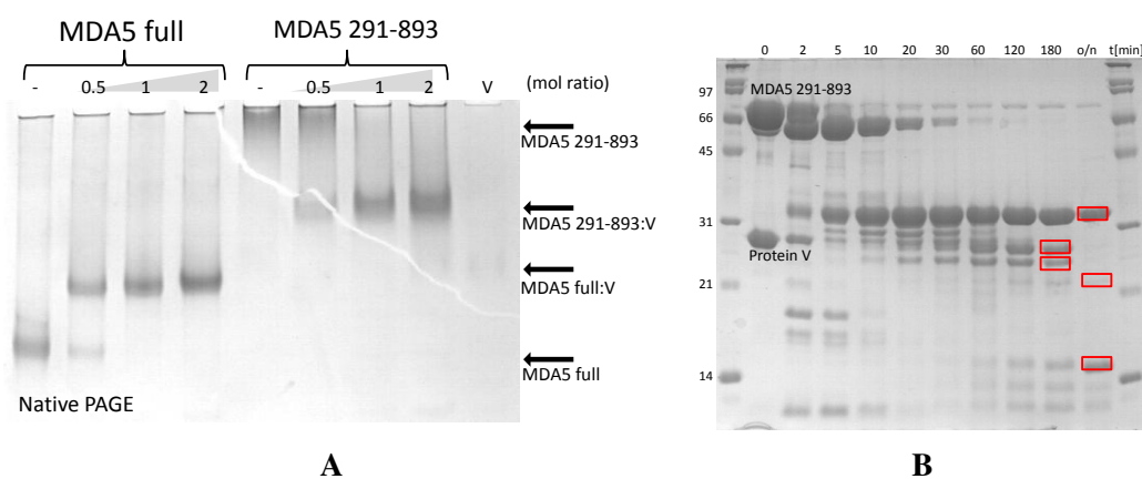
Figure 2.46: (A) Native PAGE of MDA5 (full length and a construct comprising only the helicase domain 291-893) and parainfluenza virus V protein. (B) Results from a trypsination experiment of MDA5-V complex. Bands in red boxes were analyzed by mass spectrometry and appeared to be fragments of MDA5.
