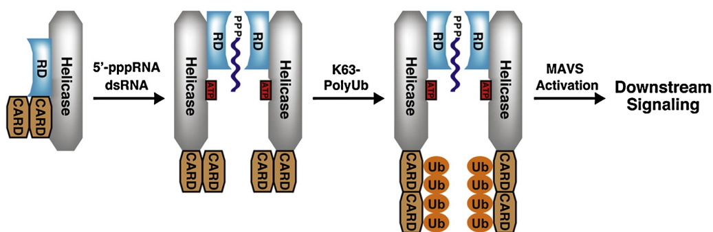
Figure 1.7: Proposed activation mechanism of RIG-I by Zeng et al. [157]
