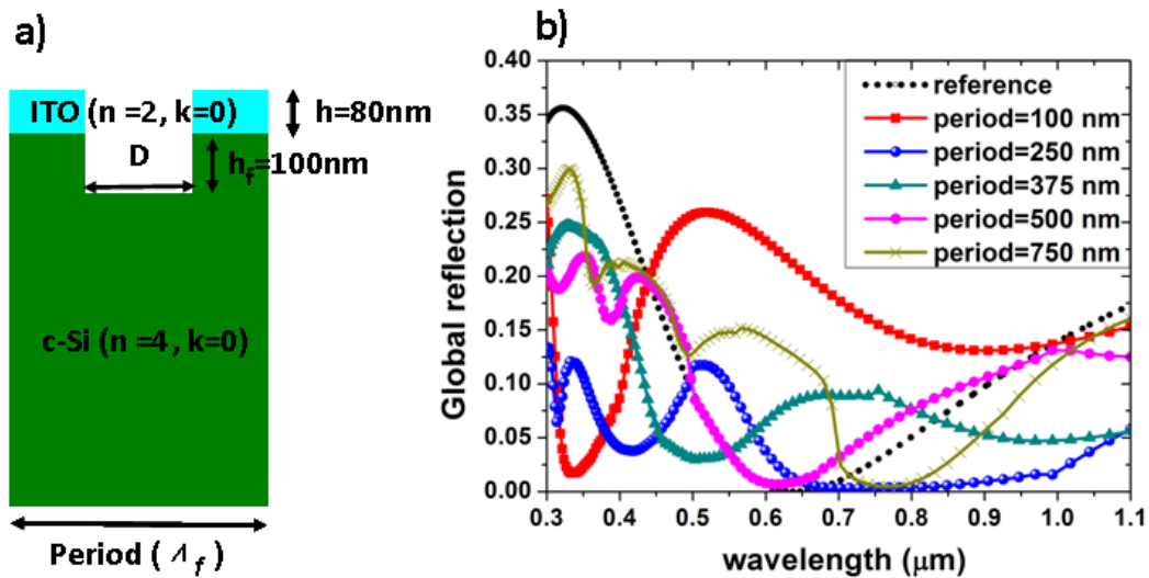
Fig. 6.4. Schematic view of the front grating (a), and reflected intensity versus the wavelength, for various grating periods and considering a TM polarization, and a 50% ffair; the reference corresponds to a planar Si surface covered by a 80nm thick ITO layer (b).
