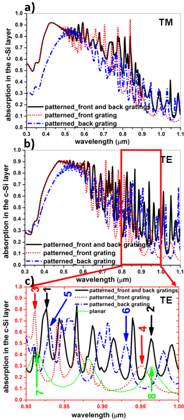
Fig. 6.5. Absorption spectra of the c-Si layer for the front grating, the back grating and the double grating optimized structures, for (a) TM and (b) TE polarized incident light, (c) with a close-up of the spectra for TE polarized light between 800 and 1000 nm.
