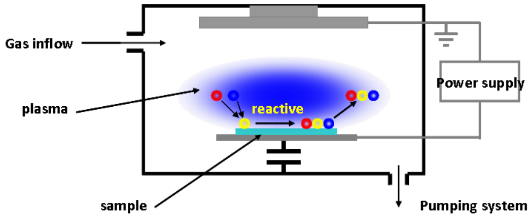
Fig. 3.6. Schematic of RIE and ICP etching system
