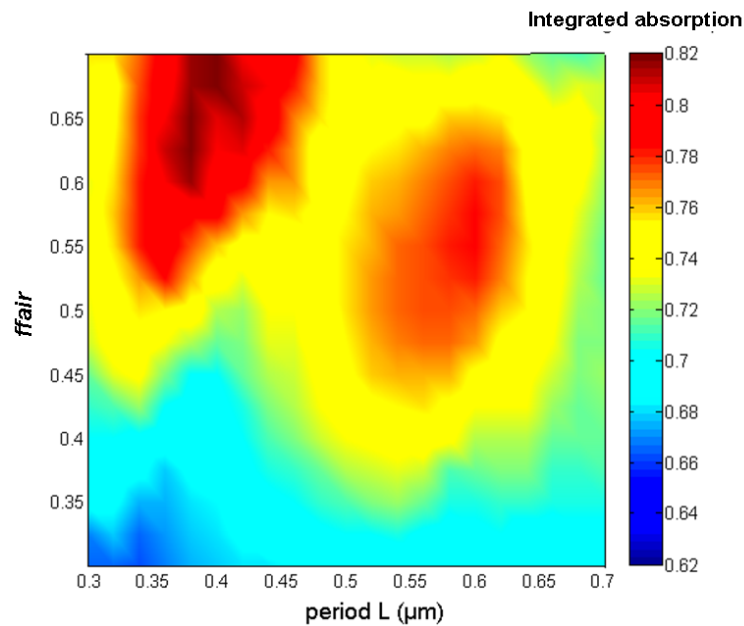
Fig. 4.2. Integrated absorption in the whole patterned cell in function of the period L (x-axis, in \mu\text{m} ) and the ffair ratio (y-axis) of the PC membrane
