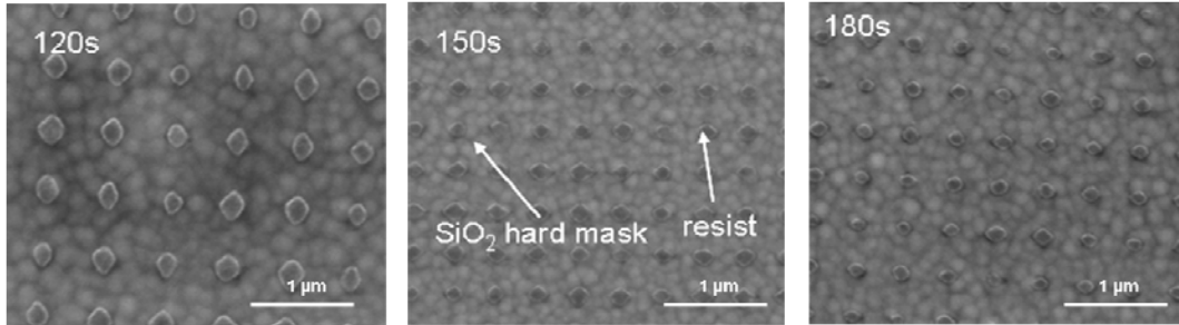
Fig. 4.5. SEM images of the patterned photoresist for different PAB times
