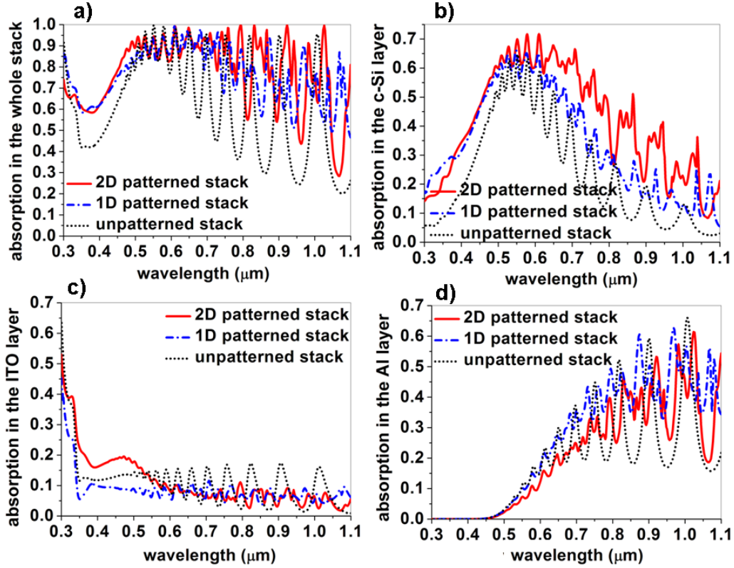
Fig. 5.10. Average absorption spectra on both TE and TM polarizations in (a) the whole stack, (b) the sole c-Si layer, (c) the ITO and (d) the Al layer for the 1D and 2D PC patterned stacks ( L , f_{fair} and h set to 0.61 \mu\text{m} , 35\% and 0.14 \mu\text{m} respectively) obtained by simulation
