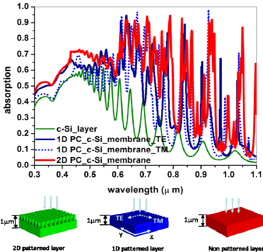
Fig. 5.3. Simulated absorption spectra of the patterned 2D and 1D PC patterned c-Si layer with the same period, f_{fair} and etching depth ( L = 0.61 \mu\text{m} , f_{fair} = 35\% and h = 0.14 \mu\text{m} ) compared to the one of a planar c-Si layer of the same thickness ( 1 \mu\text{m} ).
