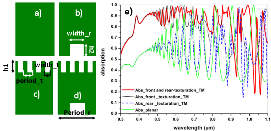
Fig. 6.1. (a) Planar (b) back patterned (c) front patterned and (d) front and back patterned configurations on a 1 \mu\text{m} thick c-Si layer (e) Optical absorption spectra comparison of those 4 configurations, based on TM polarization
