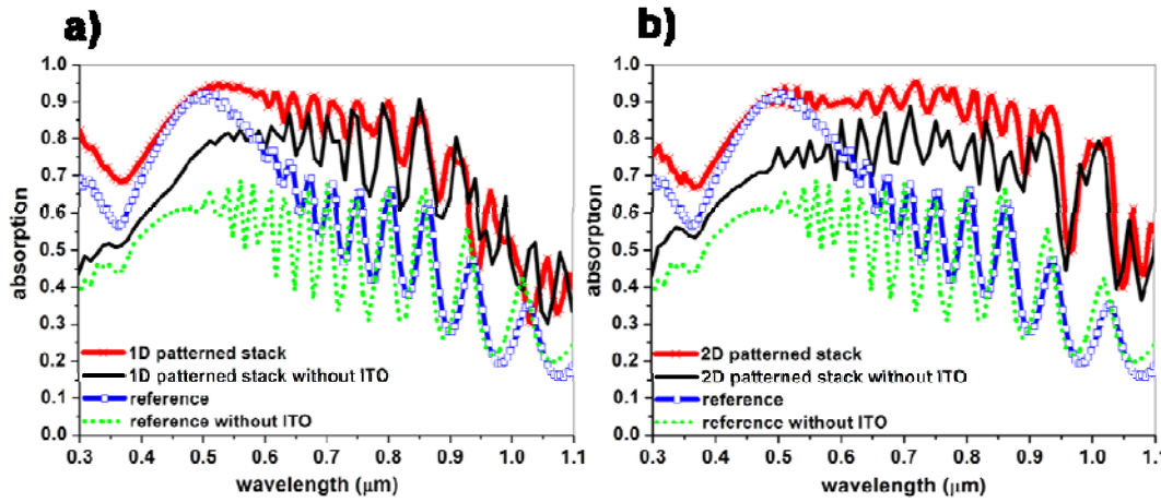
Fig. 5.15. The measured absorption spectra comparison between the (a) 1D and (b) 2D patterned and the unpatterned stacks with and without front ITO layer
