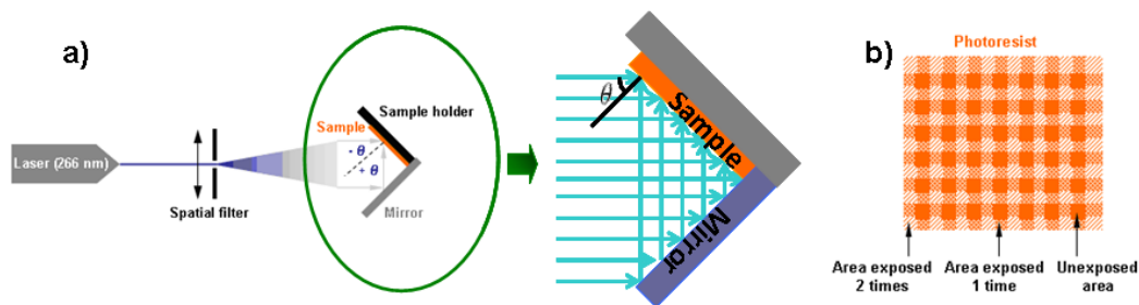
Fig. 4.4. (a) Out of the spatial filter, the beams either impinge directly on the sample's surface or are reflected by the mirror, leading to interference fringes in the photoresist. After a 90 ° tilt of the sample, (b) the second exposure enables to create a square array of unexposed areas
