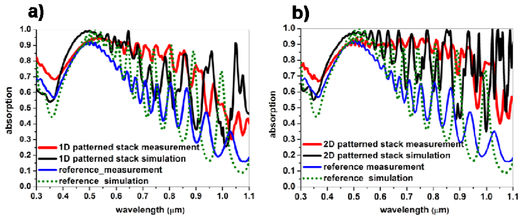
Fig. 5.14. The simulated and the measured integrated absorption spectra comparison of the (a) 1D and (b) 2D patterned stack to the measured and simulated unpatterned stack
