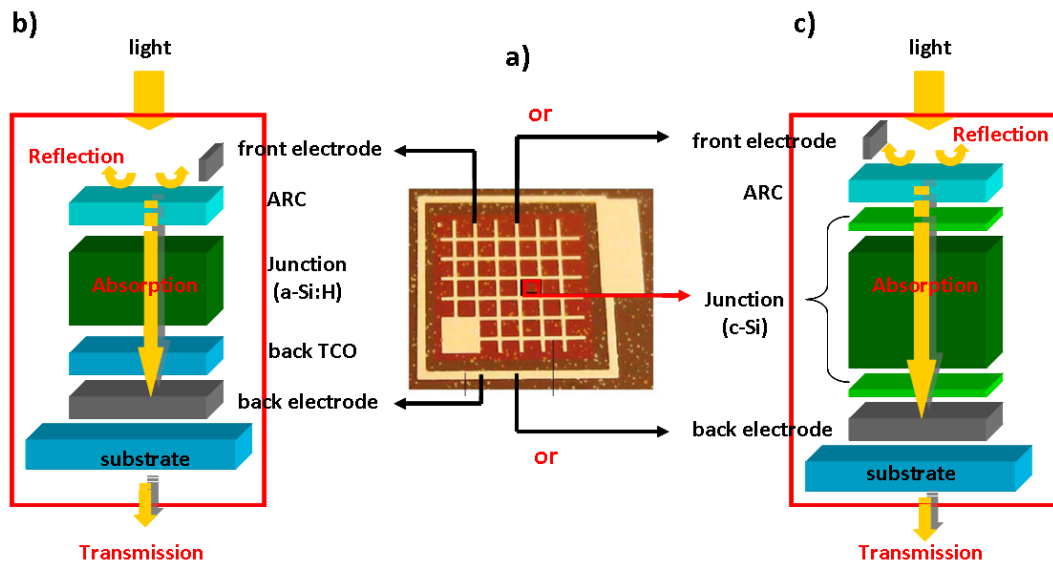
Fig. 2.2. A typical solar cell device (a), a typical a-Si:H thin film solar cell is shown in (b) and a classical c-Si solar cell is described in (c).
