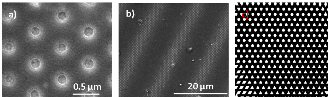
Fig. 4.16. SEM images of the triple exposure on the resist for triangular lattice with (a) correct parameters (b) wrong rotating angle ( -62^\circ , 0 , 60^\circ ), and (c) schematic view corresponding to (b).
