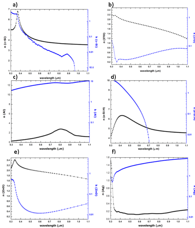
Fig. A. Refractive index n and extinction coefficient k of ITO [from ellipsometric measurement], a-Si:H [from ellipsometric measurement] (above 0.7 \mu\text{m} , k=0 ), c-Si [from ellipsometric measurement] (above 1 \mu\text{m} , k=0 ), ZnO [from ellipsometric measurement], Ag, and Al ① (between 300 \text{ nm} and 1100 \text{ nm} ) used for optical simulations
