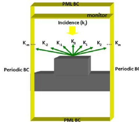
Fig. 3.4. Reflection diffraction grating orders of 1D grating structure
