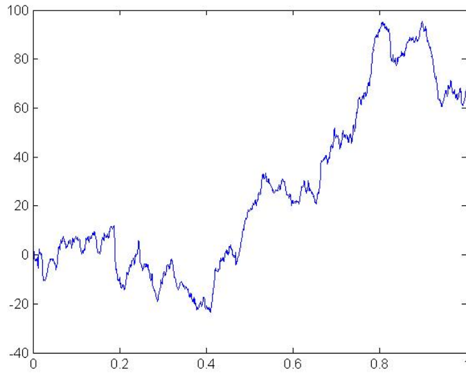
FIGURE 1. Simulation of a path of the process Y_1 when \alpha = 1.8 and H(t) = 0.7 for all t \in [0, 1] .
