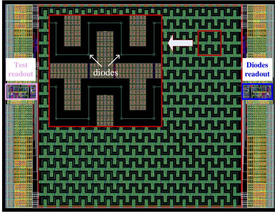
Figure 4.14: Layout of the AlphaRad-2 chip.
