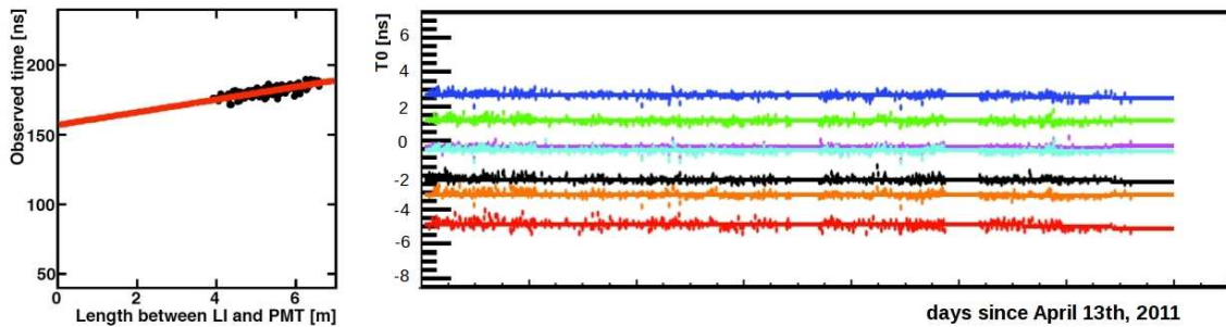
Figure 4.5: (left) Observed time as a function of the length between an LED and opposite PMTs [9]. (right) Time offsets stability over a hundred days for seven channels [9].
