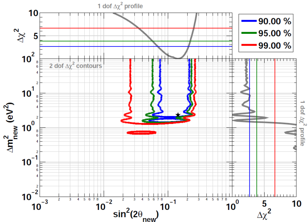
Figure 2.11: Allowed regions projected in the (\sin^2 2\theta_{\text{new}}, \Delta m_{\text{new}}^2) plane from the combination of reactor neutrino experiment, Gallex and SAGE calibration source experiments, MiniBooNE reanalysis of [100], and ILL-energy spectrum distortion [141].
