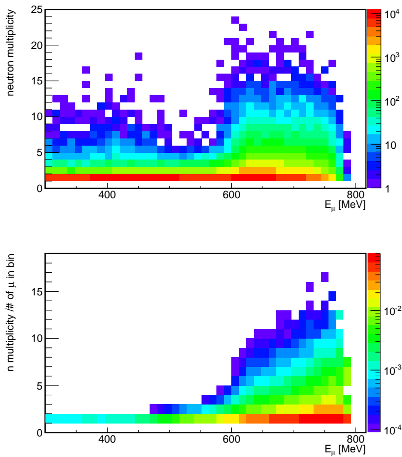
Figure 6.56: (top) Neutron multiplicity as a function of the deposited energy in the inner detector. (bottom) Neutron multiplicity scaled to the number of \mu per energy bin (cf. Figure 6.55).
