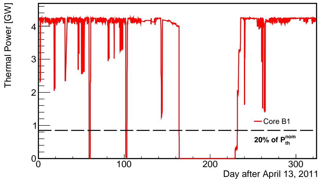
Figure 7.2: Thermal power evolution for reactor B1, per day since April 13 th 2011, in GW. The black dashed line represents 20 % of the nominal thermal power.
