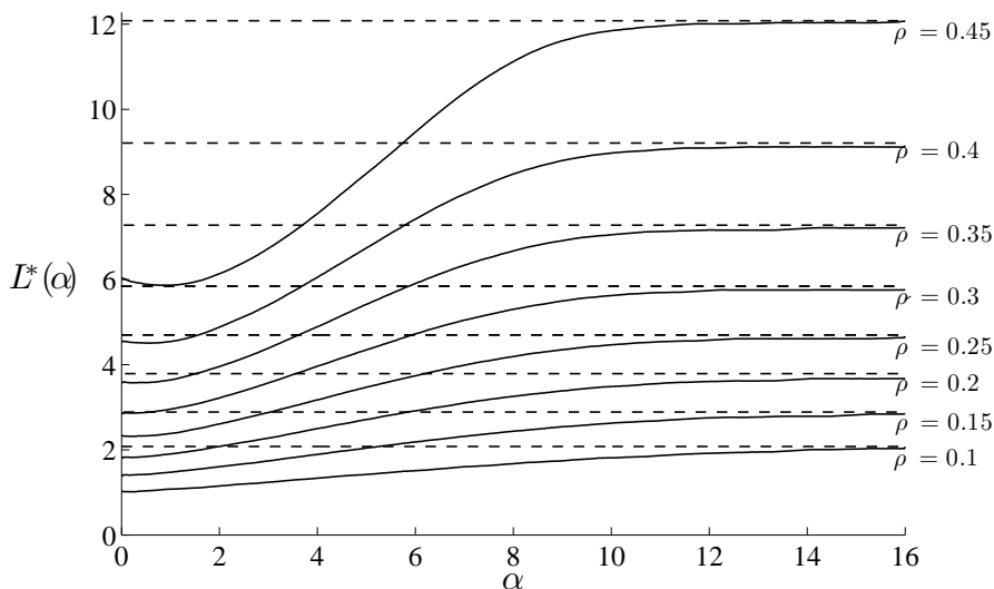
FIGURE 3.4 – Value of the critical threshold L^*(\alpha) in terms of the distance \alpha and the Allee threshold \rho . For each value of \rho , the dotted line corresponds to the associated value of 2L^*(0) .
