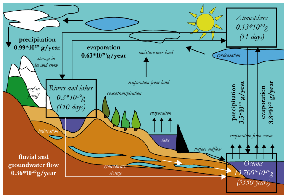
Figure 1.2.2: Hydrological cycle, residence times and matter flux between reservoirs (modified from Drever 1988 [33]); numbers are from Garrels & Mackenzie 1971 [31].
