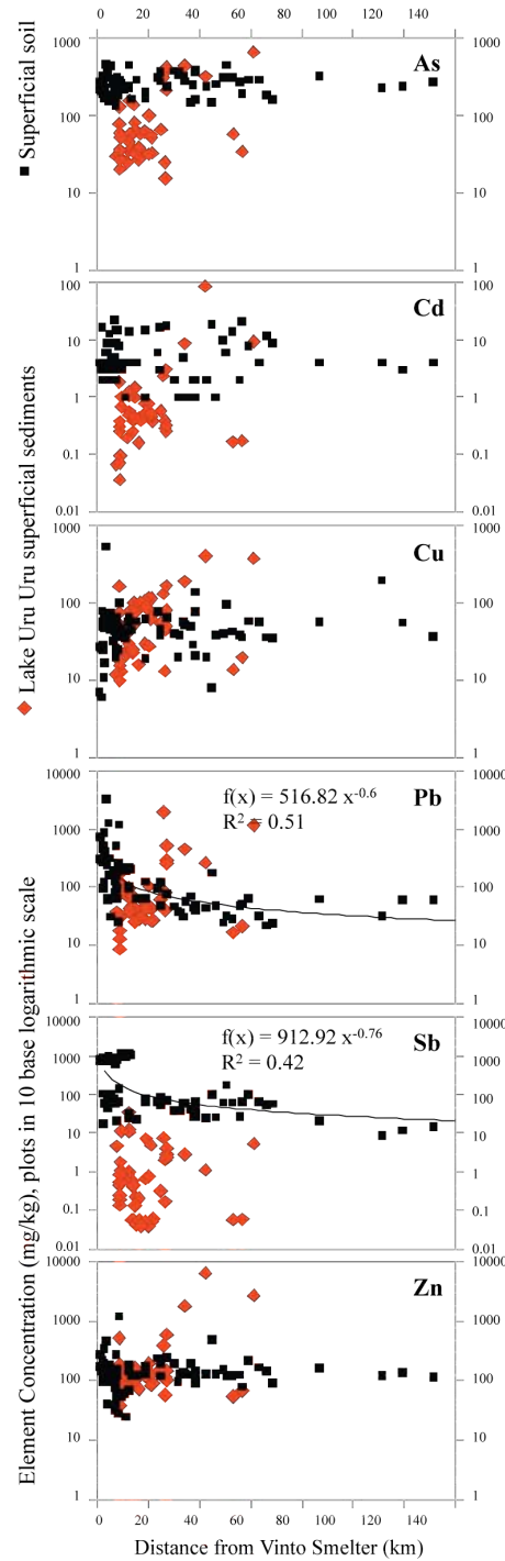
Figure 3.5.3: Arsenic, Cd, Cu, Pb, Sb and Zn distribution of soils and sediments respect to the distance from the Vinto Smelter. Regression models are for soils where fits exceeded 40% ( R^2 > 0.4 ).
