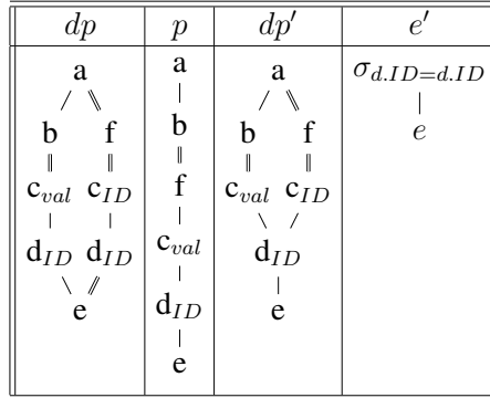
Figure 4.12: Node unification.
