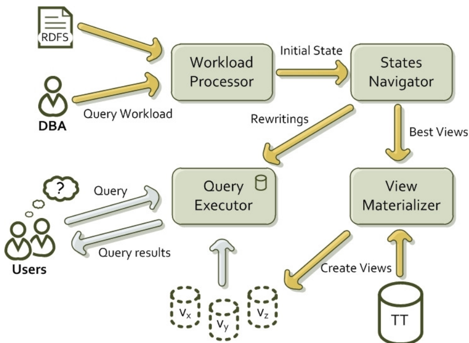
Figure 3.5: RDFViewS architecture.
